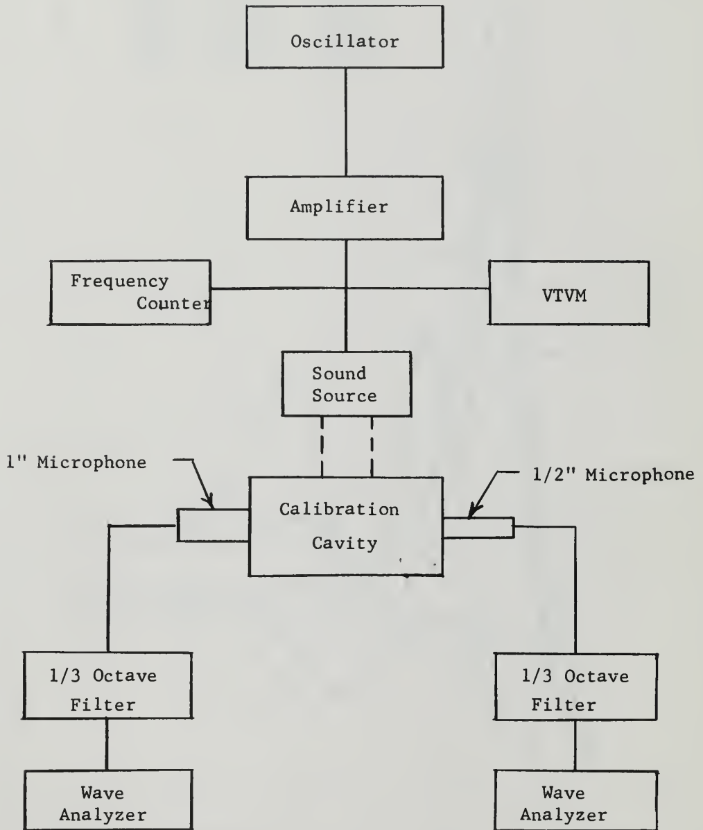
Fig. 3.4. Circuit Diagram for Comparison Calibration
