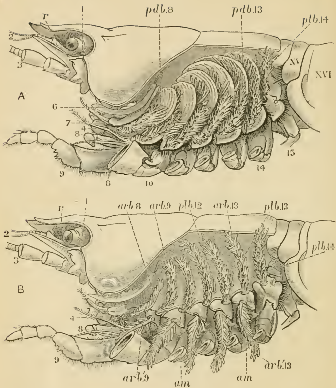
FIG. 4.— Astacus fluviatilis .—In A, the gills, exposed by the removal of the branchio-stegite, are seen in their natural position; in B, the podobranchiæ ( sec p. 75 ) are removed, and the anterior set of arthrobranchiæ turned downwards ( \times 2 ): 1, eye-stalk; 2, antennule; 3, antenna; 4, mandible; 6, scaphognathite; 7, first maxillipede, in B the epipodite, to which the line points, is partly removed; 8, second maxillipede; 9, third maxillipede; 10, forceps; 14, fourth ambulatory leg; 15, first abdominal appendage; xv., first, and xvi., second abdominal somite; arb. 8, arb. 9, arb. 13 , the posterior arthrobranchiæ of the second and third maxillipedes and of the third ambulatory leg; arb'. 9, arb'. 13 , the anterior arthrobranchiæ of the third maxillipede and of the third ambulatory leg; pbd. 8 , podobranchiæ of the second maxillipede; pbd. 13 , that of the third ambulatory leg; pbd. 12, plb. 13 , the two rudimentary pleurobranchiæ; plb. 14 , the functional pleurobranchia; r , rostrum.
