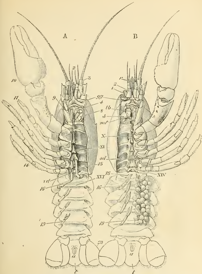
FIG. 3.— Astacus fluvialtilis .—Ventral or sternal views (nat. size). A, male; B, female:— a , vent; gg , opening of the green gland; lb , labrum; mt , metastoma or lower lip; od , opening of the oviduct; vd , that of the vas deferens. 1, eye-stalk; 2, antennule; 3, antenna; 4, mandible; 8, second maxillipede; 9, third or external maxillipede; 10, forceps; 11, first leg; 14, fourth leg; 15, 16, 19, 20, first, second, fifth, and sixth abdominal appendages; x, xi, xiv., sterna of the fourth, fifth, and eighth thoracic somite; xvi., sternum of the second abdominal somite. In the male, the 9th to the 14th and the 16th to the 19th appendages are removed on the animal's left side; in the female, the antenna (with the exception of its basal joint) and the 5th to the 14th appendages on the animal's right are removed; the eggs also are shown attached to the swimmerets of the left side of the body.
