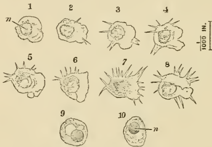
FIG. 14.— Astacus fluviatilis .—The corpuscles of the blood (highly magnified). 1-8 show the changes undergone by a single corpuscle during a quarter of an hour ; 9 and 10 are corpuscles killed by magenta, and having the nucleus deeply stained by the colouring matter. n , nucleus.
