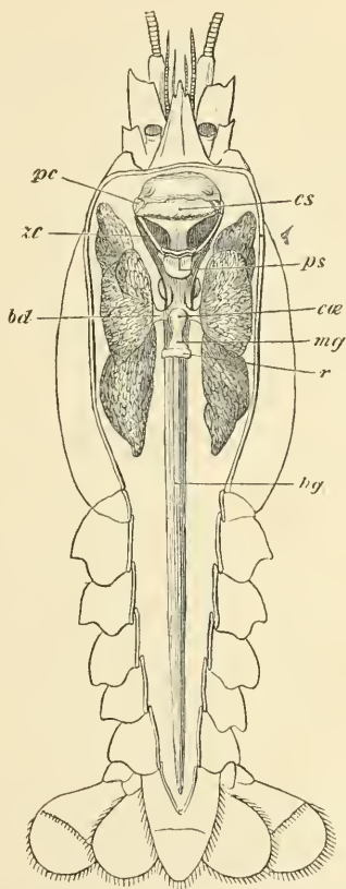
FIG. 13.— Astacus fluvialis . — The alimentary canal and livers seen from above (nat. size). bd , bile-duct ; cae , caecum ; cs , cardiac portion of stomach, the line pointing to the cardiac ossicle ; hg , hind-gut ; mg , mid-gut ; pc , ptero-cardiac ossicle ; ps , pyloric portion of stomach, the line pointing to the pyloric ossicle ; r , ridge separating mid-gut from hind-gut ; ze , zygo-cardiac ossicle.
