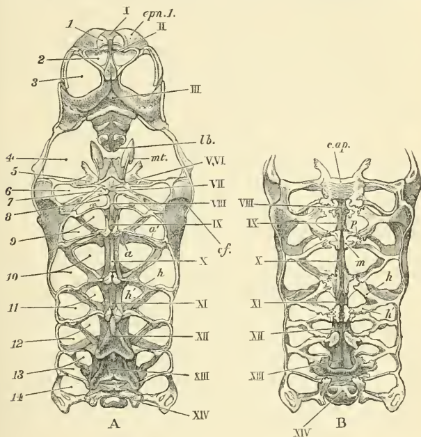
FIG. 39.— Astacus fluviatilis .—The cephalothoracic sternum and the endophragmal system ( \times 2 ). A , from beneath; B , from above. a , a' , arthropodites or partitions between the articular cavities for the limbs; c.ap. , cephalic apodeme; cf. , cervical fold; epn. I. , epimeron of the antennular somite; h , anterior, and h' , posterior horizontal process of endopleurite; lb. , labrum; m , mesophragm; mt. , meta-stoma; p , paraphragm; I—XIV , cephalothoracic sterna: 1—14 , articular cavities of the cephalothoracic appendages. (The anterior cephalic sterna are bent downwards in A so as to bring them into the same plane with the remaining cephalothoracic sterna; in B these sterna are not shown.)
