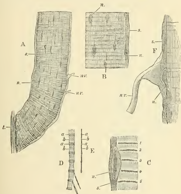
FIG. 19.— Astacus fluviatilis .—A, a single muscular fibre; transverse diameter \frac{1}{100} th of an inch; B, a portion of the same more highly magnified; C, a smaller portion still more highly magnified; D and E, the splitting up of a part of fibre into fibrillæ; F, the connexion of a nervous with a muscular fibre which has been treated with acetic acid. a , darker, and b , clearer portions of the fibrillæ; n , nucleus of sarcolemma; n.v. , nerve fibre; s , sarcolemma; t , tendon; 1—5, successive dark bands answering to the darker portions, a , of each fibrilla.
