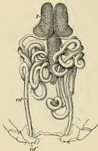
FIG. 31.— Astacus fluvialilis .—The male reproductive organs ( \times 2 ); t , testis; vd , vas deferens; vd' , aperture of vas deferens.
