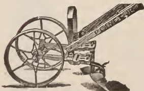
No. 13 Double Wheel Hoe.
