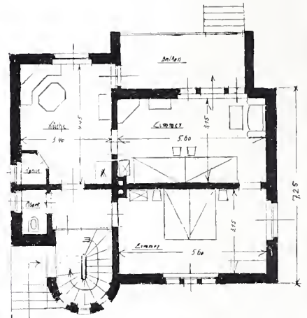
Erdgeschoss.
