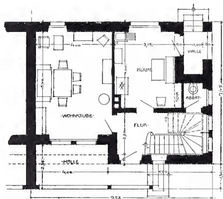
Erdgeschoss.
