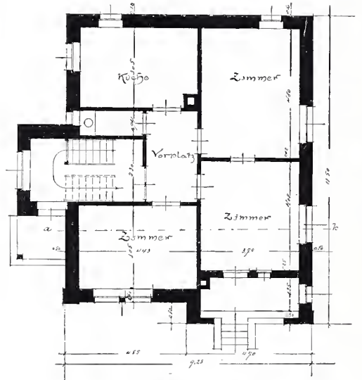
Erdgeschoss.
