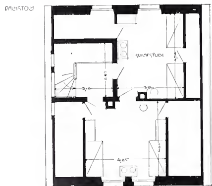
Dachstock.
