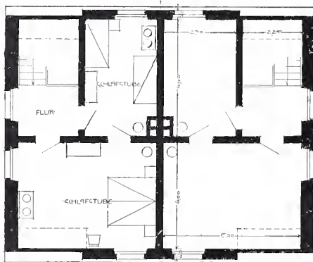
Dachstock.
