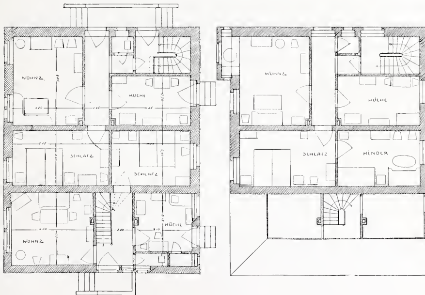
Erdgeschoss.
