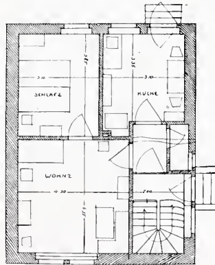
Erdgeschoss.
