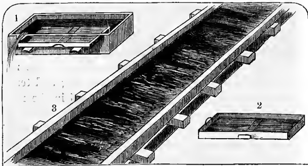
Fig. 1. Terra-cotta Tray, to fit crosswise in race-way. Fig. 2. Grille of glass tubes, made to fit in the tray. Fig. 3. Race-way, as wide inside as the length of the tray.
