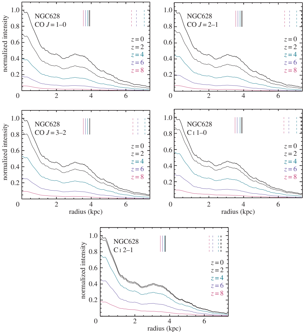
Figure 7. Radial distributions of the simulated CO J = 1-0 , CO J = 2-1 , CO J = 3-2 , C I 1-0 and C I 2-1 emission of NGC 628 at redshift 0, 2, 4, 6 and 8, respectively. The colours show the redshifts. Similar to figure 4, we measure the average flux in each concentric elliptical rings, and normalize it with the flux in the central position at z = 0 . The vertical solid lines show the half-light radii ( R_{50} ), and the vertical dashed lines show the 90% light radii ( R_{90} ).
