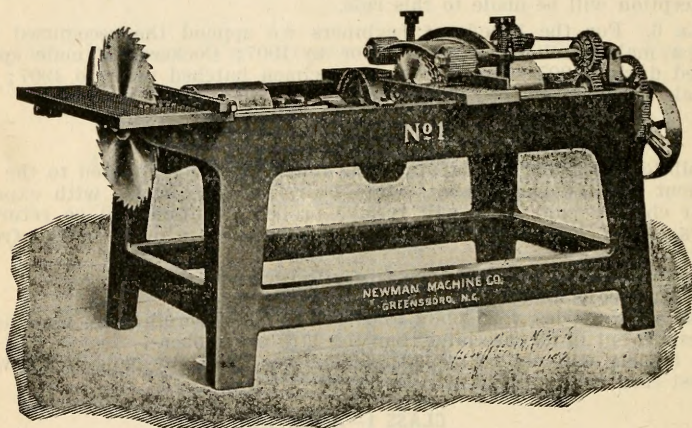
COMBINED LATH MILL AND BOLTER.
