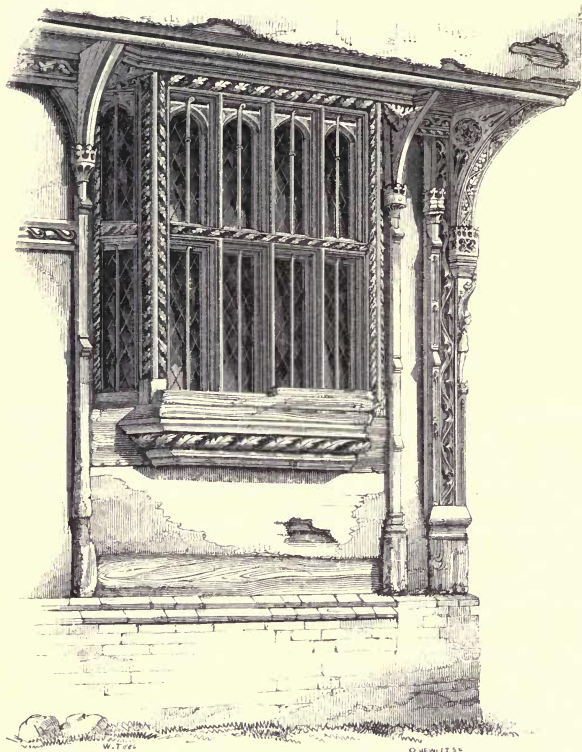
WINDOW AND CORNER-POST,
