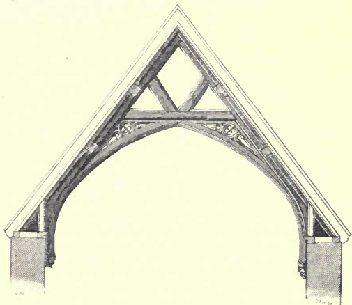
Roof of the Deanery, or Prior's Hall.
