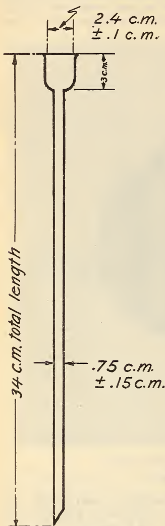
FIG. 13.—Condenser tube
