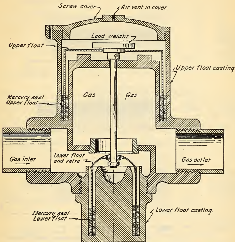
FIG. 20.—Sectional view of one form of gas pressure regulator
