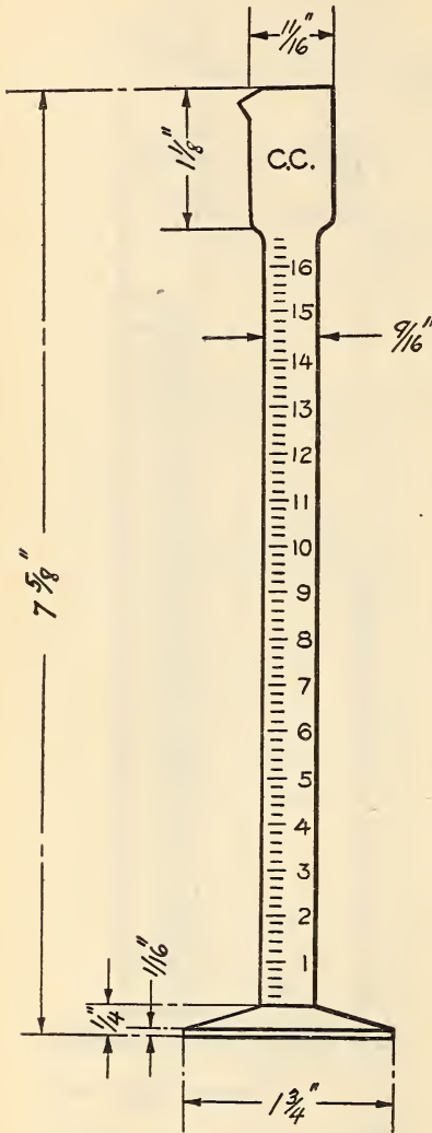
FIG. 6.—Special moisture-testing graduate, 16 cubic centimeters capacity, for use in testing moisture content of oats and other lightweight material
