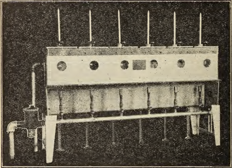
FIG. 1.—Brown-Duvel moisture tester equipped with gas burners and gas-pressure regulator
