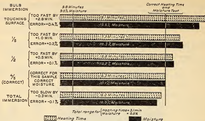
FIG. 22.—Effect of variations in the depth of immersion of the thermometer bulb in the oil on the moisture-test result
