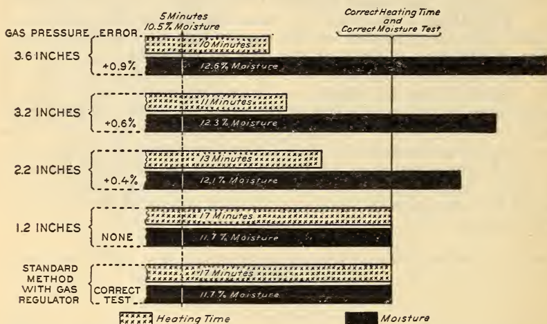
Fig. 19.—Effect of gas pressure on the heating time and the moisture test result
