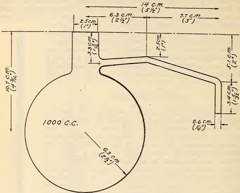
FIG. 8.—Standard single-walled distillation flask, 1,000 cubic centimeters capacity
