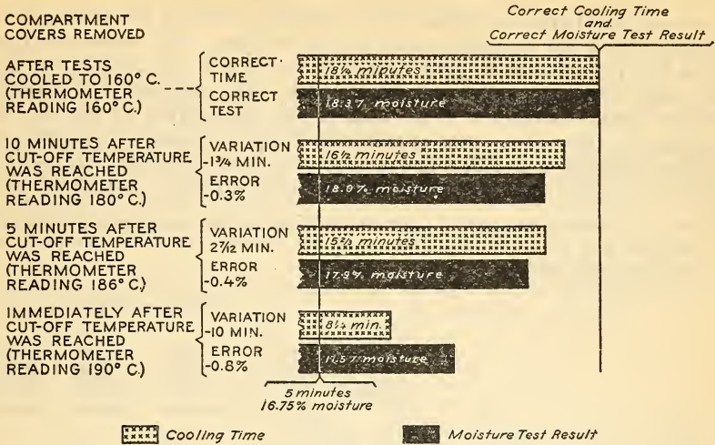
FIG. 23.—Effect of cooling time on the moisture-test result
