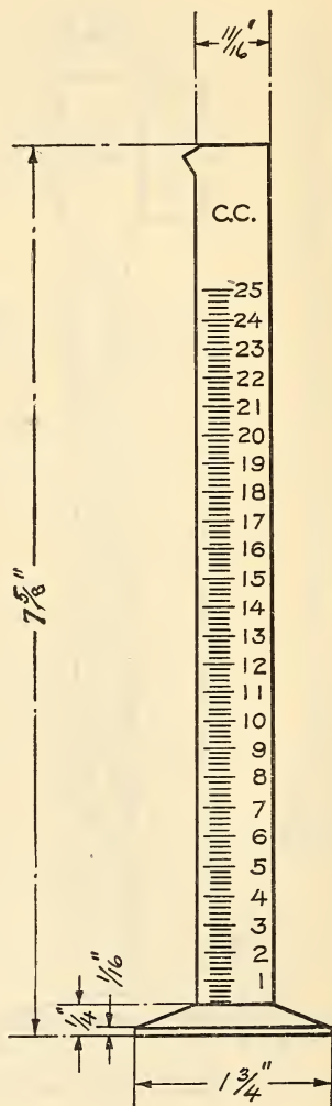
FIG. 5.—Standard moisture-testing graduate, 25 cubic centimeters capacity
