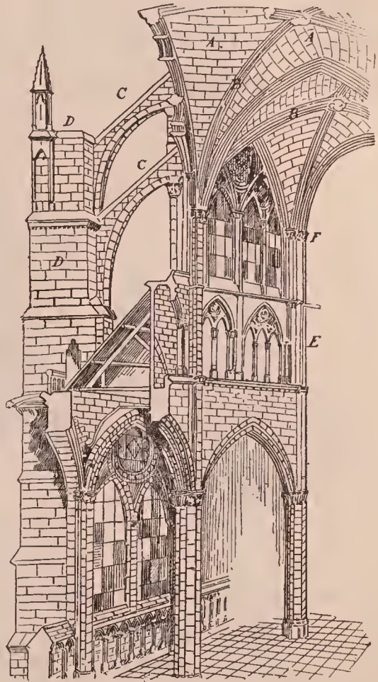
CROSS SECTION OF AMIENS CATHEDRAL
