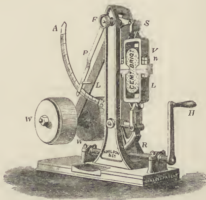
Fig. 91. Michele's Cement Testing Machine.
