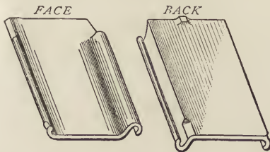
Sections showing the wing lock
