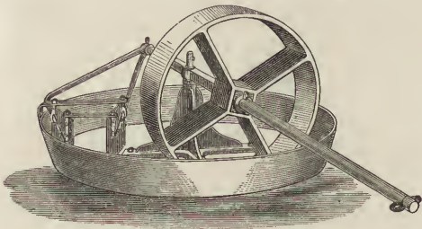
Fig. 105. Horse Mortar-Mill.
