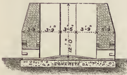
Fig. 10. Cross Section.
