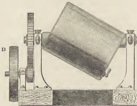
Fig. 107. Inclined Cylinder Concrete-Mixer.
