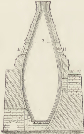
Fig. 99. Section.
