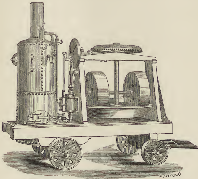
Fig. 104. Portable Mortar-Mill.
