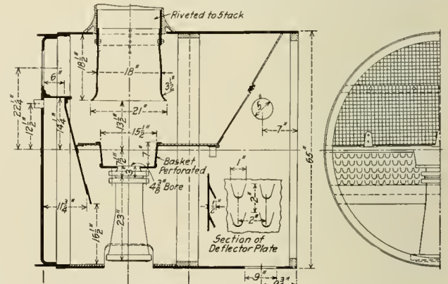
Fig. 5—Front End for a Consolidation Locomotive In 1893
