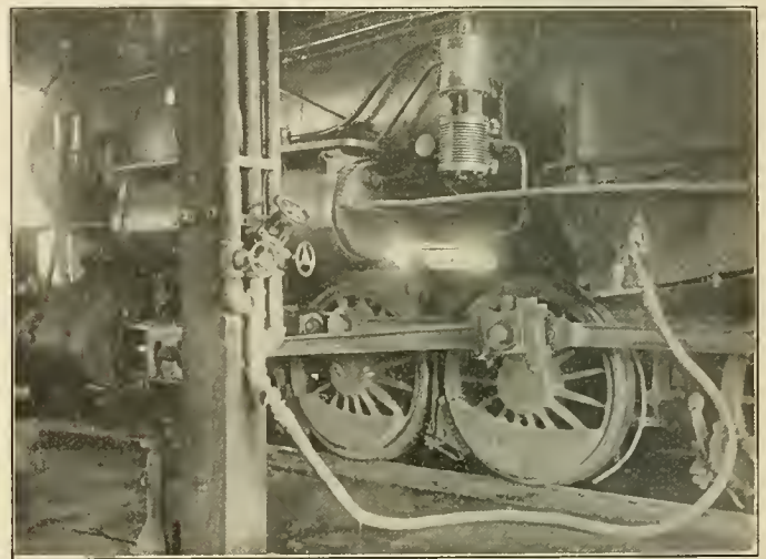
Arrangement of Drop Lines Between Roundhouse Stalls
