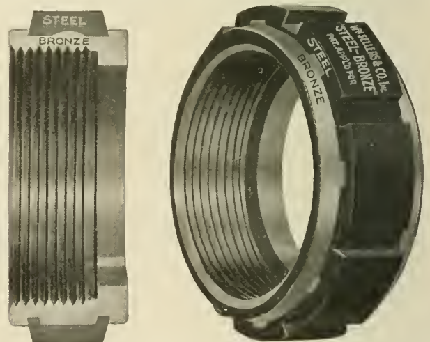
Sellers Coupling Nut for Injector Connections
