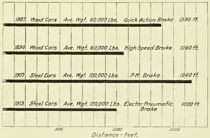
Fig. 3—Comparison of Emergency Stops
