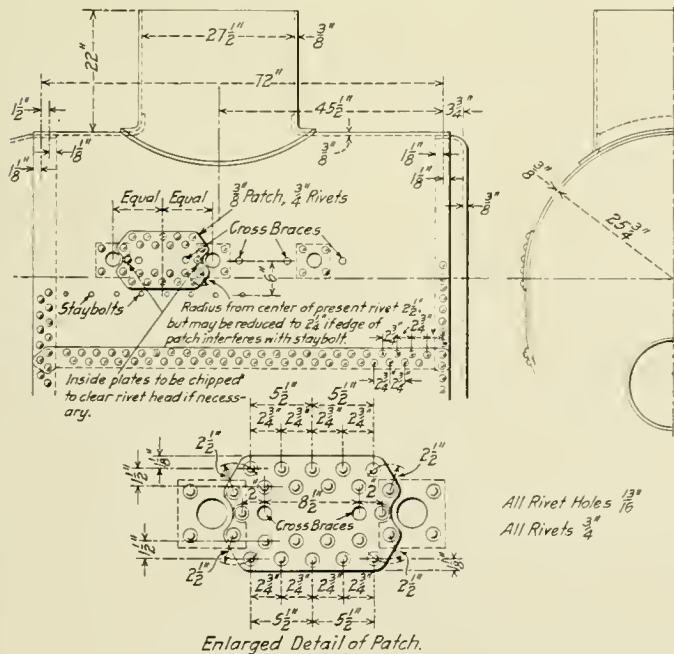
Fig. 4—Difficult Patch Placed Between Two Washout Holes
