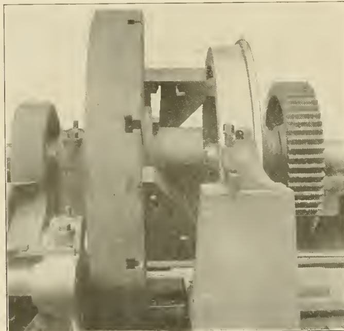
Socket Plate and Driver Arms for Centering and Driving Mounted Wheels with Outside Journals
