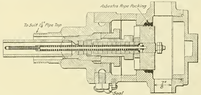
Section Through the Saturated Steam Fixture
