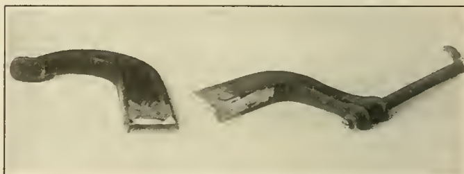
Clamp Prepared for Welding
