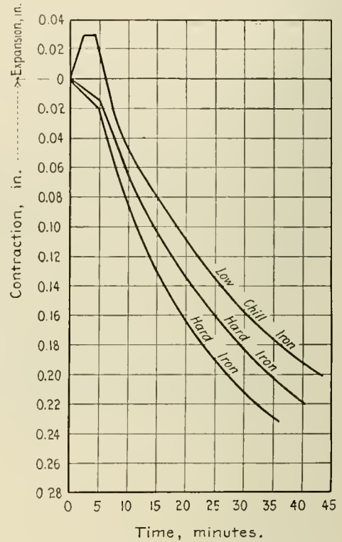
Fig. 6—Shrinkage Curves for 1 In. Square Bar, 12 In. Long, Wheel Iron, Cast in Sand
