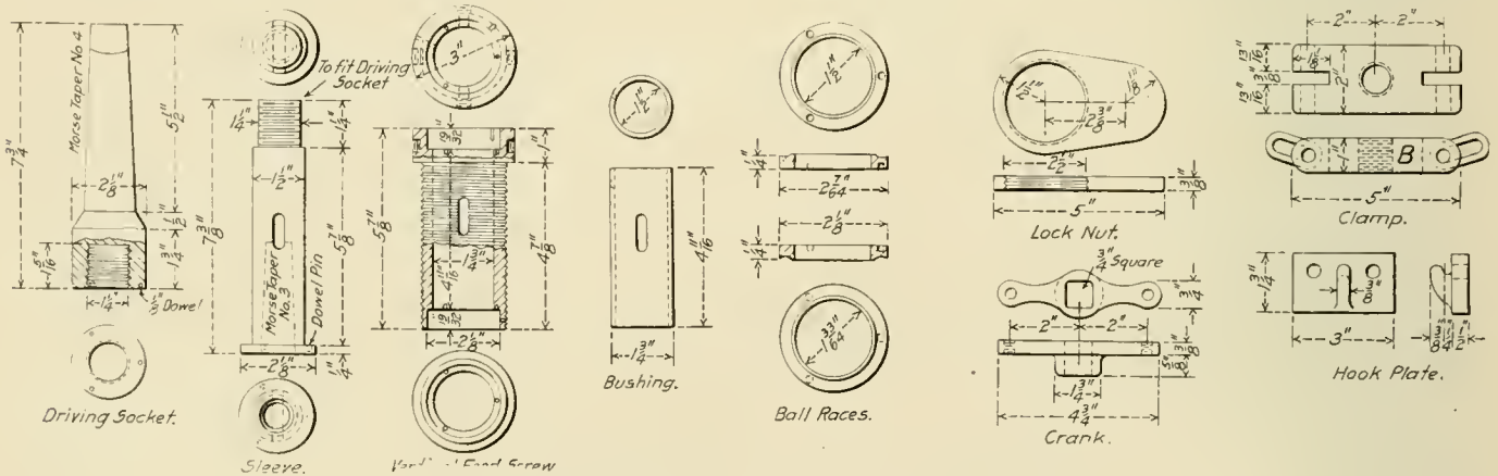
Fig. 5—Details of Machine for Milling Eccentric Keyways
