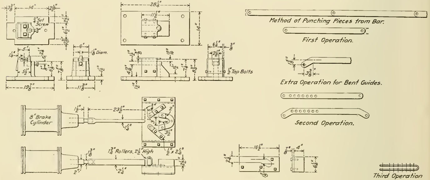
Fig. 2—Apparatus Used in Making Slack Adjusters
