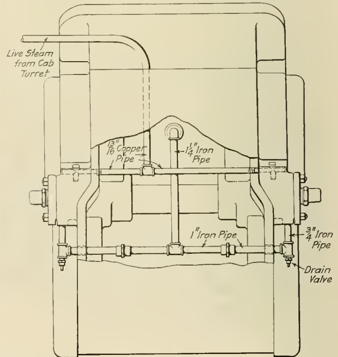
Steam Connections to By-pass Drifting Valves
