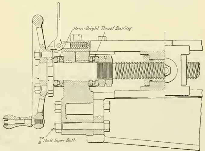
Section of Screw Reverse Gear
