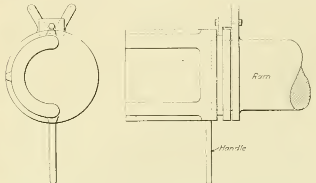
Fig. 15—Attachment for Mounting Press Ram
