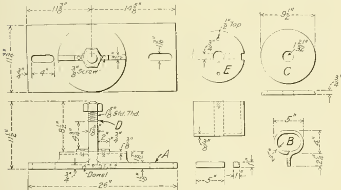
Fig. 1—Mandrel for Turning Eccentrics on a Boring Mill
