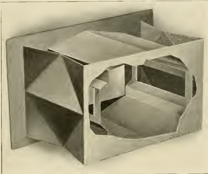
Fig. 1—Type 4 Mudge-Peerless Ventilator Showing Interior Arrangement
