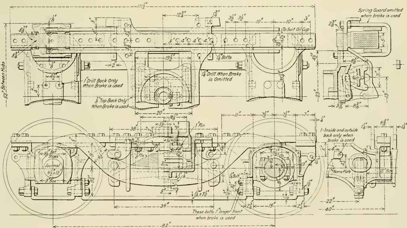
Arrangement of the Constant Resistance Engine Truck
