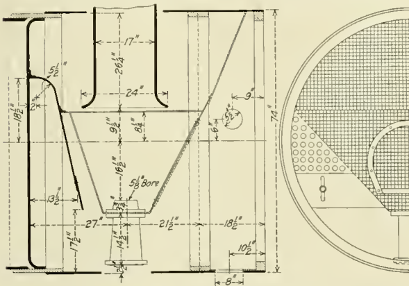
Fig. 6—A Front End Design of 1903
