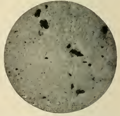
Fig. 5—Porous Steel. Section Near the Fracture; 50 Diameters
