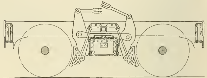
Brake Rigging with One Shoe to Each Wheel
