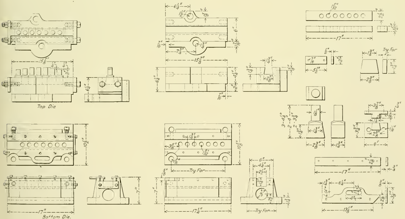
Fig. 1—Gang Punch for Punching Slack Adjuster Rods
