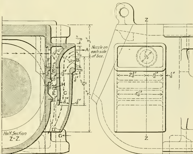
Journal Box Arranged for Induced Ventilation
