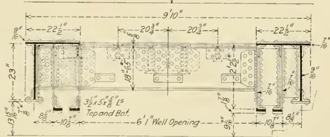
Sections of Lehigh Valley Well Car
