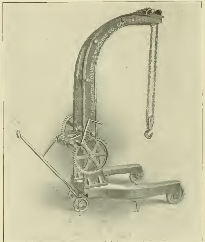
Portable Crane and Hoist Equipped with Back Gear
