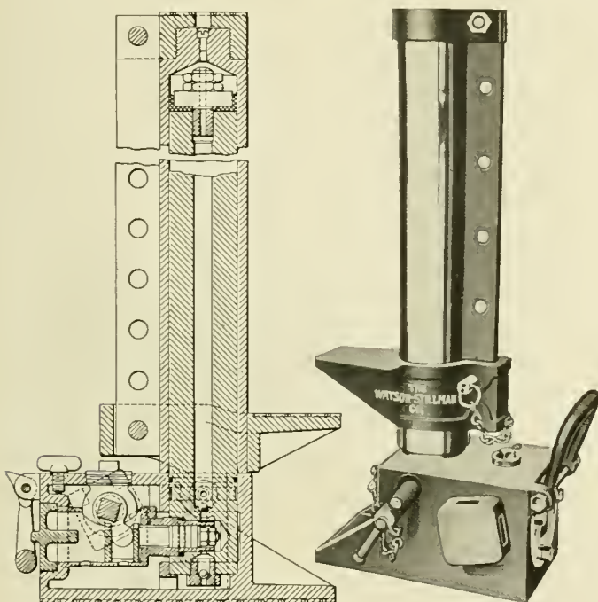
Exterior and Sectional Views of Emergency Jack
