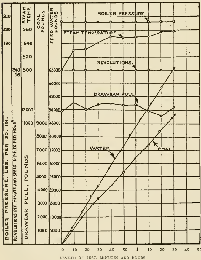
Fig. 12—Graphical Log of Test
