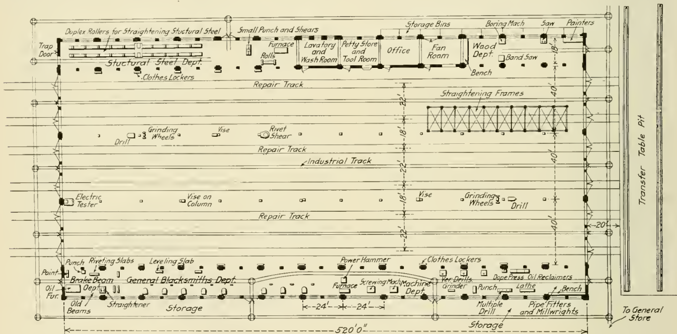
Plan of Proposed Steel Freight Car Repair Shop
