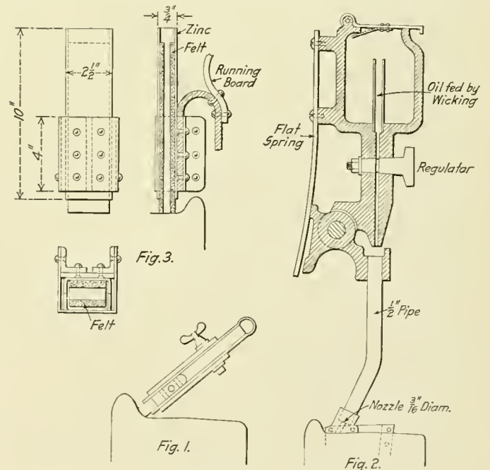
Flange Oilers Used In Europe
