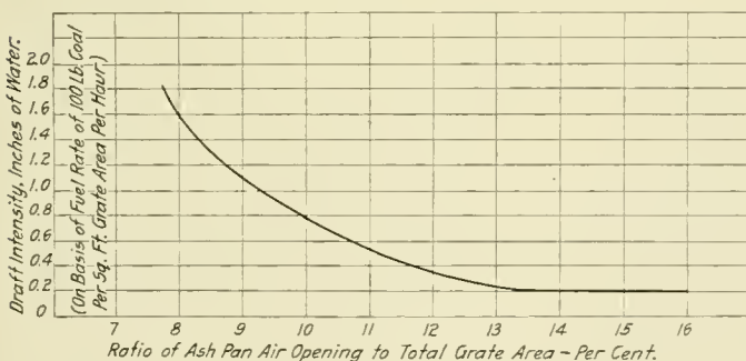
Diagram of Ash Pan Coefficients
