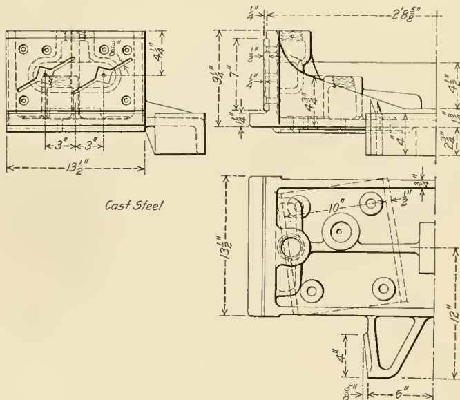
Engine Truck Bolster Gulde, Canadian Pacific Mikado
