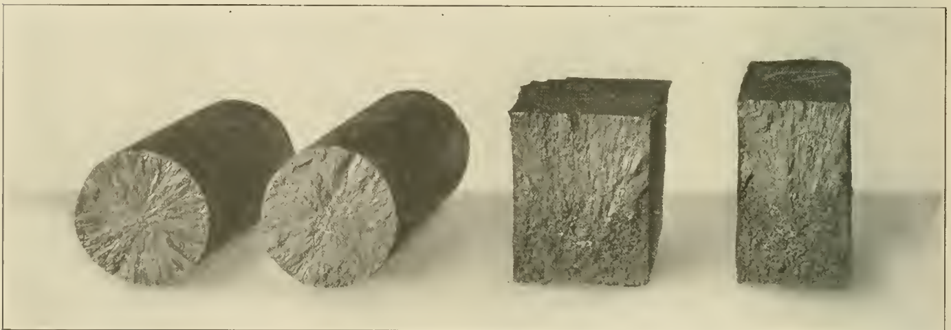
Fig. 5—(a) Ends of Two Chilled Rolls; (b) End of Chill Block; (c) End of Partly Chilled Rectangular Block
