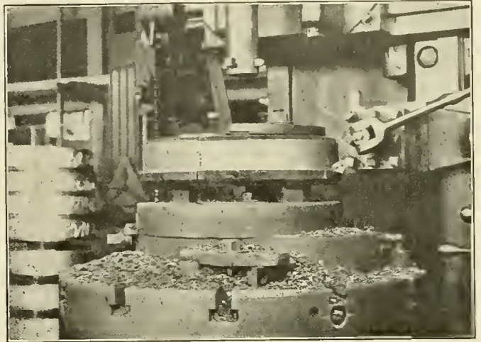
Eccentric Chuck Attached to a Boring Mill
