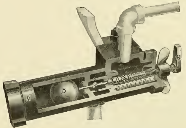
Control Valve of Automatic Flange Lubricator
