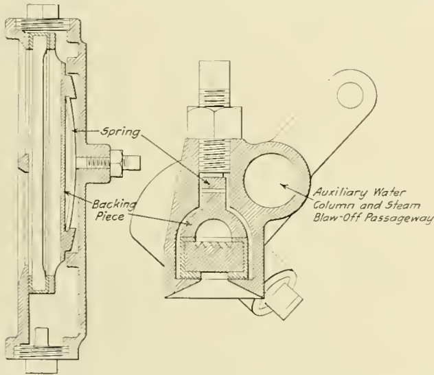
Sections Through Registering Column of "Pressurlokd" Water Glass
