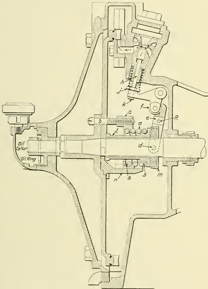
Fig. 11—Turbine End of Pyle-National Generator
