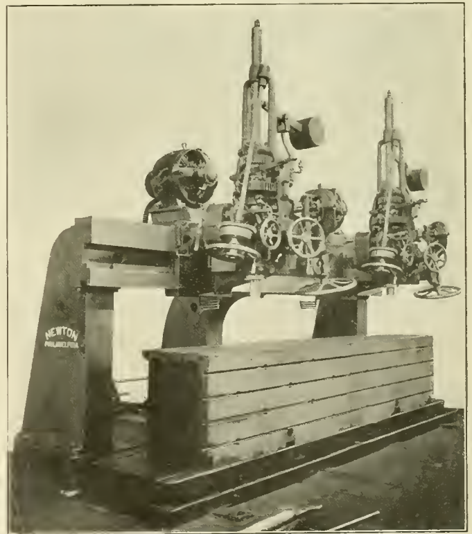
Frame Drill with Top Work Table in Forward Position
