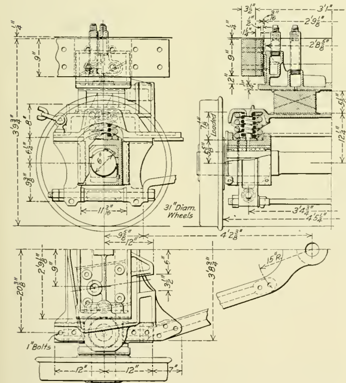
Arrangement of the Engine Truck of the Canadian Pacific Mikado
