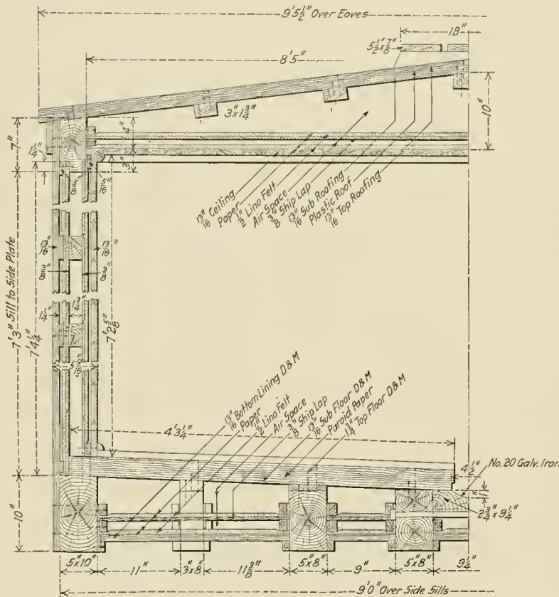
Insulation Details of the Milwaukee Refrigerator Transit & Car Company Dairy Car
