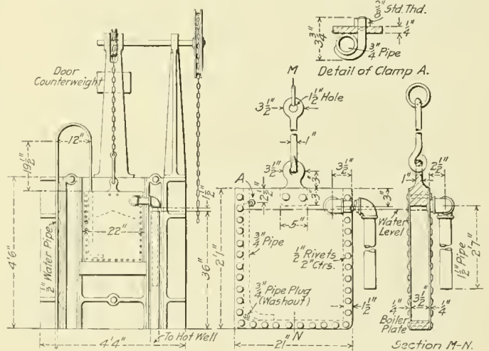
Fig. 3—Water Jacket Door for Oil Furnace
