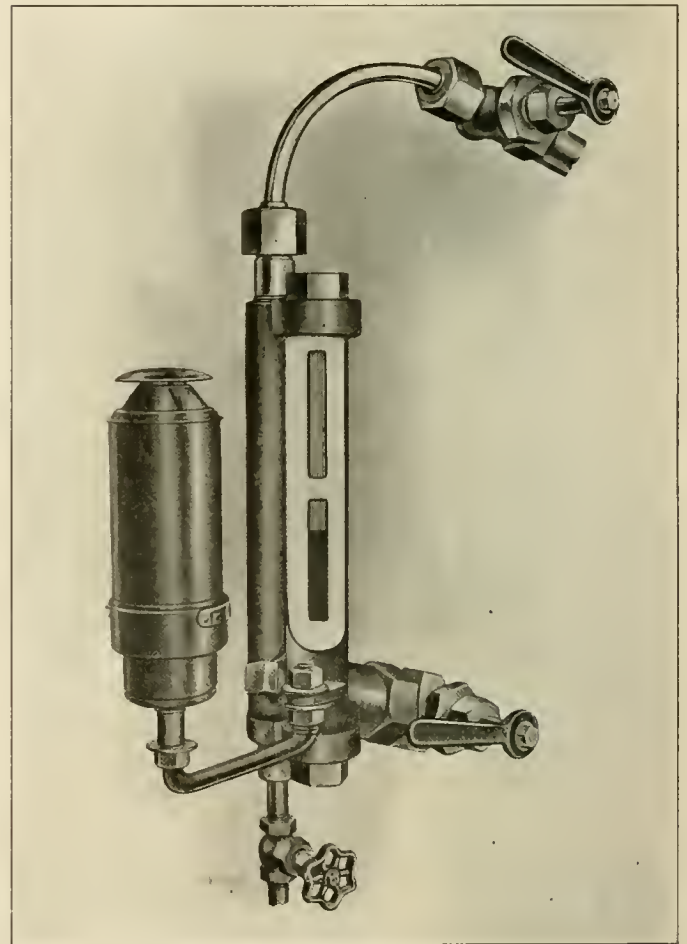
Reflex Water Gage with Metal Encased Glass
