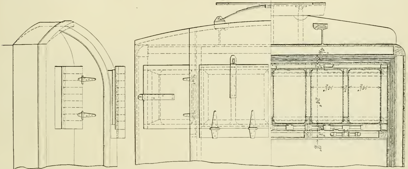
Half-Sectional Plan and Elevation Showing Brine Tanks and Hatches
