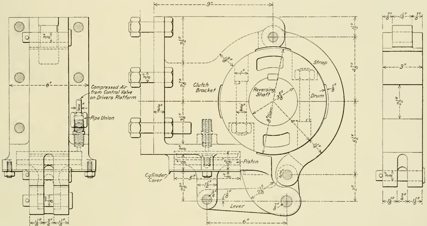
Clutch for Reversing Shaft
