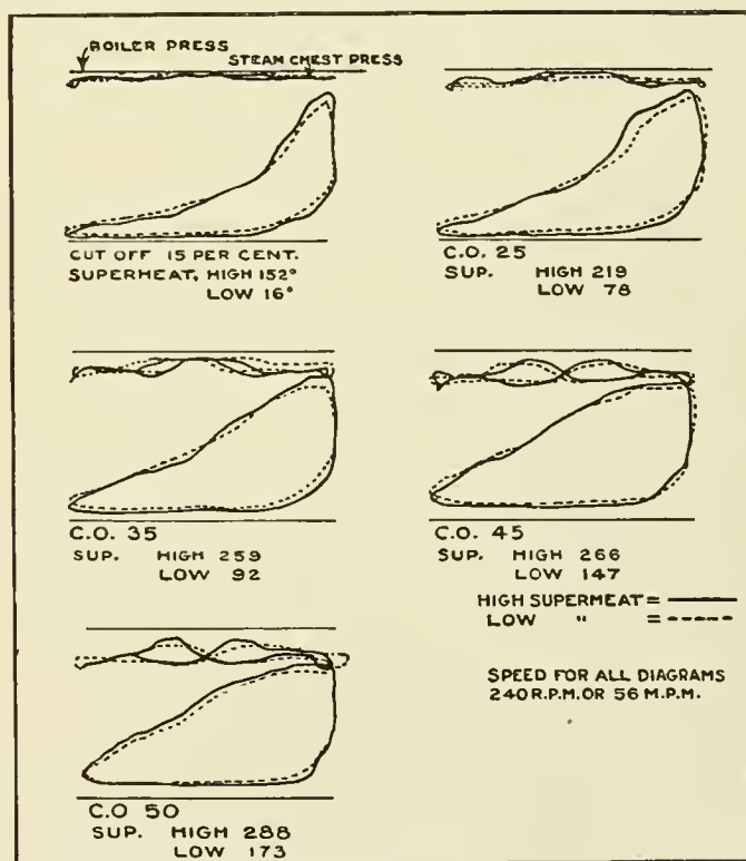
Fig. 11—Indicator Diagrams Showing High and Low Superheat
