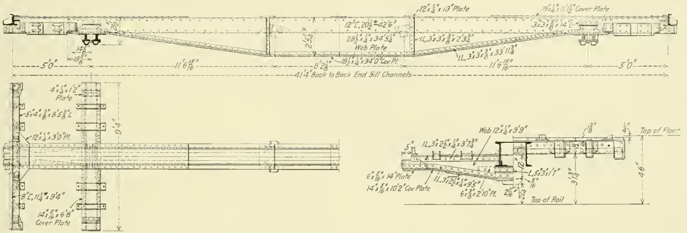
Steel Underframe for the Northern Pacific Stock Car
