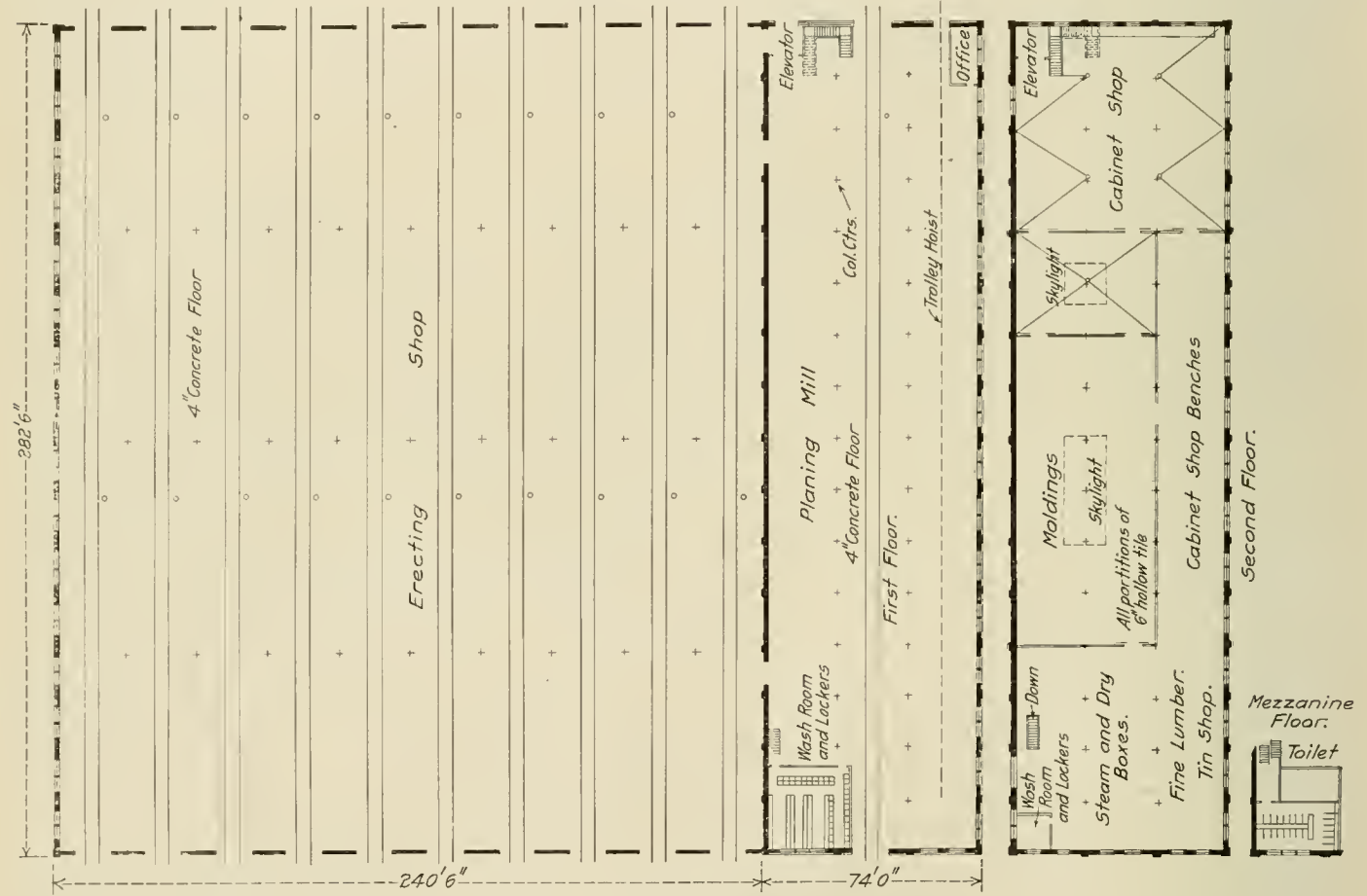
Floor Plan of the Passenger Car Shop
