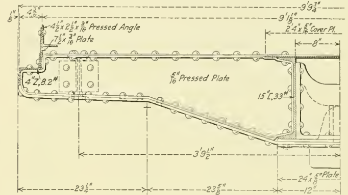
Steel Pressings Are Used in the Construction of the Double Body Bolster
