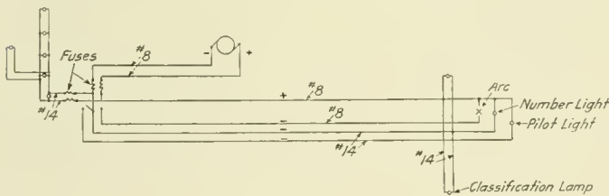
Western Pacific Headlight Wiring
