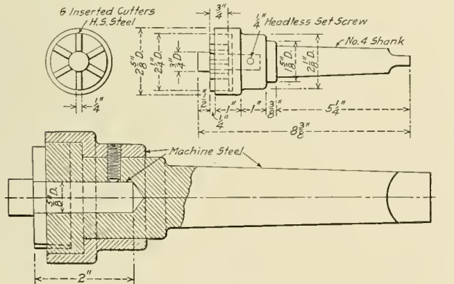
Fig. 8—Rotary Scarfing Tool
