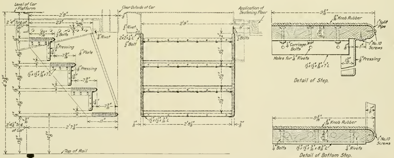
Standard Four-tread Coach Step Used on the Grand Trunk
