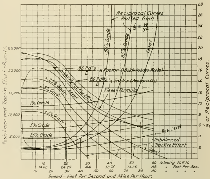
Fig. 1—Characteristic Curves
