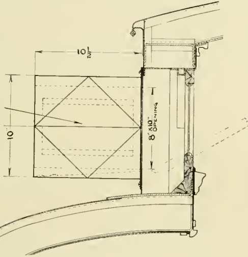
Fig. 5—Application of Ventilator to Monitor or Clerestory Roof
