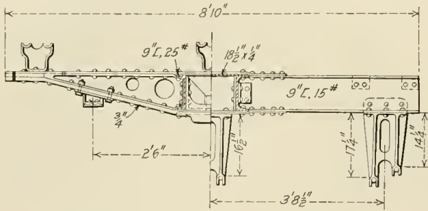
Cross Sections of the Gondola Car Underframe
