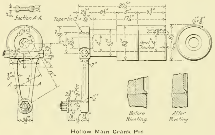
Hollow Main Crank Pin
