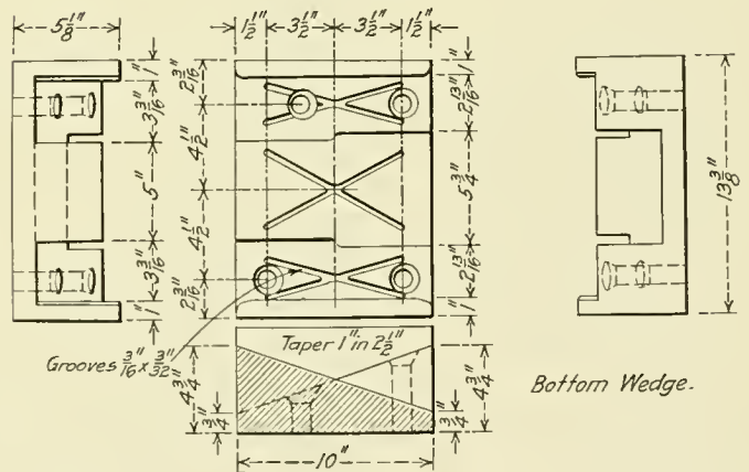
Engine Truck Wedges Used on the Canadian Pacific Mikado
