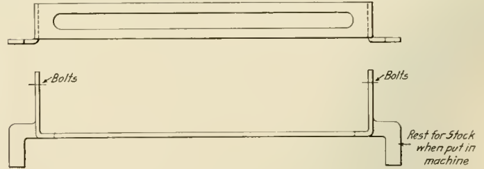
Fig. 5—Extension Used on Stationary Die When Forging Saddle Straps
