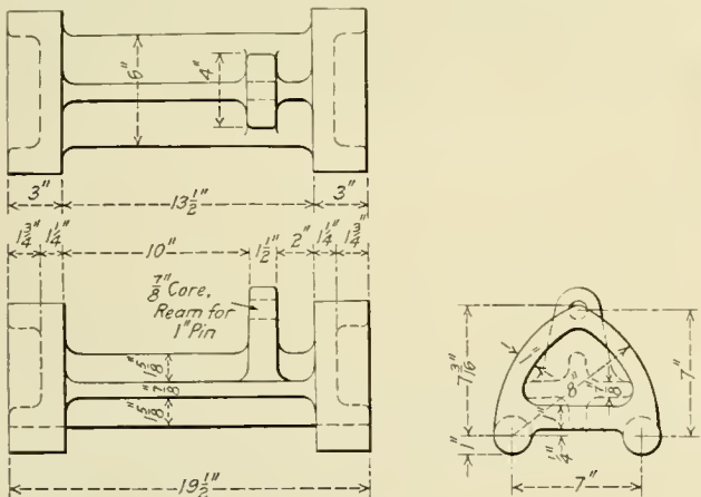
Rocker Used in the Engine Truck
