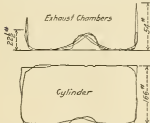
Fig. 3—Card with Solid Internal Admission Piston Valve
