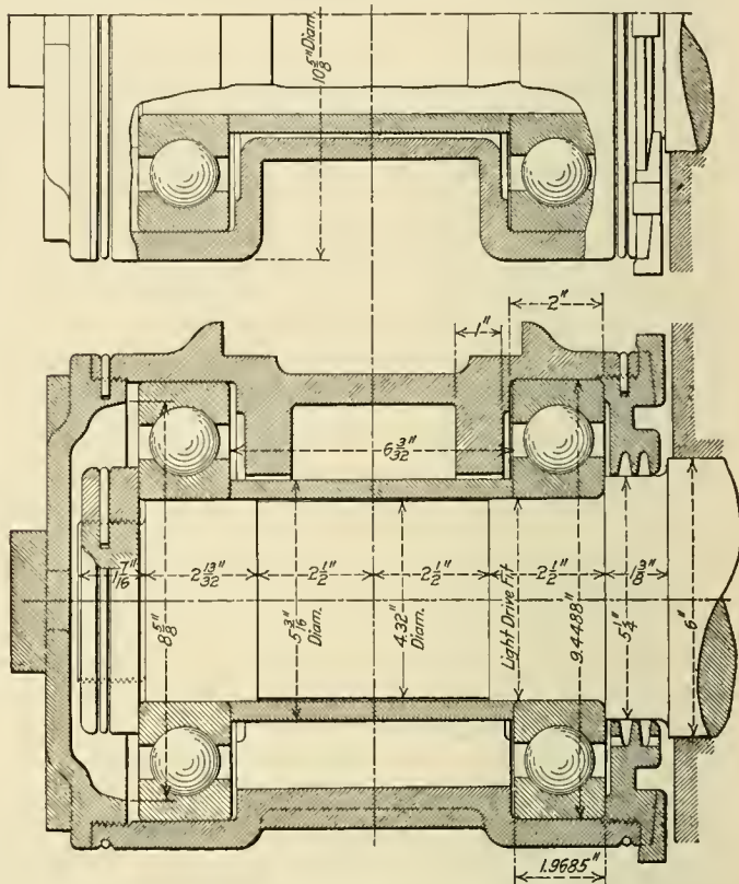
Typical Arrangement of Ball Bearing Car Journal
