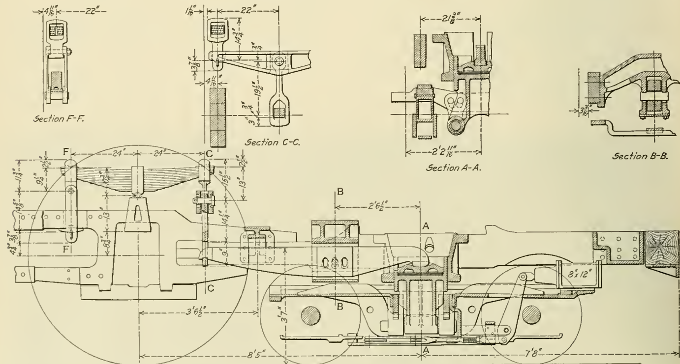
Equalization Between Front Truck and First Pair of Drivers
