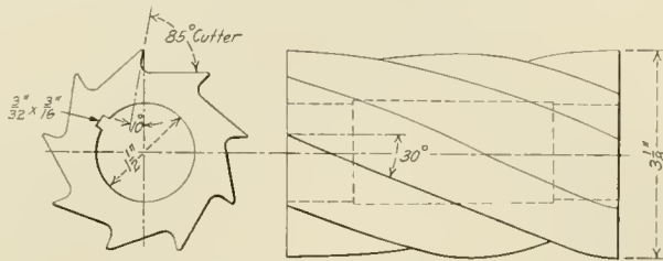
High Speed Steel. 9 Teeth.
