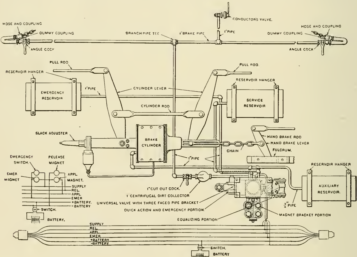
Diagram of the Complete Westinghouse Electro-Pneumatic Brake (U C Equipment)
