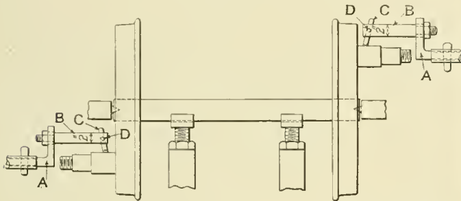
Attachment for Turning Crank Pins in a Quartering Machine
