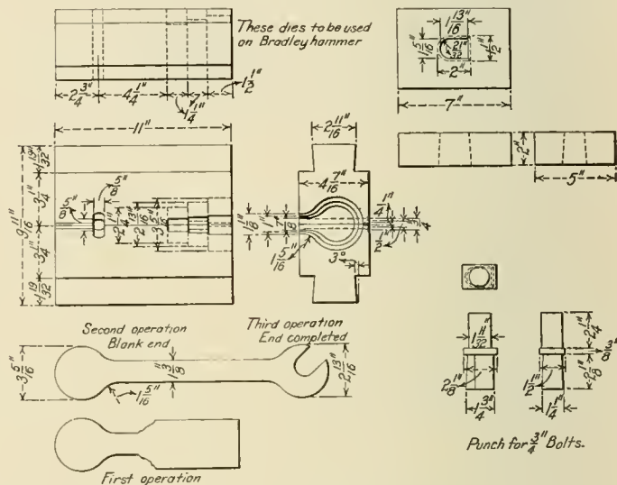
Fig. 12—Dies for Forming Wrenches from Scrap Spring Steel
