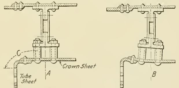
Fig. 2—Effect of Rigid T Bar Construction
