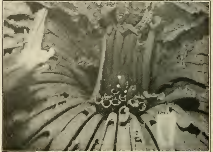
Fig. 5—Condition of Tubes Just Back of Injector Checks
