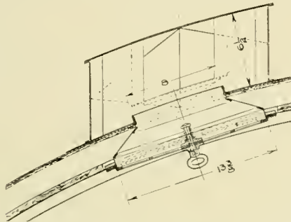
Fig. 6—Application of Ventilator to Arch Roof
