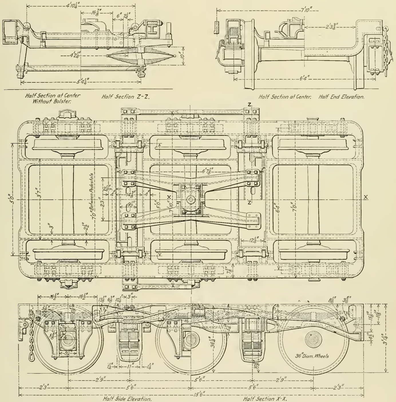
General Arrangement of New York Central Six-Wheel Steel Truck
