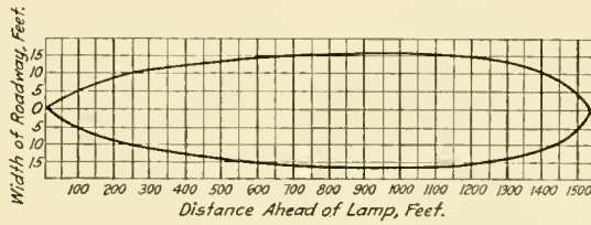
Fig. 2-Isolux Curve.
