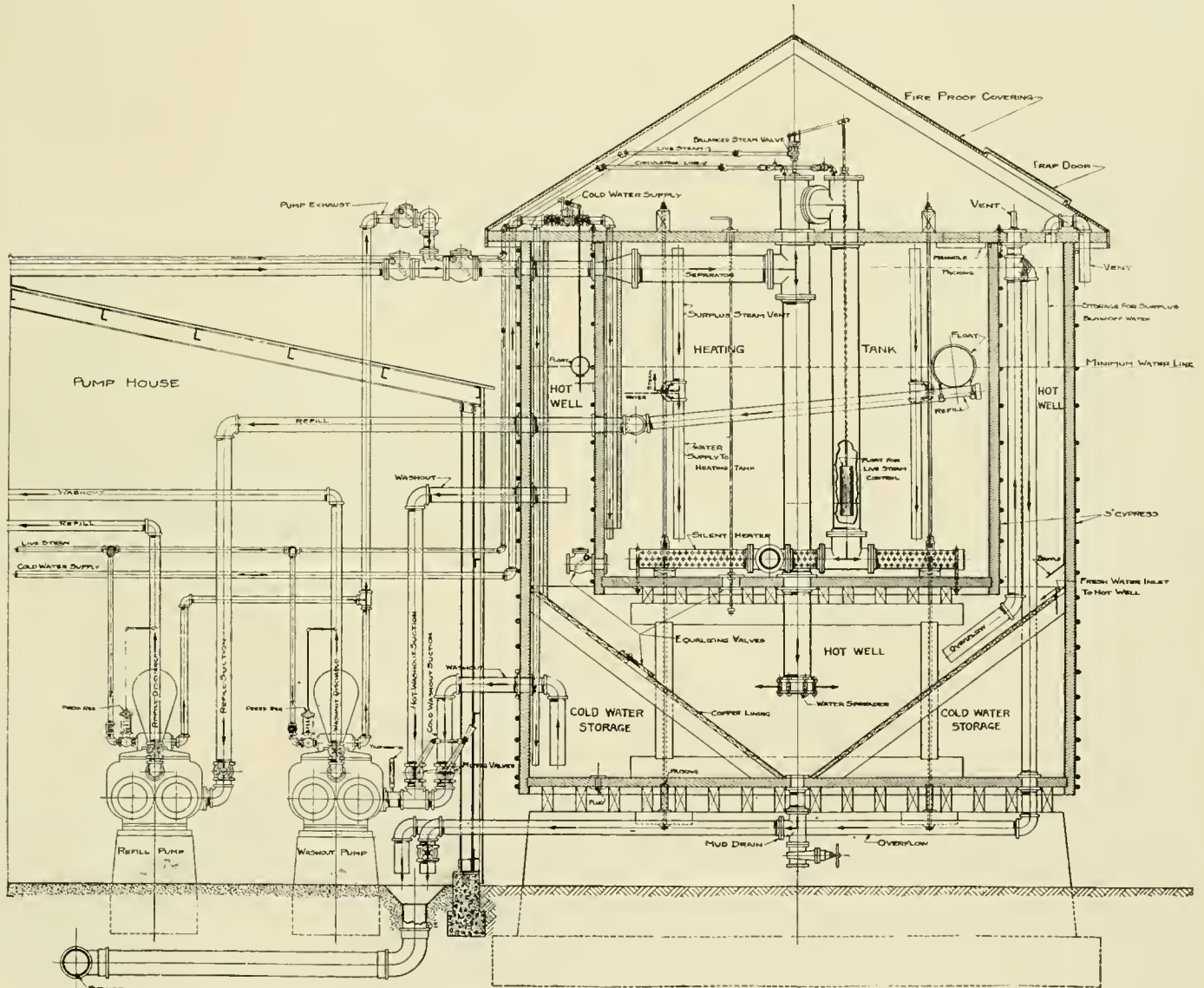
Hot Water Boiler Washing and Filling Plant
