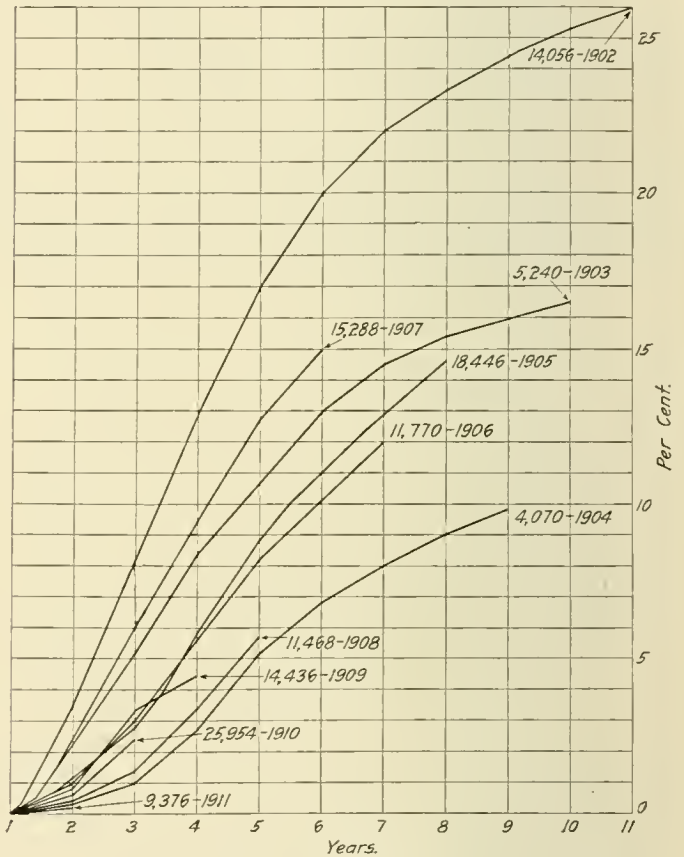
Fig. 4—Failures Caused by Manufacturer's Defects on Wheels for 80,000 lb. Capacity Cars
