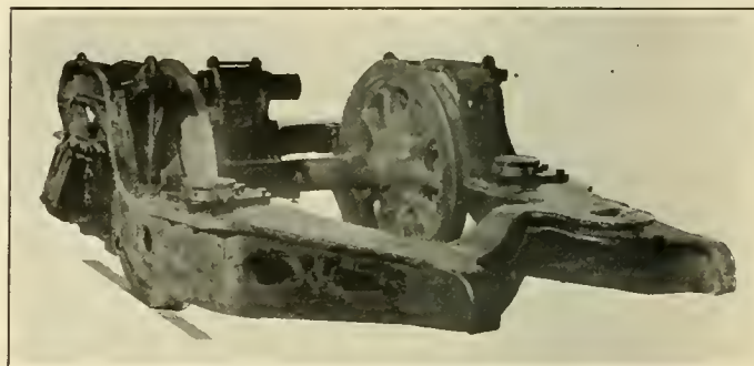
Trailer Truck for E6s Pennsylvania Locomotive
