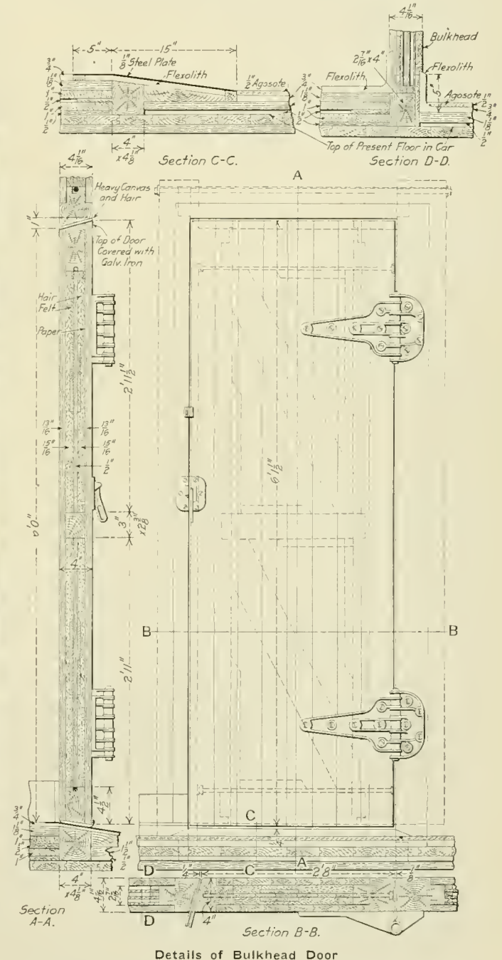
Details of Bulkhead Door
