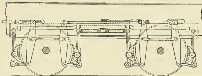
Brake Rigging Referred to as No. 3 Clasp Brake
