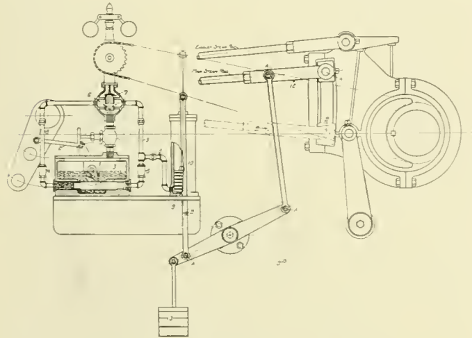
Speed Governor and Speed Regulator for Cross Compound Air Compressor
