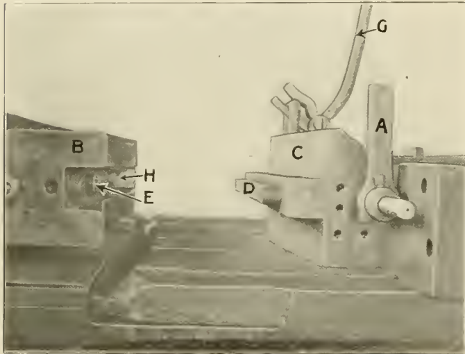
Fig. 4—Stripper D in Release Position
