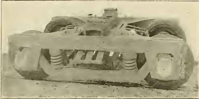
Four-Wheel All-Steel Passenger Truck
