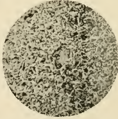
Fig. 3—Inside Oxidized Portion, Midway Between Center and Circumference, Polished and Etched with Iodine; 50 Diameters
