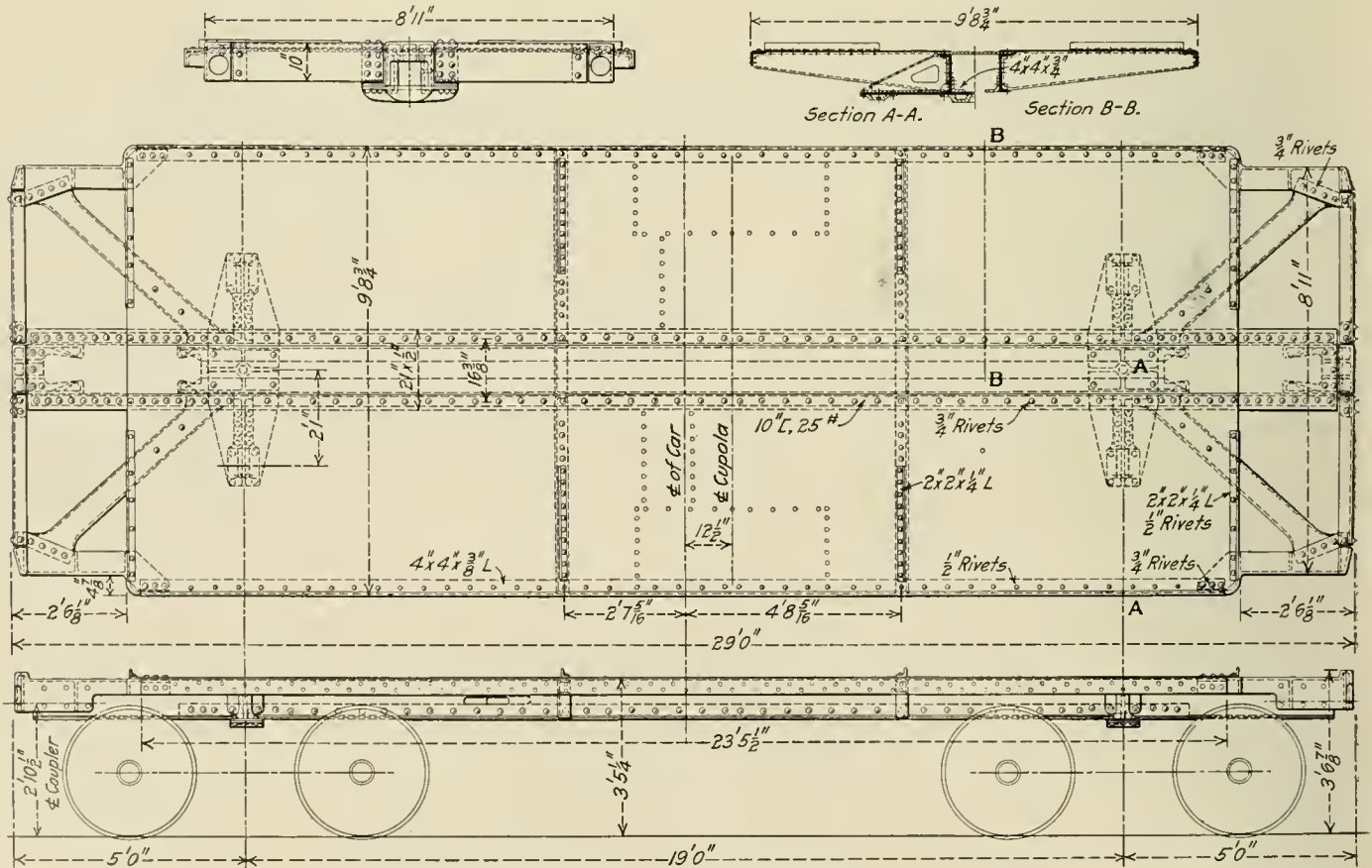
Underframe Construction Used on the Pennsylvania Steel Caboose
