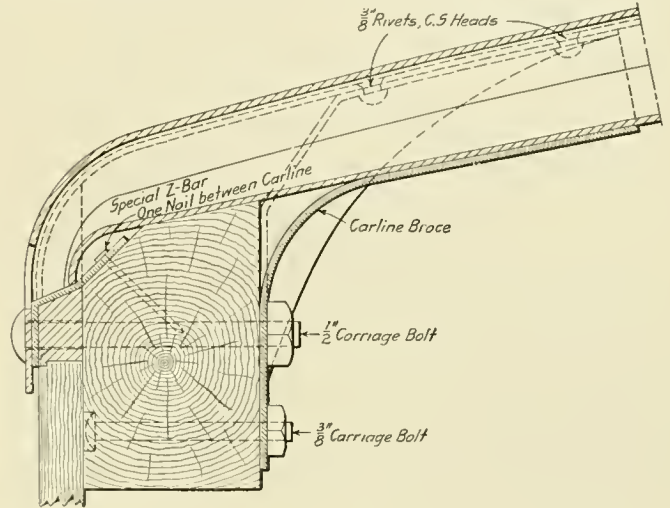
Section Through Carline at the Side Plate on a Wooden Frame Car
