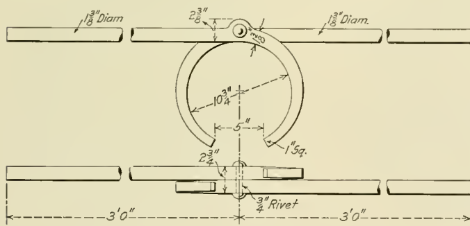
Handy Tongs for Carrying Large Sizes of Pipe
