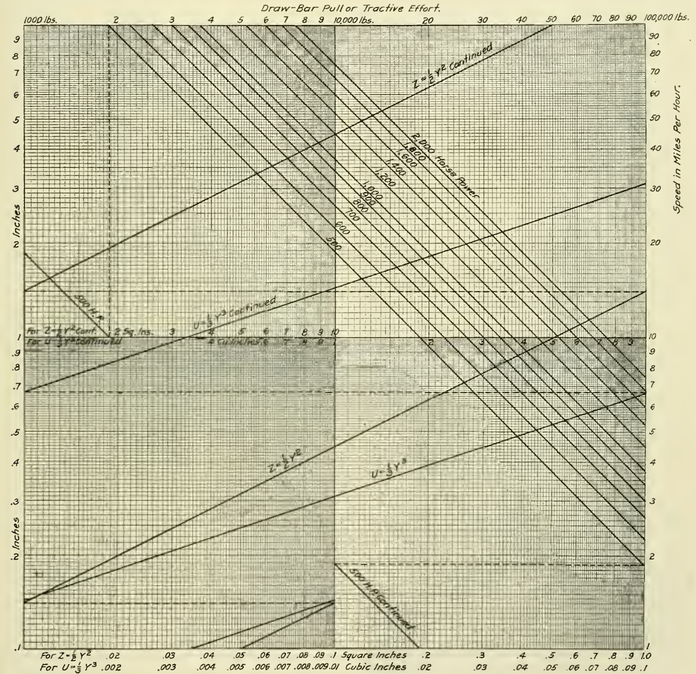
Chart Illustrating the Uses of Logarithmic Paper
