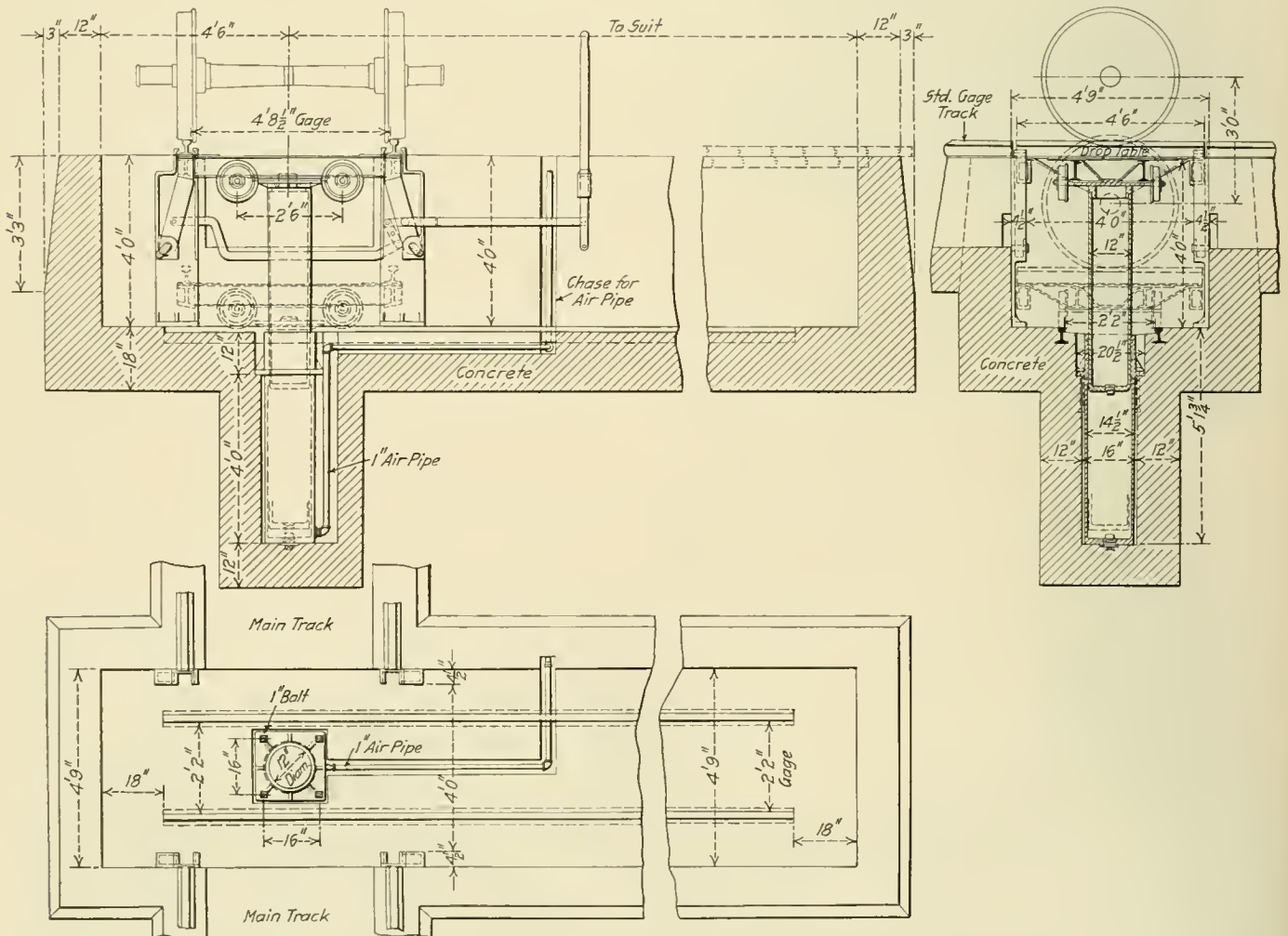
Improved Drop Pit for Removing Passenger Car Wheels
