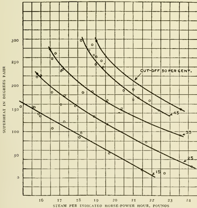
Fig. 5—Cut-off and Steam per Indicated Horse Power
