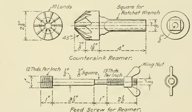
Fig. 9—Tools for Applying Patch Bolts
