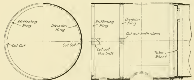
Method of Cutting Rings to Remove a Front Tube Sheet
