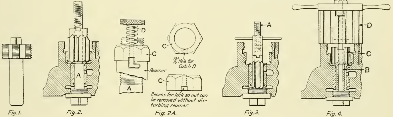
Method of Repairing Slide Valve Feed Valves
