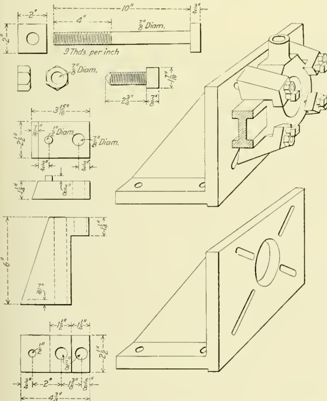
Fig. 7—Clamp for Side Rods
