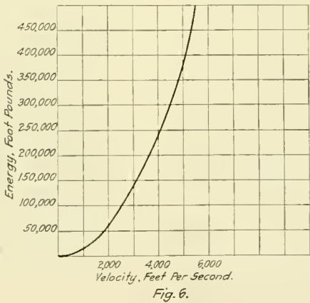
Diagrams for Use in Electric Headlight Turbine Calculations
