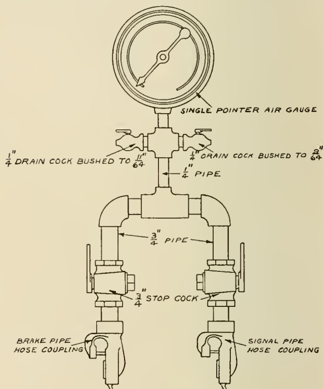
Testing Device for Locomotive Brakes
