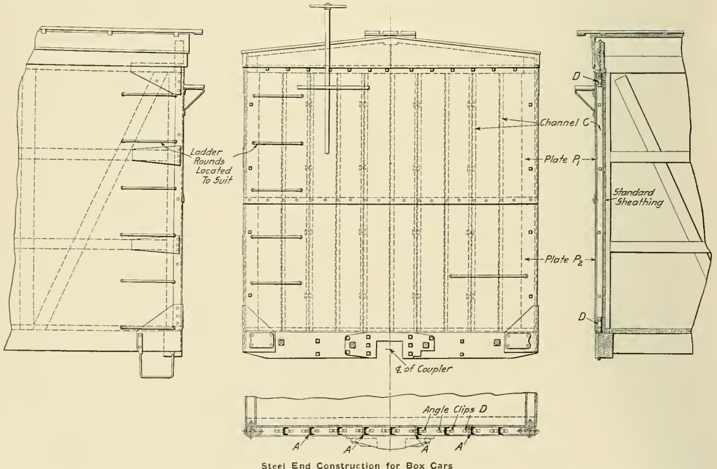
Steel End Construction for Box Cars
