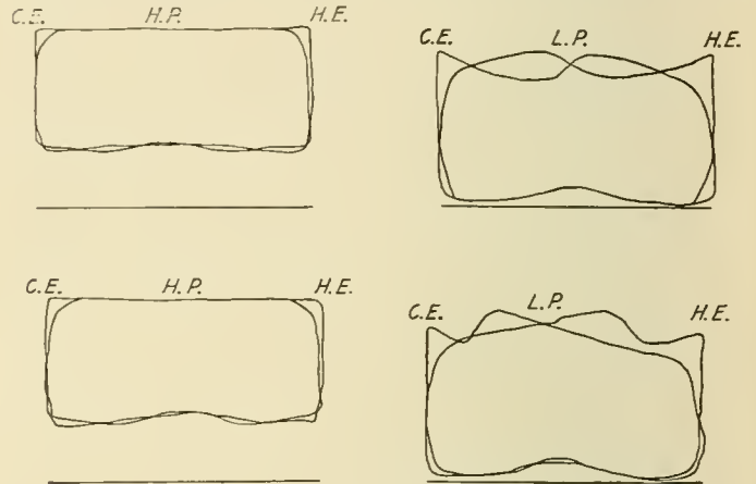
Fig. 6—Starting Cards of a Mallet
