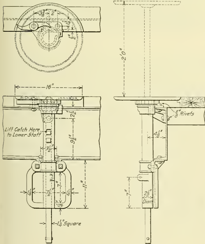
Application of the Union Drop Brake Shaft
