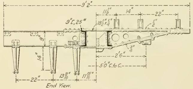
Cross Sections of the Box Car Underframe
