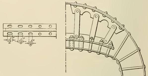
Fig. 5—Eliminating Crown Sheet Sagging
