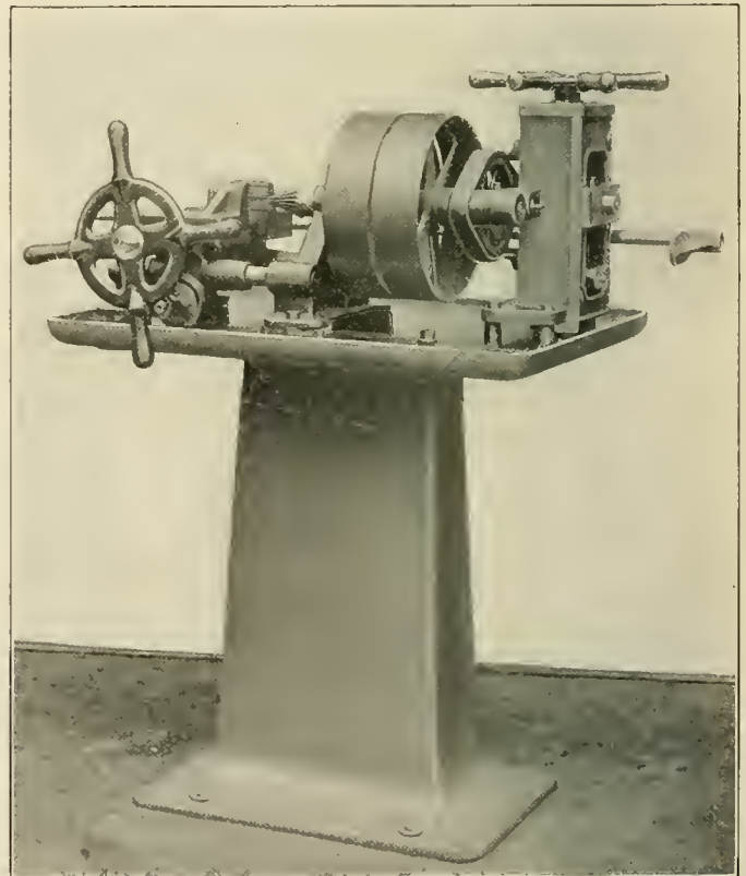
Oster Cutting Off and Reaming Machine for Pipe and Tubes
