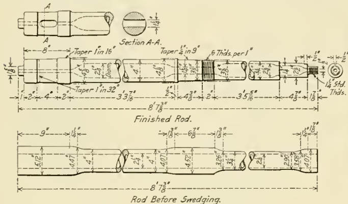
Hollow Piston Rod of Heat Treated Steel
