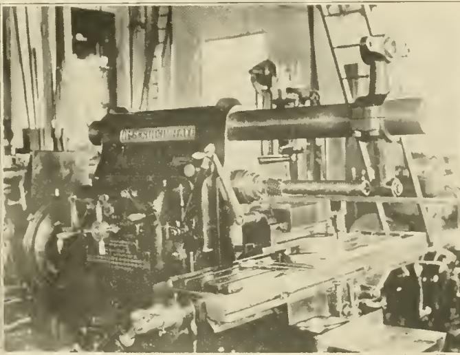
Fig. 14—High Speed Slitting Saws Making Rose Reamer Blades
