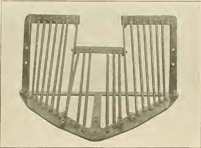
Long Nosed Pilot Formerly Used on the Lehigh Valley
