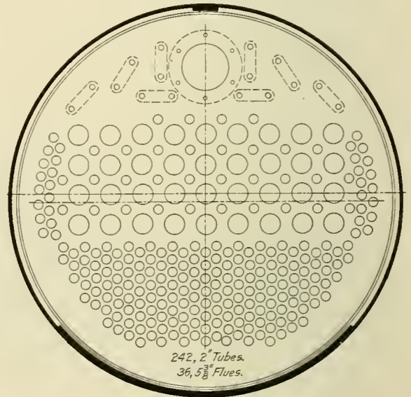
Section of the Boiler
