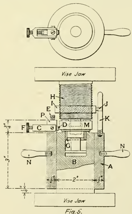
Part of the Equipment for Repairing Slide Valve Feed Valves
