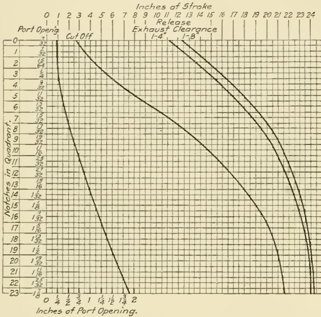
Fig. 2—Valve Event Diagram Typical of American Practice
