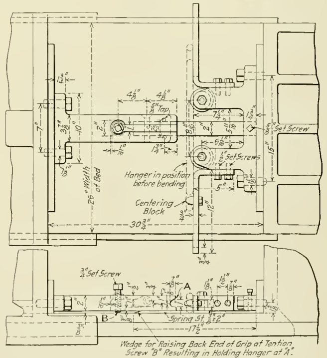
Fig. 3—Dies for Bending Brake Hangers
