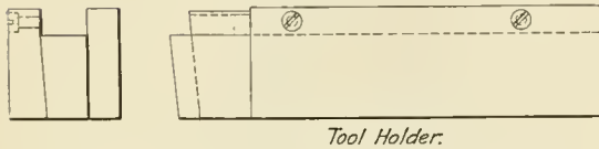
Right Hand Tool and Holder for 30 in. Wheel Lathe
