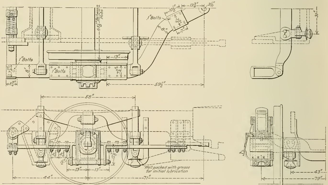
General Arrangement of the Austin Trailing Truck
