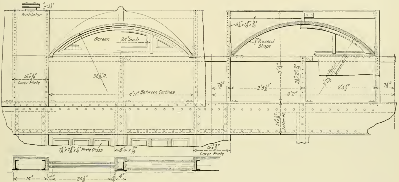
Roof Construction and Section Through Side Windows
