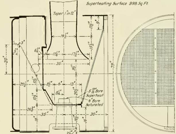
Fig. 8—Self-cleaning Front End for Saturated or Superheated Steam Locomotives
