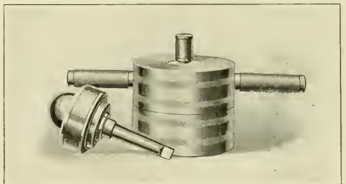
Mould Assembled for Casting the Grinding Sphere and Chuck with Grinder in Position
