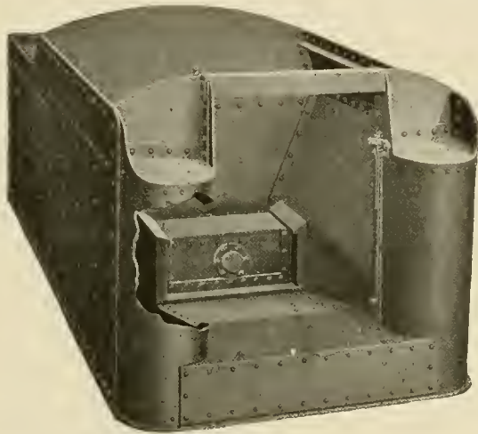
Reciprocating Coal Passer for Locomotive Tenders
