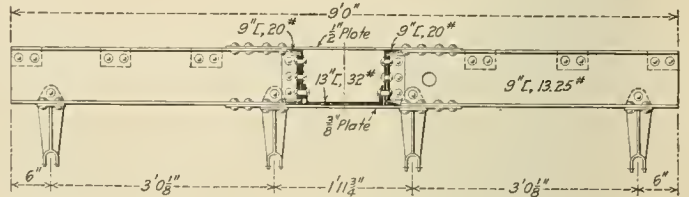
Cross Section Showing Connection Between Needle Beam and Intermediate Draft Sill
