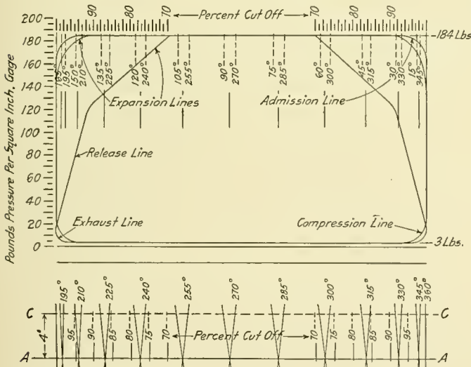
Fig. 8—Indicator Cards for 70 Per Cent. and 92 Per Cent. Cut-off
