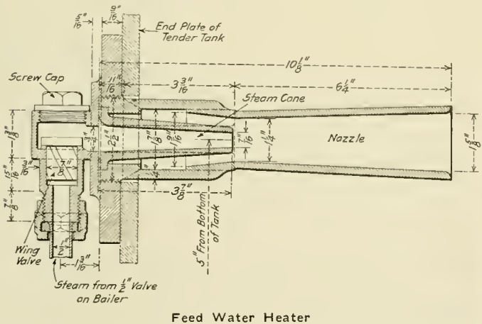
Feed Water Heater
