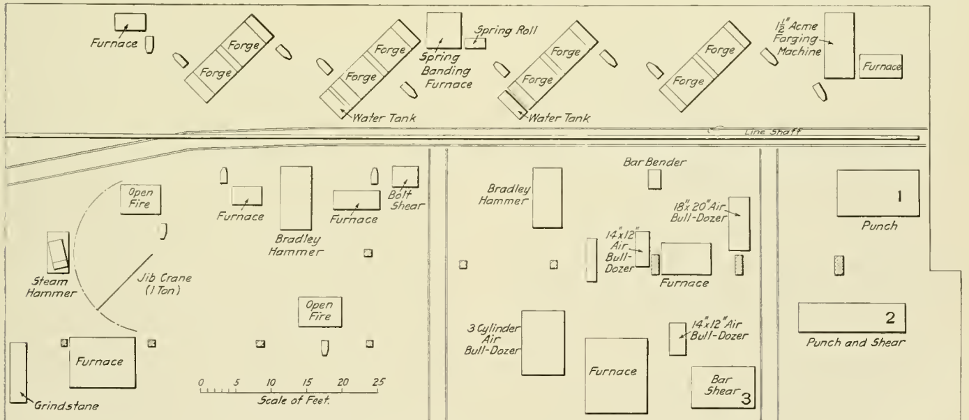
Fig. 3—Plan of Smith Shop After the Tools Had Been Rearranged
