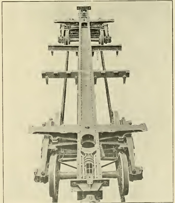
Steel Underframe for the Refrigerator Car
