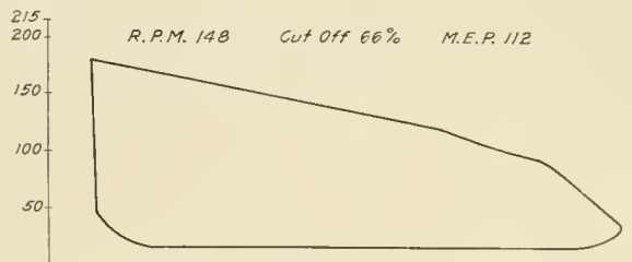
Fig. 1—Theoretical Indicator Diagram
