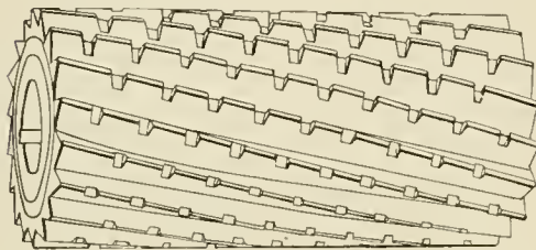
Fig. 2—New Style Milling Cutter Above; Old Style Below
