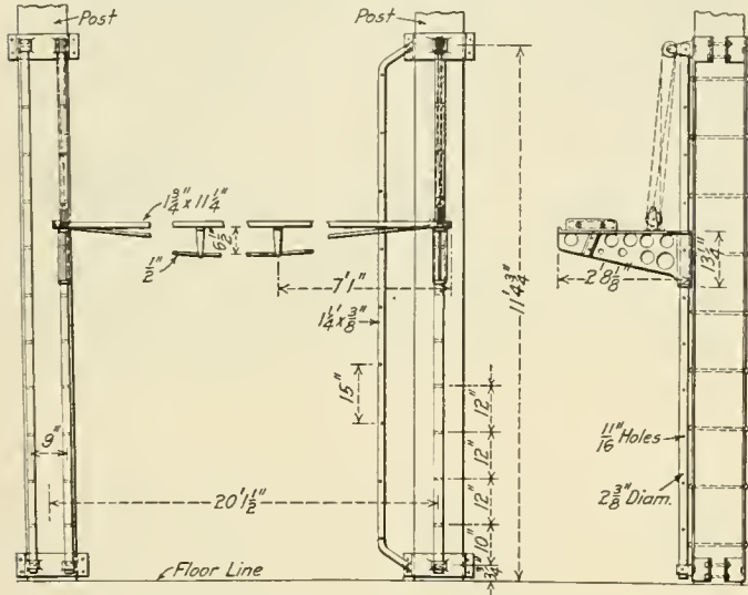
Adjustable Platform Used on the Intercolonial
