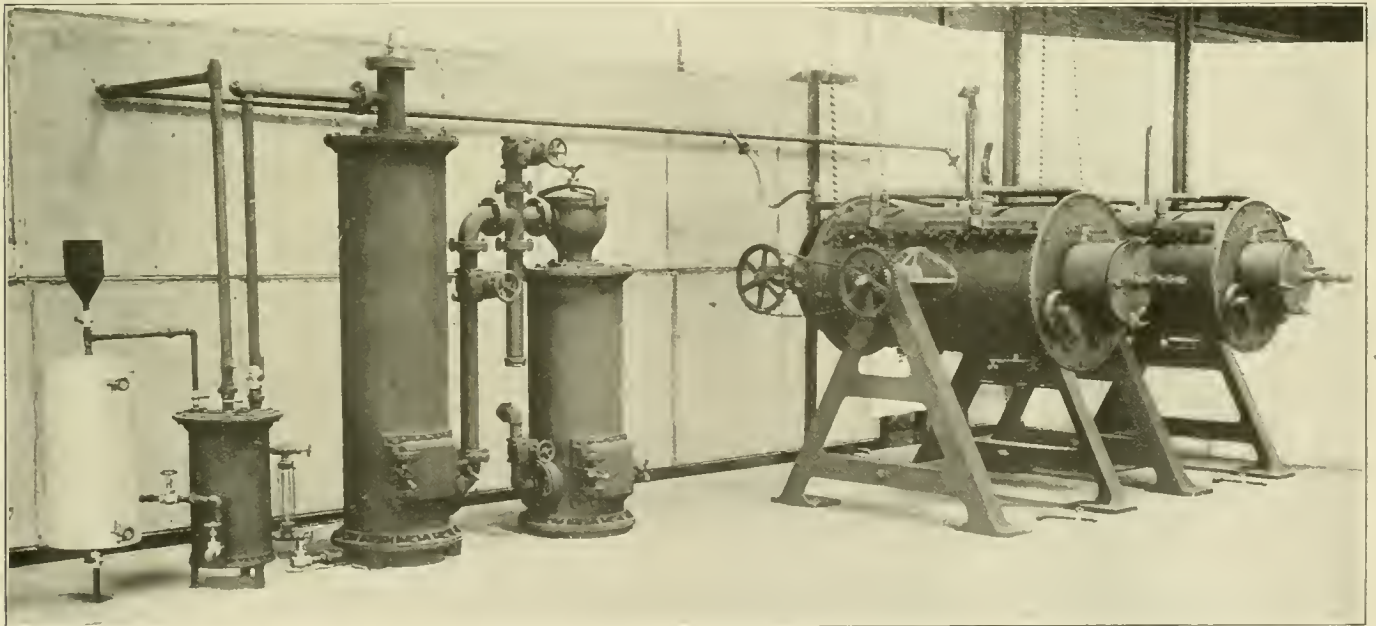
Complete Carbonizing Plant, Made Up of Gas Producer and Two Furnaces
