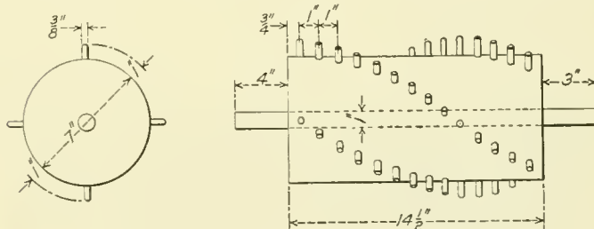
Fig. 3—Picker Used in Reclaiming Boiler Lagging
