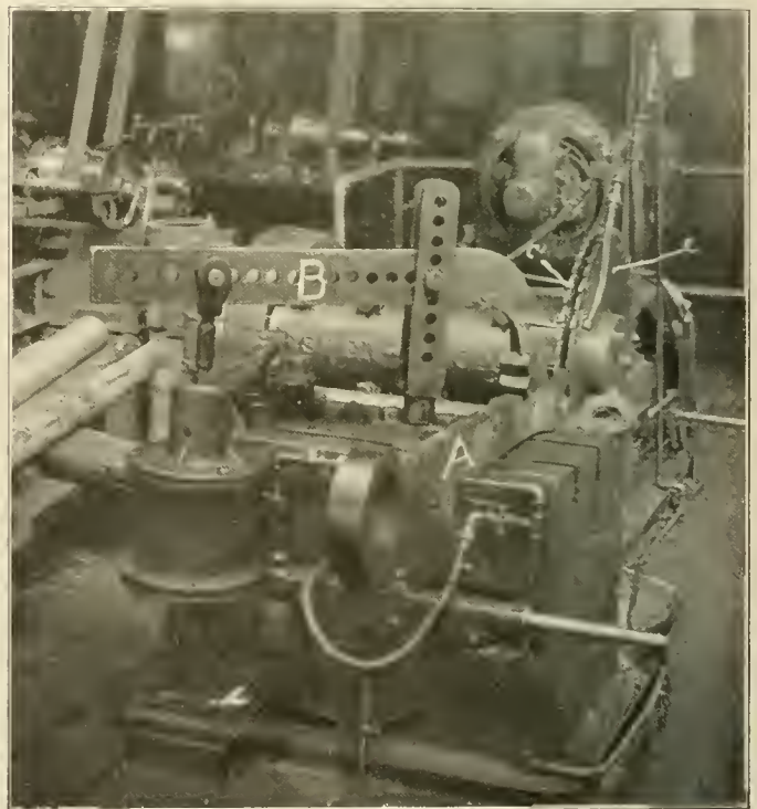
Fig. 5—Cutting Jaws in Locomotive Side Rods
