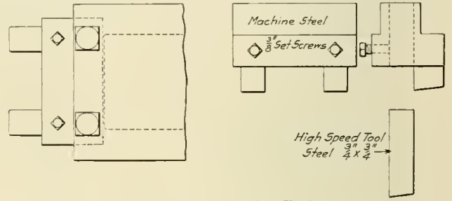
Holder for Grooving Tool
