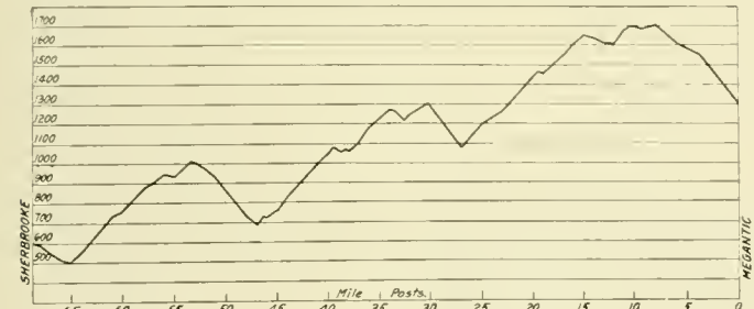
Profile of the Canadian Pacific Between Sherbrooke and Megantic
