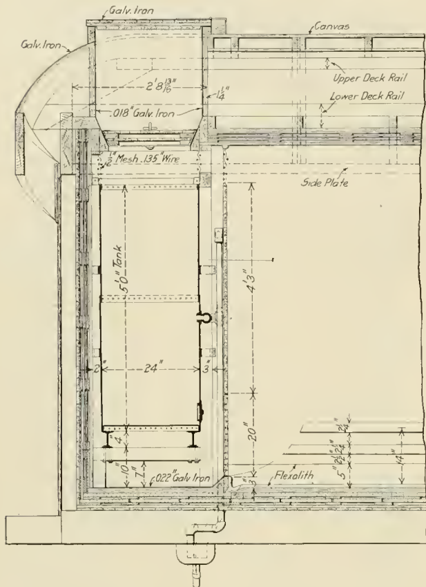
Sections Through the End of the Car Showing Arrangement of Brine Tanks
