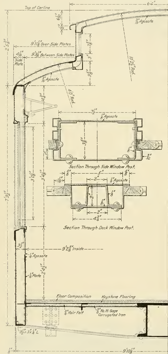
Sections Through the New Haven Coach
