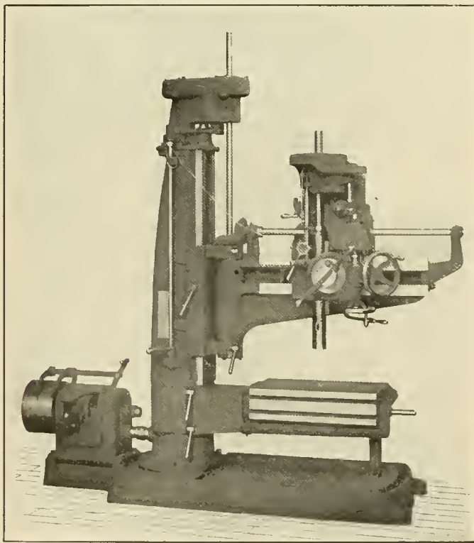
Three-Foot Box Column Radial Drill
