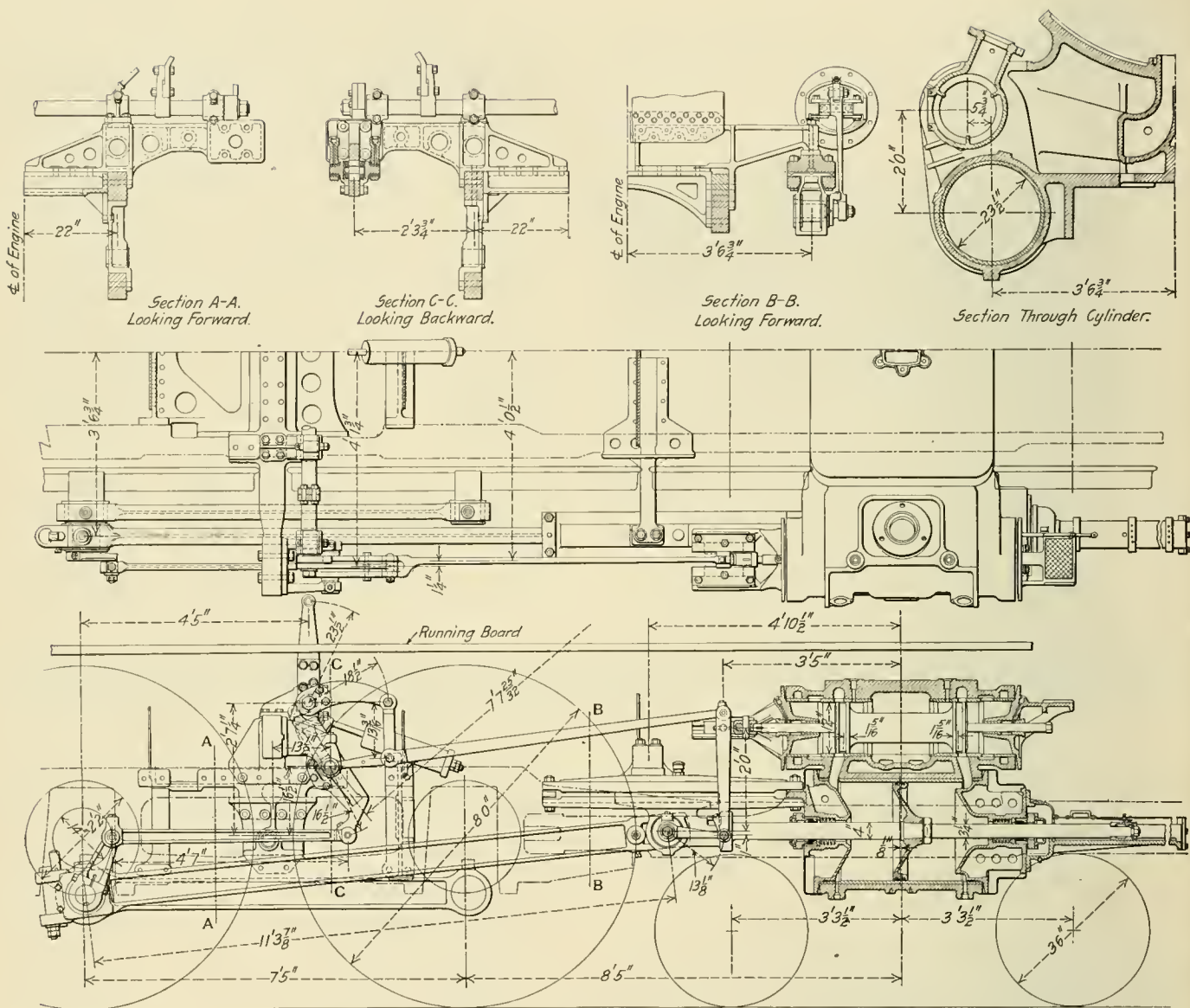
Valve Gear and Motion Work of the Pennsylvania Class E6s Locomotive
