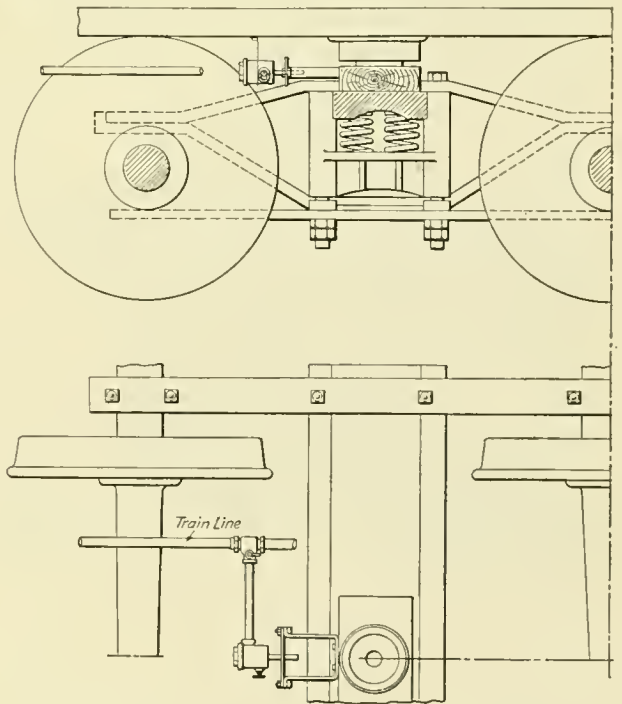
Arrangement of the Safety Release Valve on the Car
