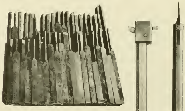
Forty-One Tools Formerly Used on Slotter
