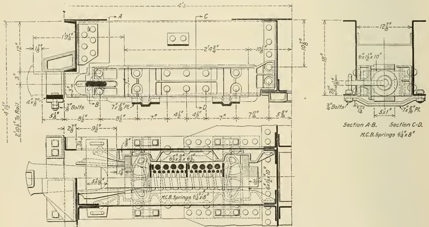
Application of Yost Draft Gear to a Steel Underframe Car
