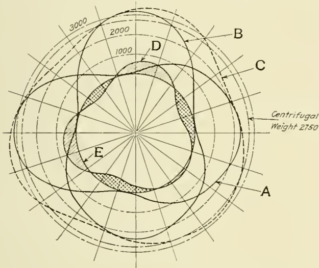
Inertia Diagram of Reciprocating Parts
