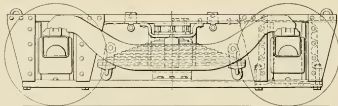
Structural Steel Pedestal Tender Truck
