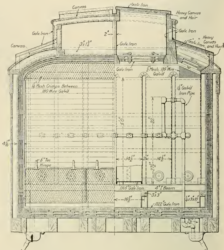
Sections Through the End of the Car Showing Arrangement of Brine Tanks
