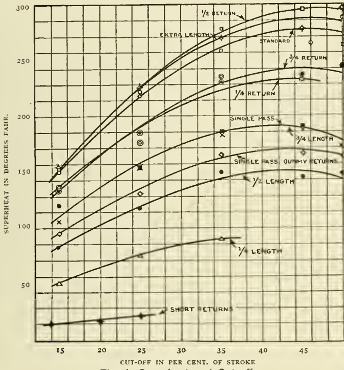
Fig. 4—Superheat and Cut-off
