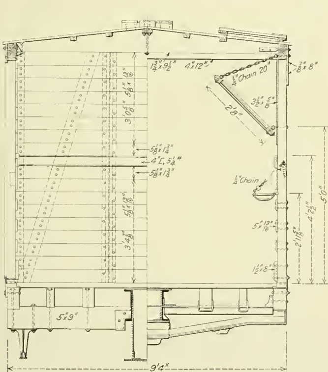
End Elevation and Cross Sections
