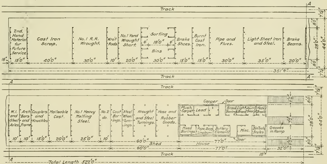
Plan Showing Arrangement of the Scrap Bins
