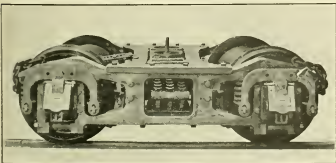
New Tender Truck on the Pennsylvania
