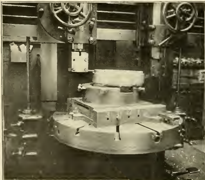
Jig Used for Machining Eccentrics
