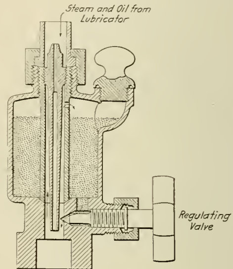
Cylinder Lubricator for Flake Graphite
