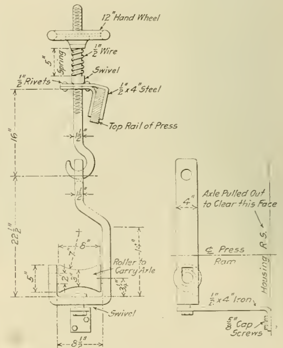
Fig. 9—Swivel Hook for Dismounting Press
