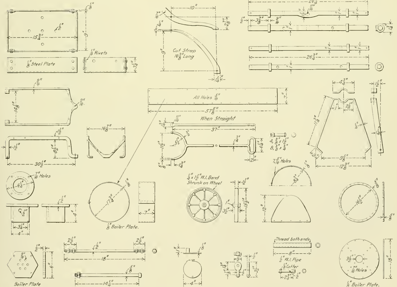
Fig. 2—Details of Portable Rivet Forge
