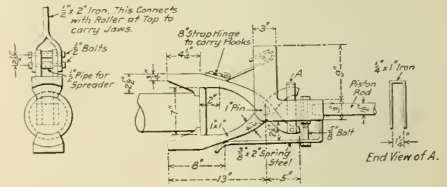
Fig. 8—Design of Hooks for Dismounting Press
