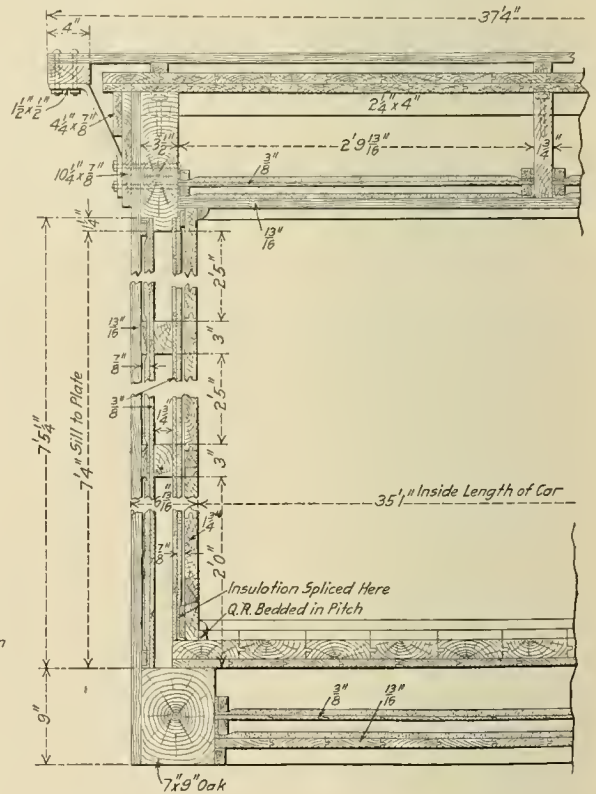
Insulation Details of the Milwaukee Refrigerator Transit & Car Company Dairy Car
