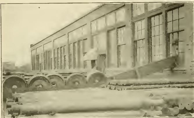
Fig. 6—Chute for Passing Scrapped Wheels out of the Shop
