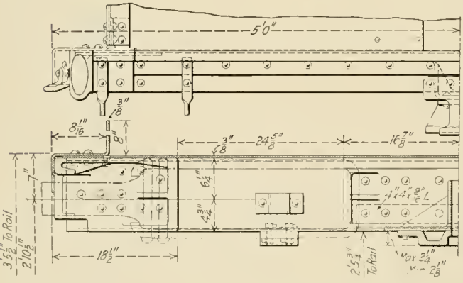
Arrangement of the End Sill and Corner Construction
