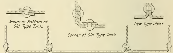
Section of New Type Tank Bottom.
