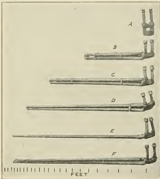
Fig. 1—Superheater Elements
