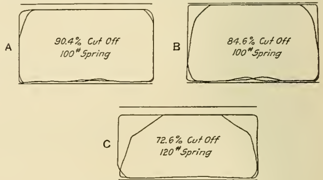
Fig. 7—Typical Cards for Slow Speed
