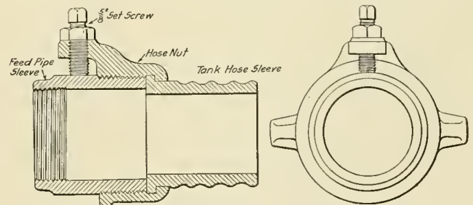
Check Nut for Tank Feed Hose Connections
