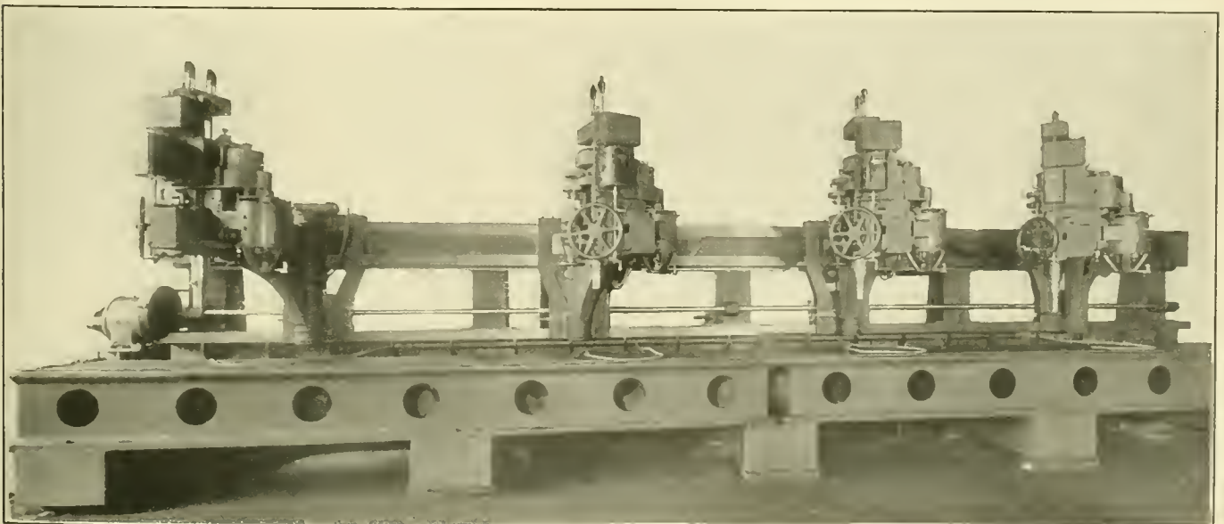
Four Spindle Radial Drill for Boiler Shop Work
