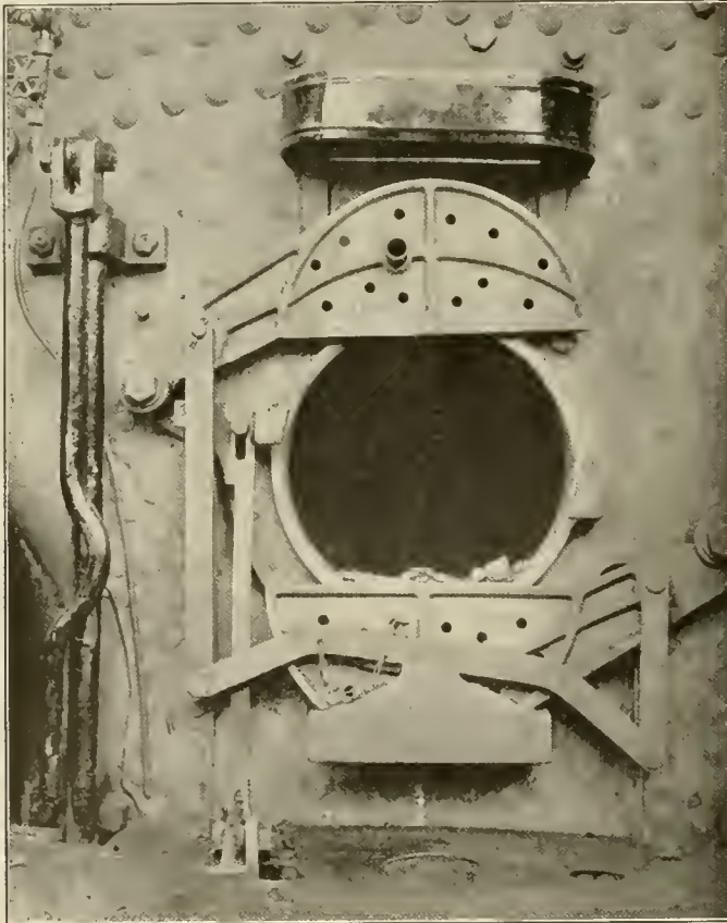
Gravity Fire Door Locked in Open Position
