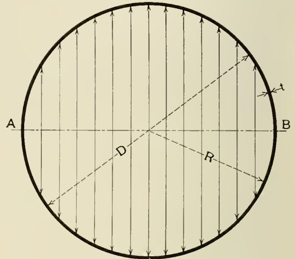
Fig. 1—Action of Steam Pressure, Tending to Burst the Shell
