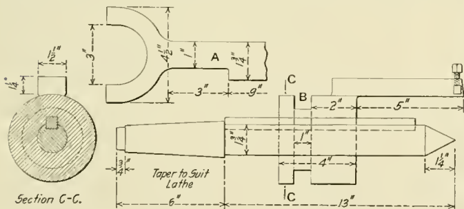
Fig. 8—Tool for Turning Tumbling Shafts
