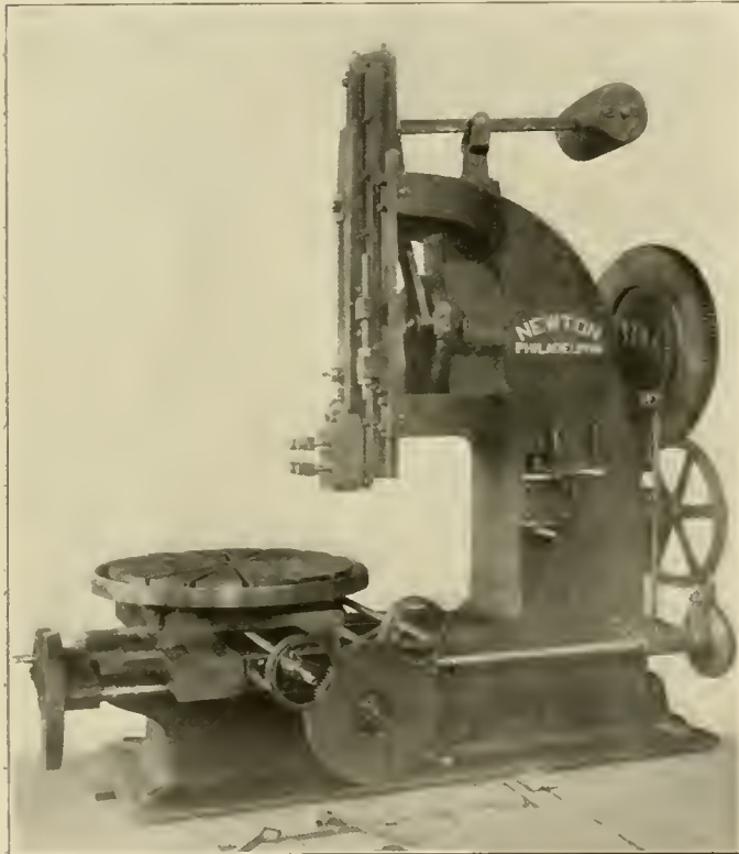
Slotting Machine With Inside Speed Box
