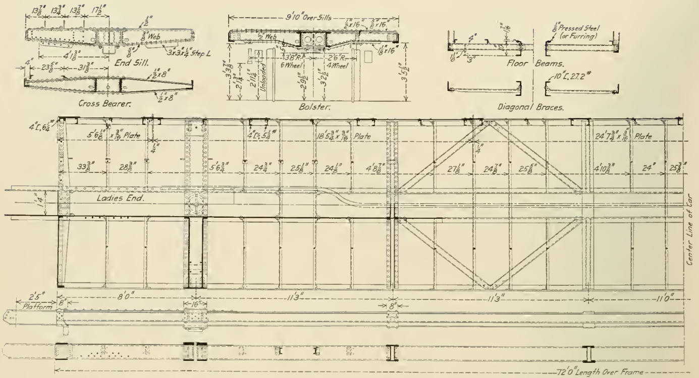
Underframe of the Canadian Pacific Steel Coach
