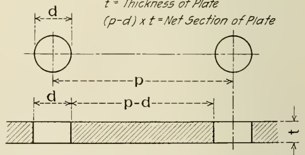
Fig. 2—Different Conditions After Drilling Holes
