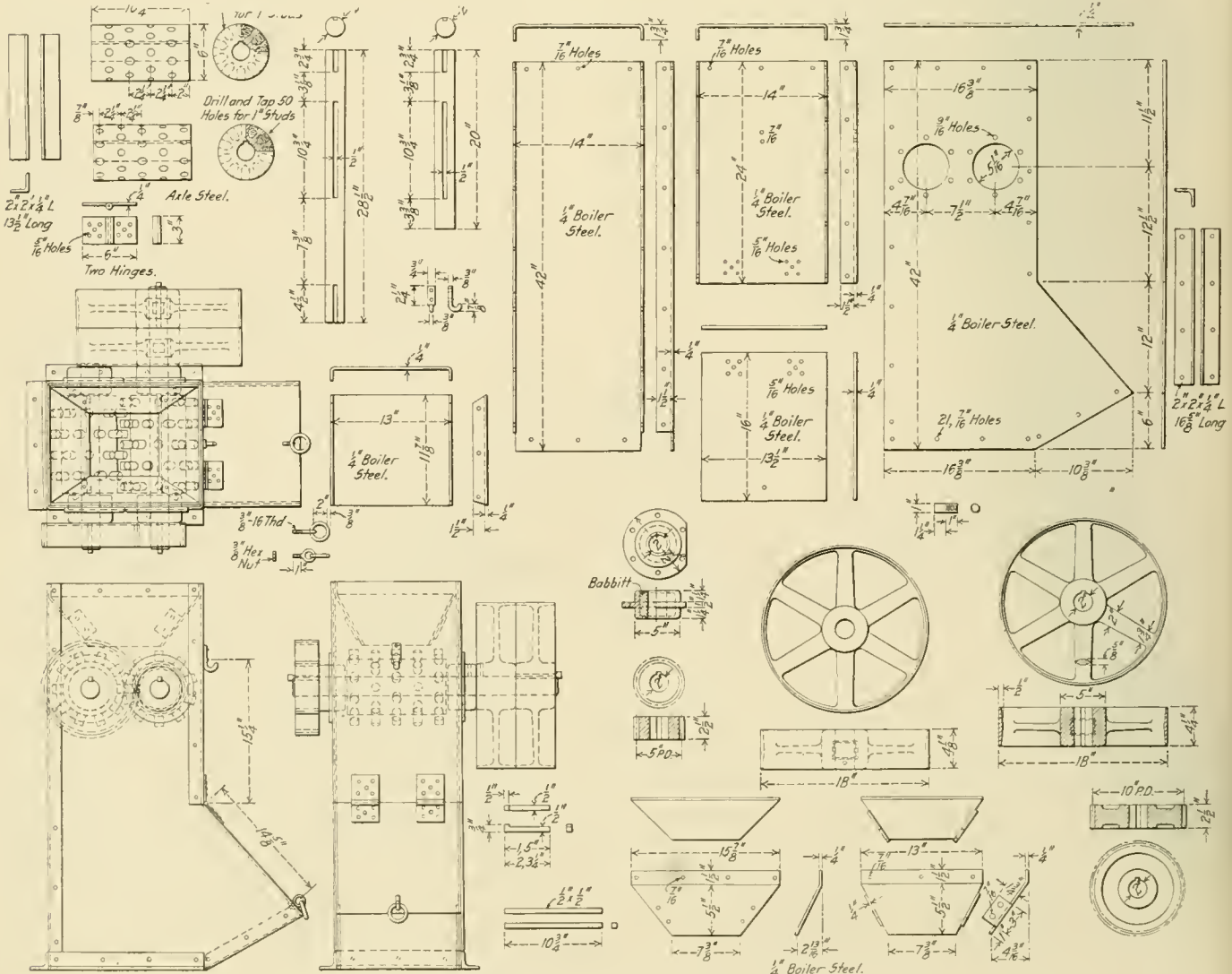
Fig. 3—Pulverizing Machine for Grinding Scrap Boiler Laggings
