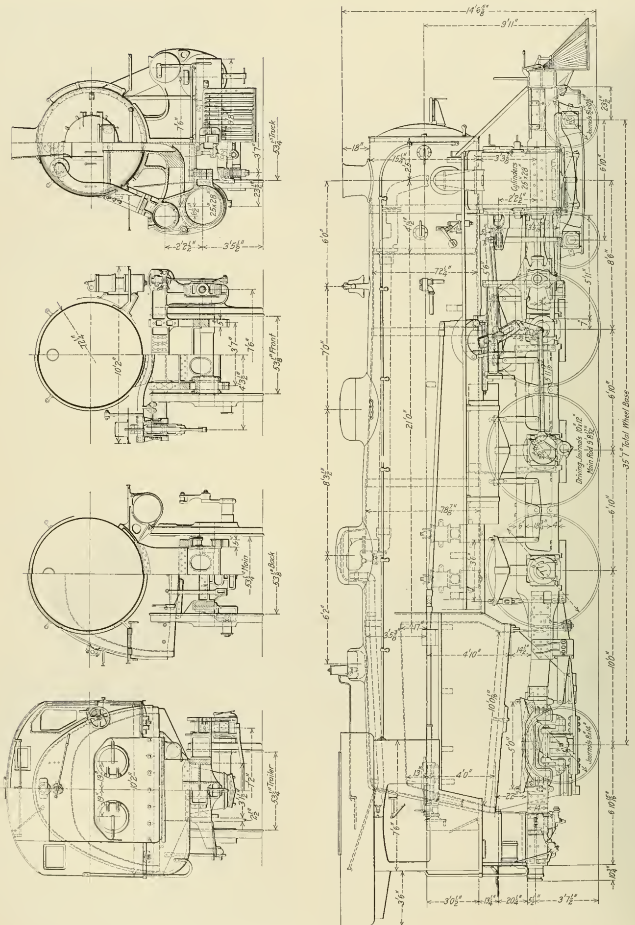
Pacific Type Locomotive Designed and Built by the Lehigh Valley
