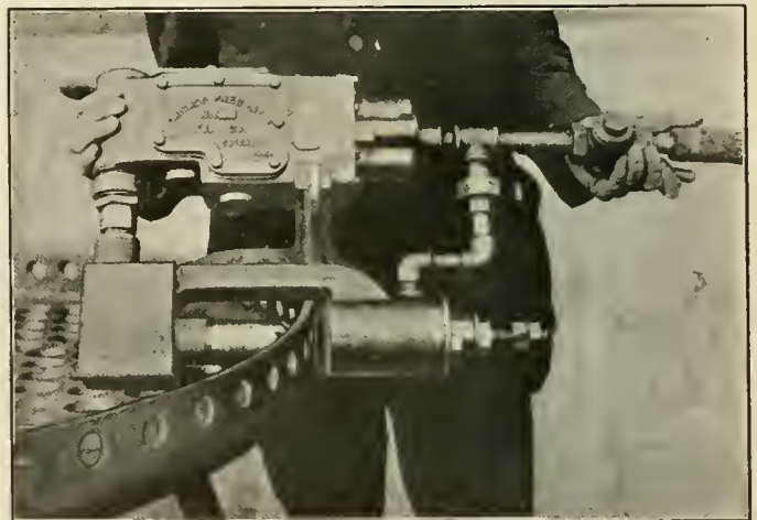
Device for Drilling and Countersinking Holes in Flanges
