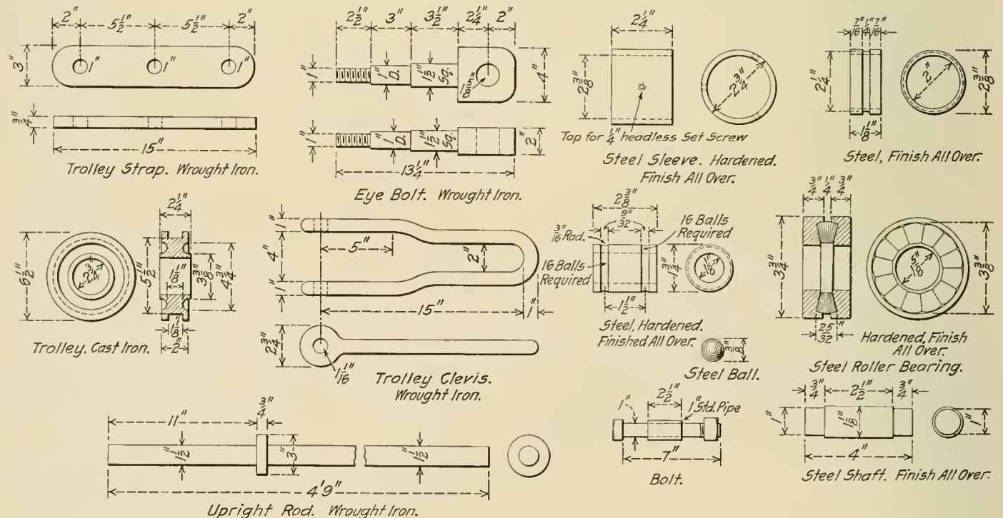
Details of Ball Bearing Crane and Trolley
