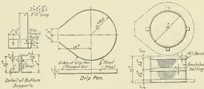
Details of the Drip Pan and Press Bucket
