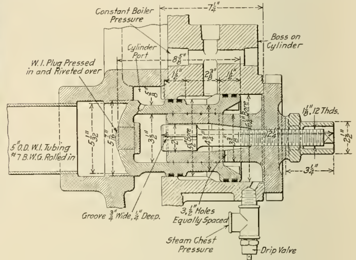
Section Through By-pass Drifting Valve Chamber
