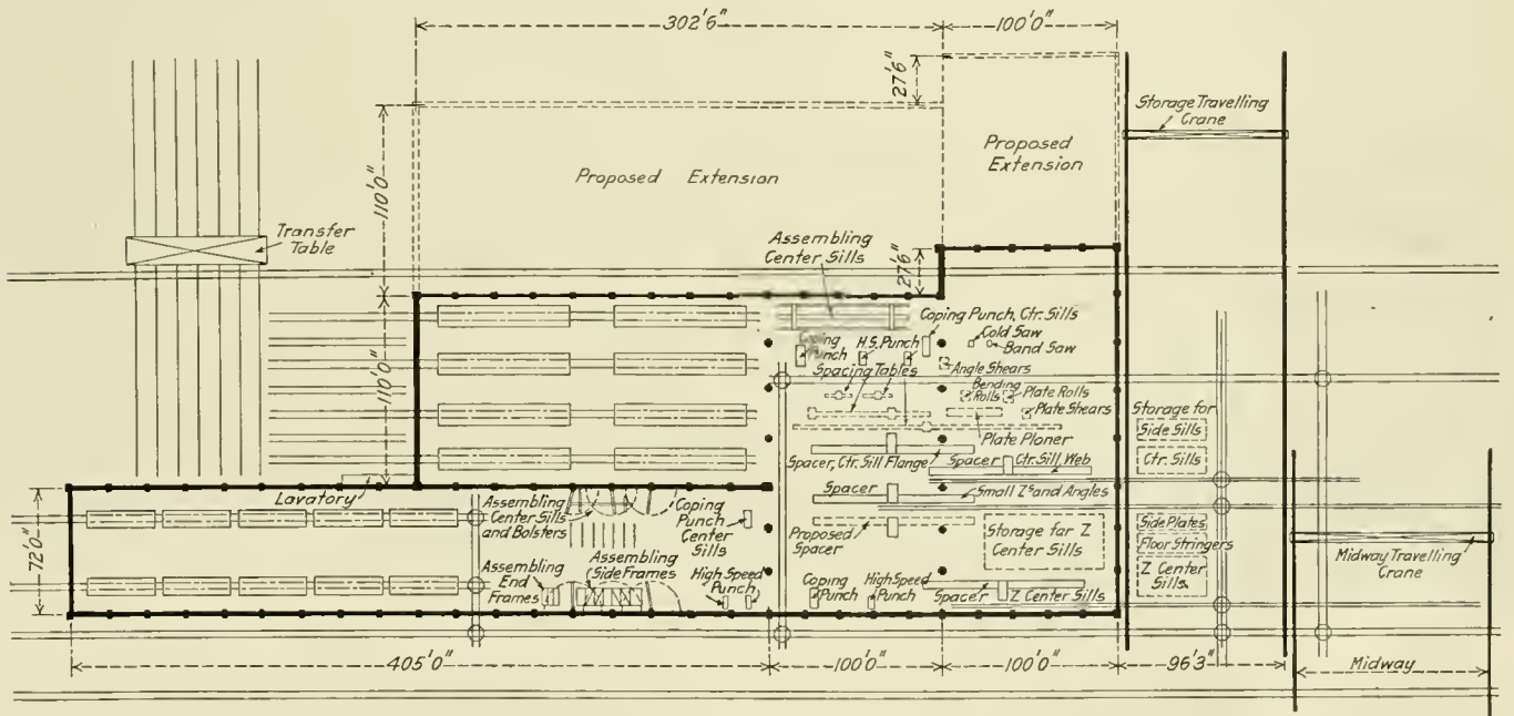
Plan of the Canadian Pacific Steel Car Shop
