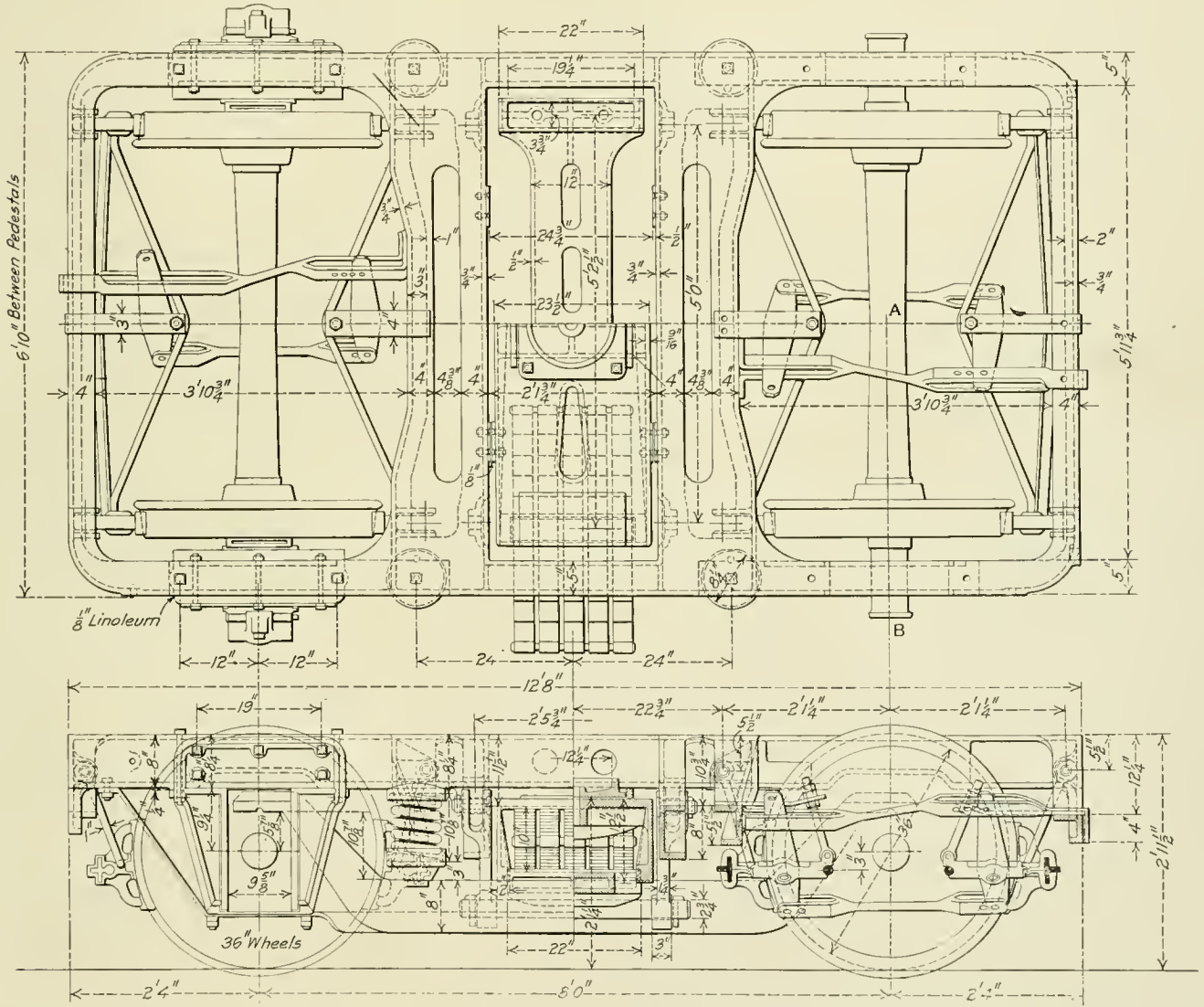
Four-Wheel Steel Truck with Clasp Brake Rigging Used on the Central of New Jersey Steel Cars
