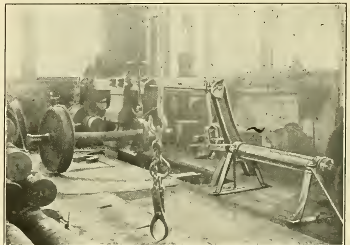
Fig. 4—Another View of the Dismantling Press Showing Air Cylinder and Grab Hook
