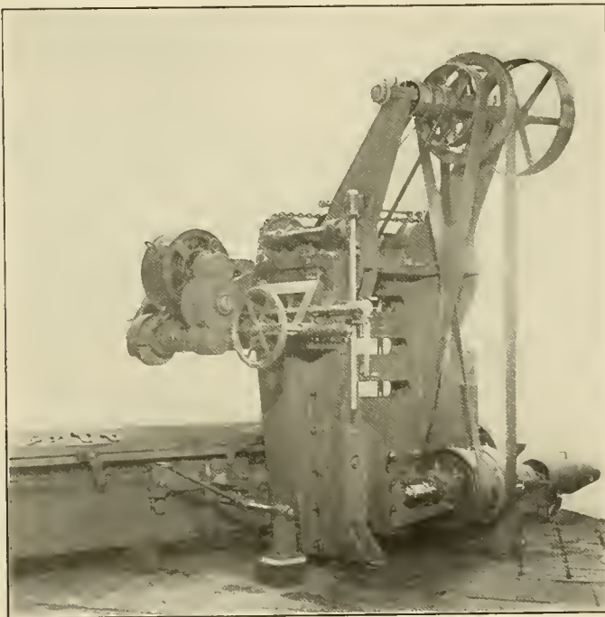
Open Side Planer Type Grinding Machine
