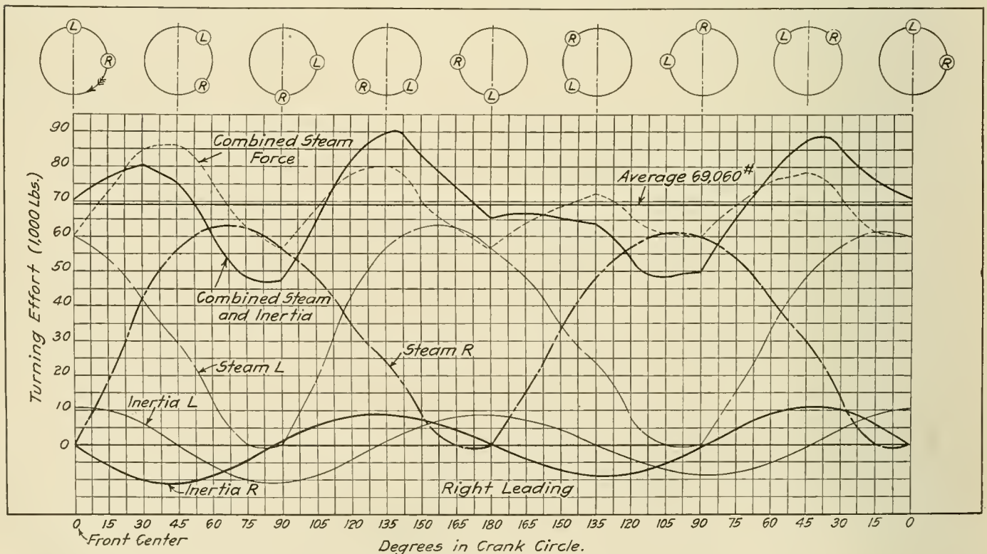
Fig. 2—Curve of Turning Moment for Lehigh Valley Pacific Type Locomotive
