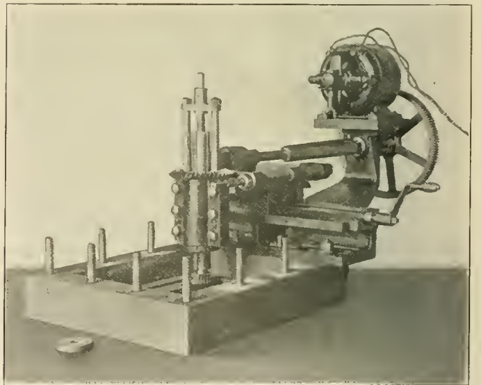
Portable Milling Machine
