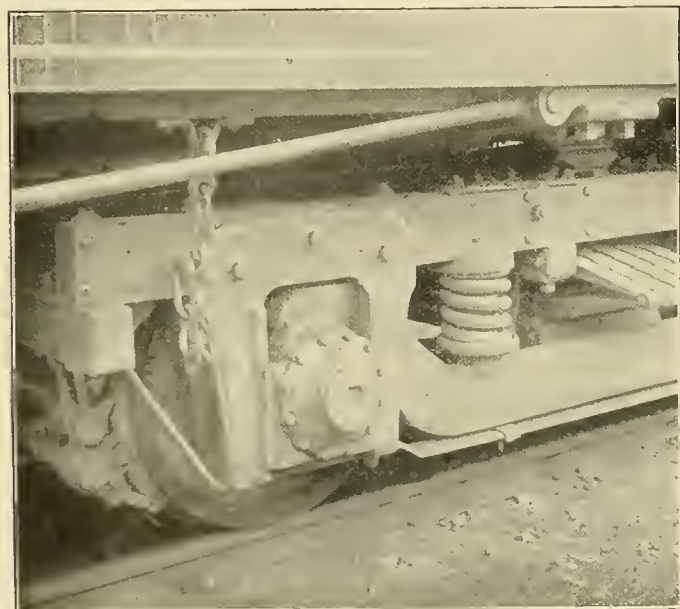
Appearance of a Truck Fitted with Roller Bearings
