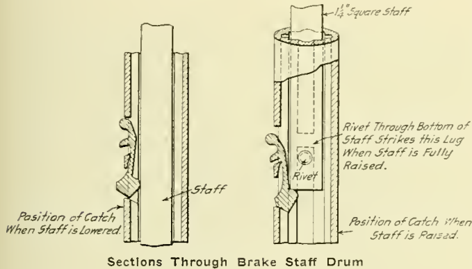
Sections Through Brake Staff Drum
