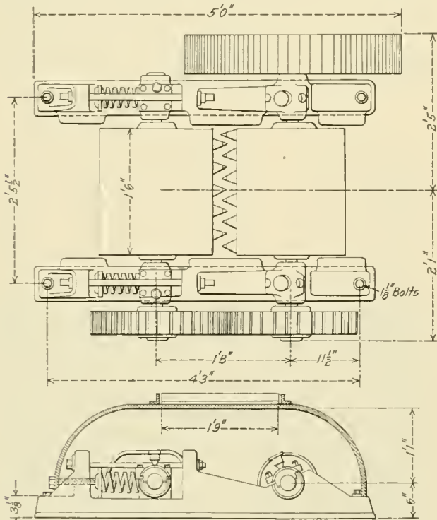
Spring Relief Coal Crusher Made by the Link Belt Company
