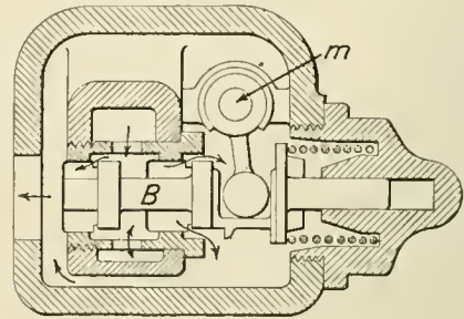
Fig. 9—Section Showing Valve of American Generator
