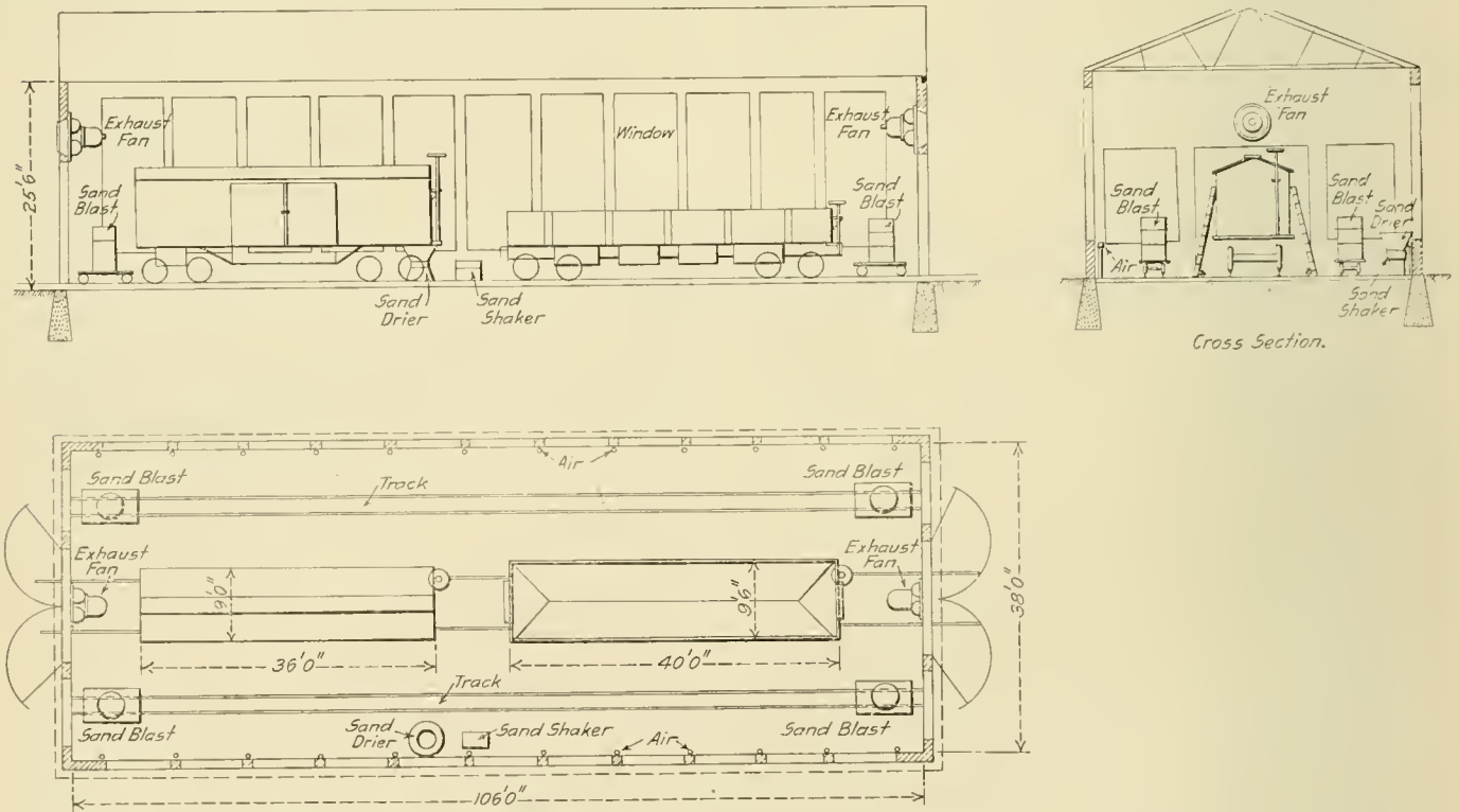
A Simpler Arrangement of Sand Blasting Equipment Which Omits the Pit and Sand Handling Apparatus
