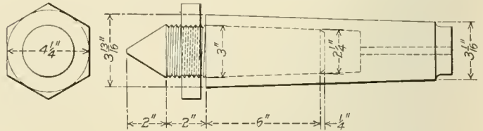
Center for Wheel Lathe
