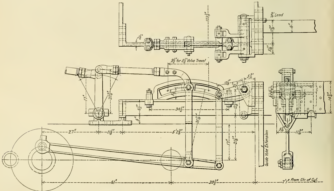
Arrangement of the Southern Locomotive Valve Gear
