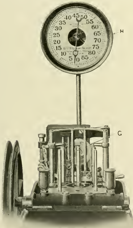
Boyer Speed Recorder with Clock Attachment
