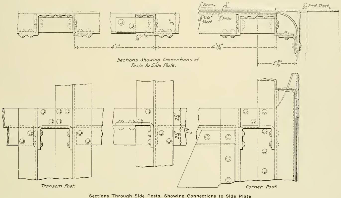
Sections Through Side Posts, Showing Connections to Side Plate
