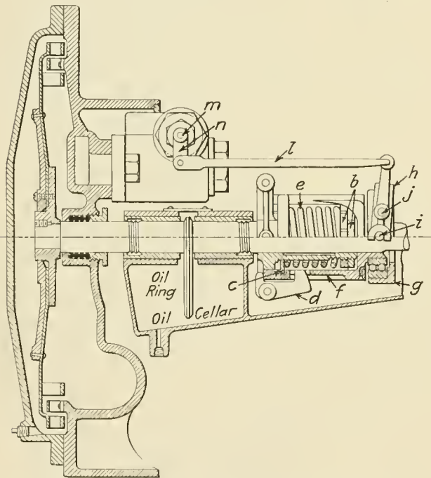
Fig. 8—Turbine End of American Generator
