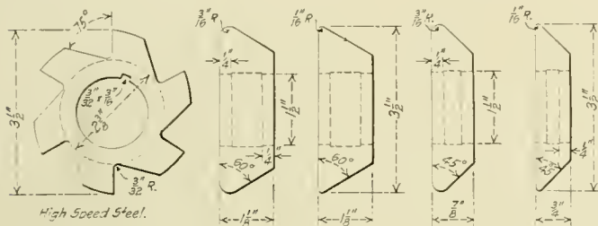
Fig. 8—Milling Machine Cutters
