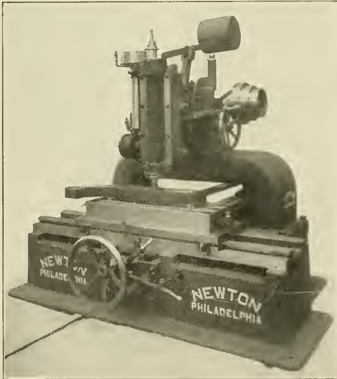
Link Grinding Machine of Substantial Construction
