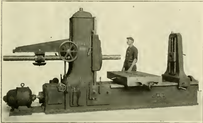
Horizontal Boring, Drilling and Milling Machine
