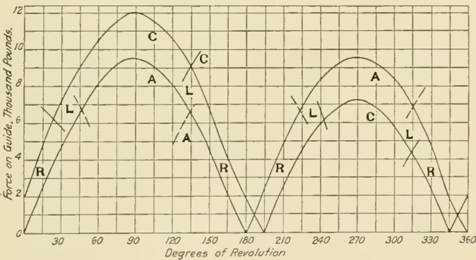
Fig. 10—Pressure on the Guides During One Revolution
