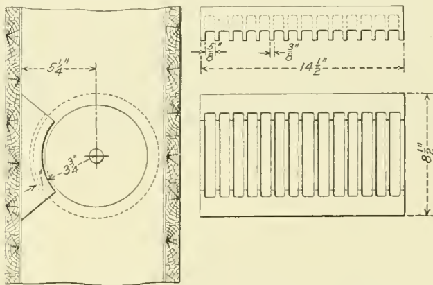
Fig. 4—Toe Plate Showing the Picker in Position
