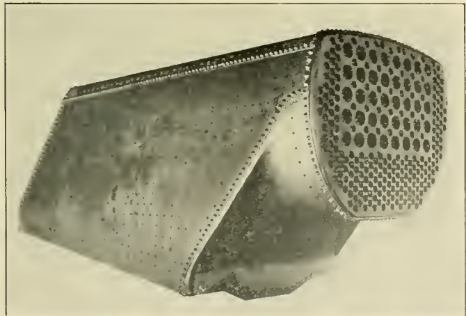
The Assembled Firebox for the Pennsylvania Locomotives
