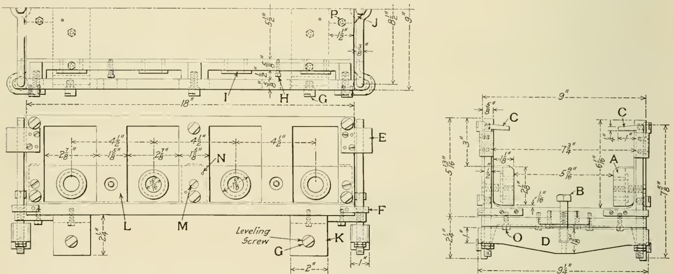
Jig for Drilling Crosshead Shoes.
