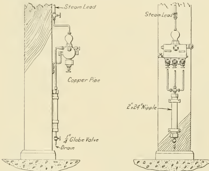
Rack for Testing Lubricators in the Roundhouse
