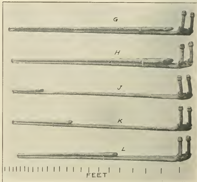
Fig. 2—Superheater Elements
