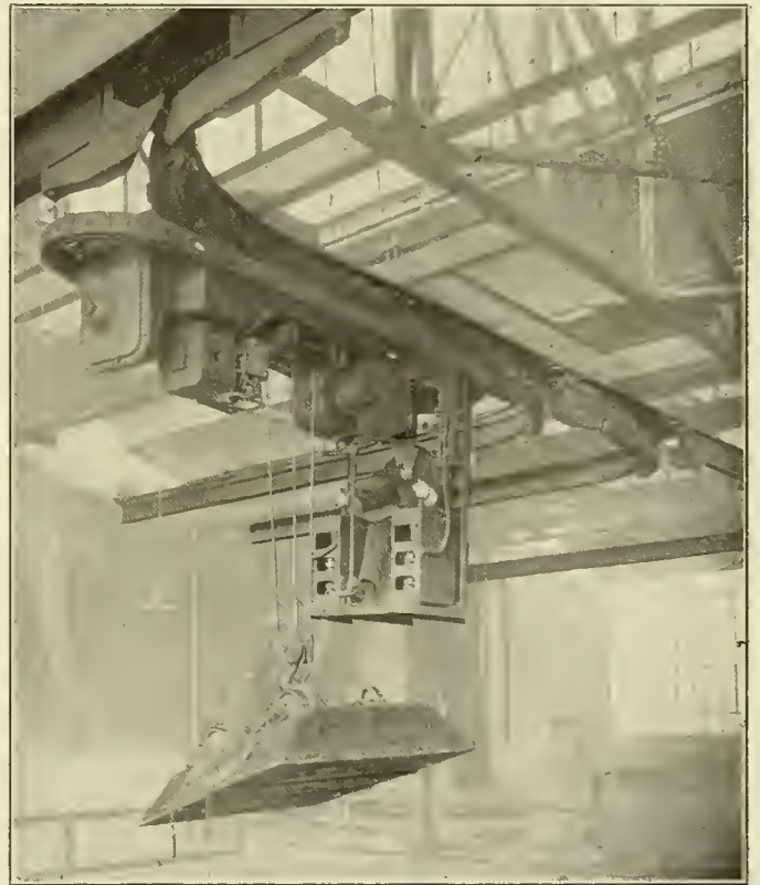
Fig. 1—Two-Motor Monorail Hoist Operating on Track System with Fixed Tongue Switches
