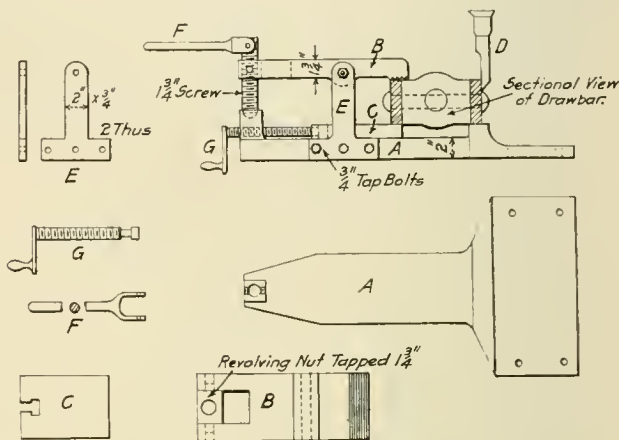
Fig. 1—Tool for Shearing Drawbar Rivets
