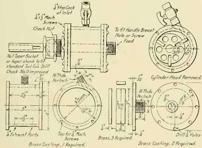
Fig. 6—Air Motor for Light Drilling
