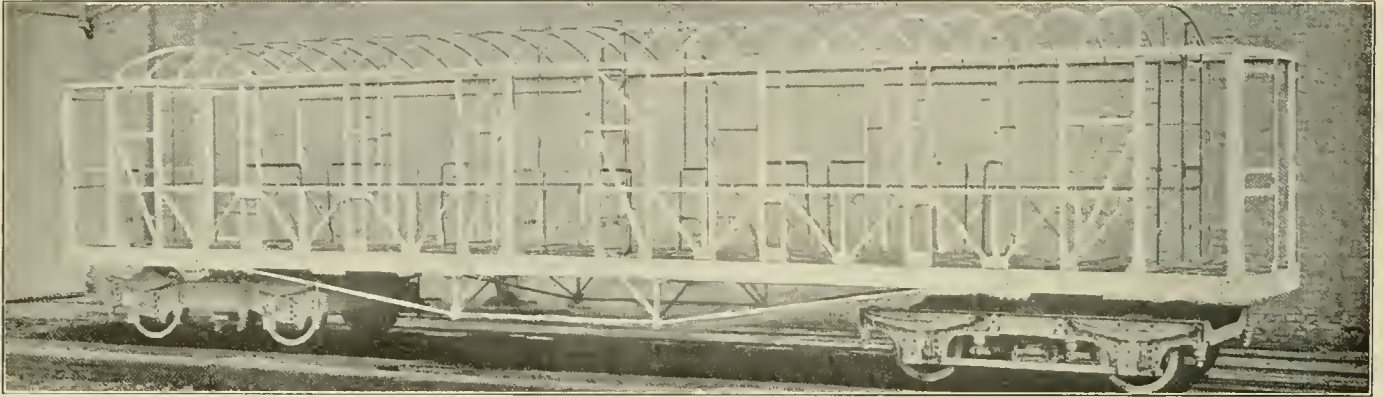
Steel Framing for the Metropolitan District Car
