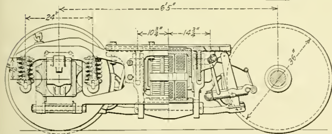
Improved Tender Truck
