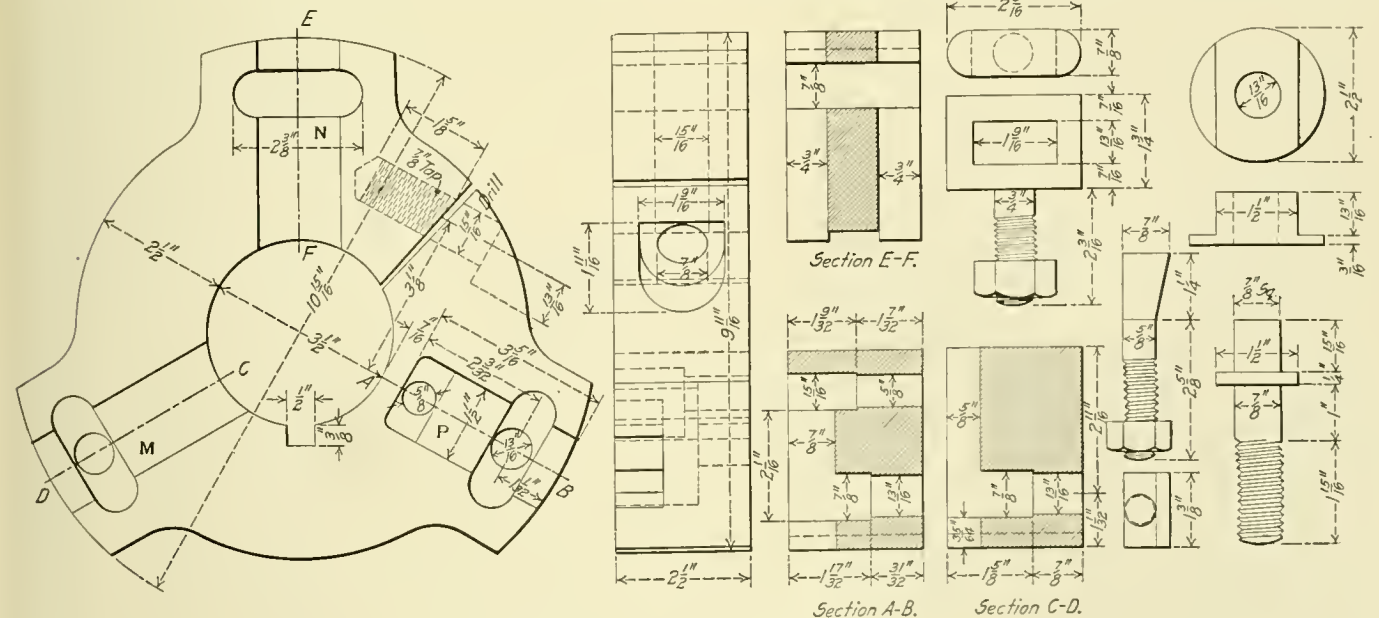
Fig. 2—Sections Through Three Tool Boring Head
