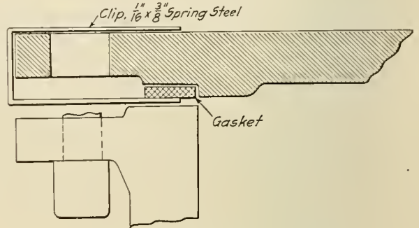
Clip for Holding Gaskets in Position
