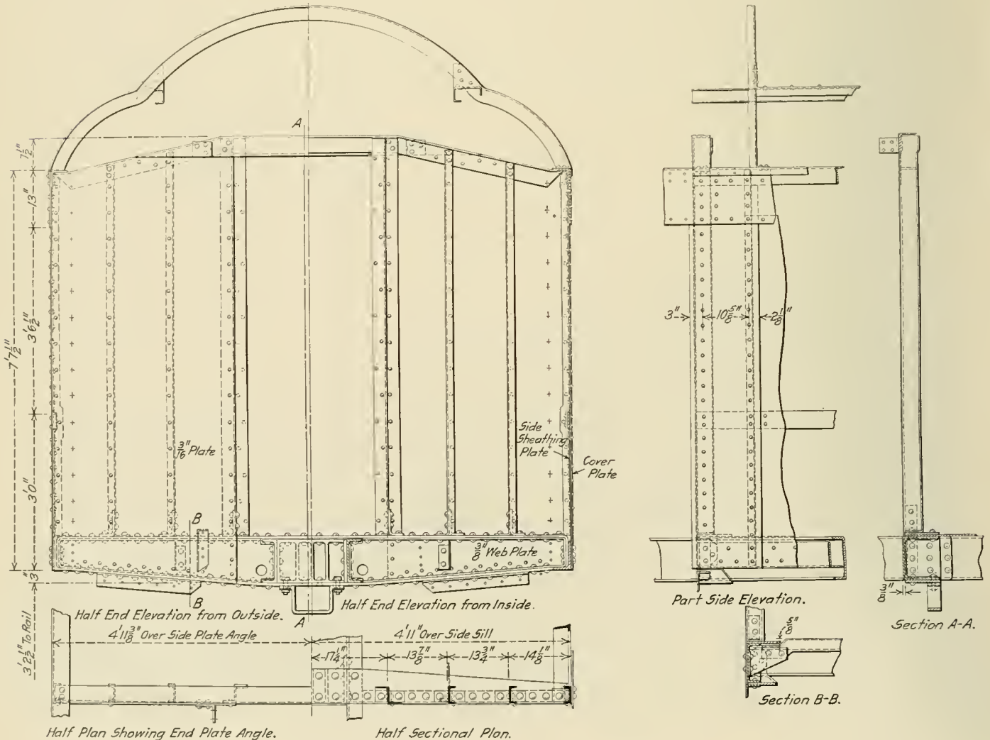
End Construction of Steel Coach on the Canadian Pacific
