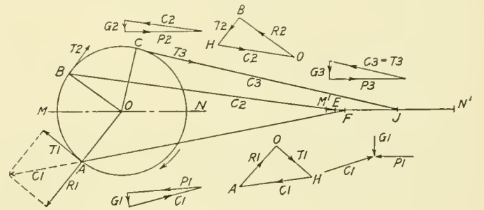
Fig. 9—Graphical Representation of the Tangential Force at the Crank Pin
