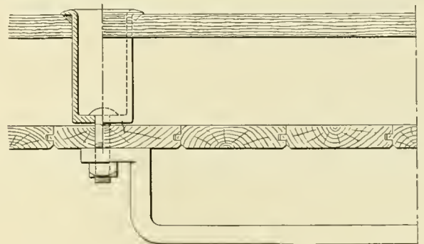
Socket Washer Used in Applying a Grab Iron
