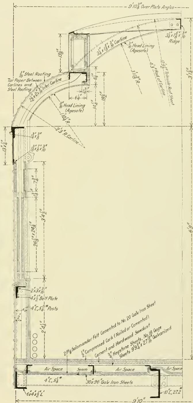
Cross Section Through Canadian Pacific Steel Coach
