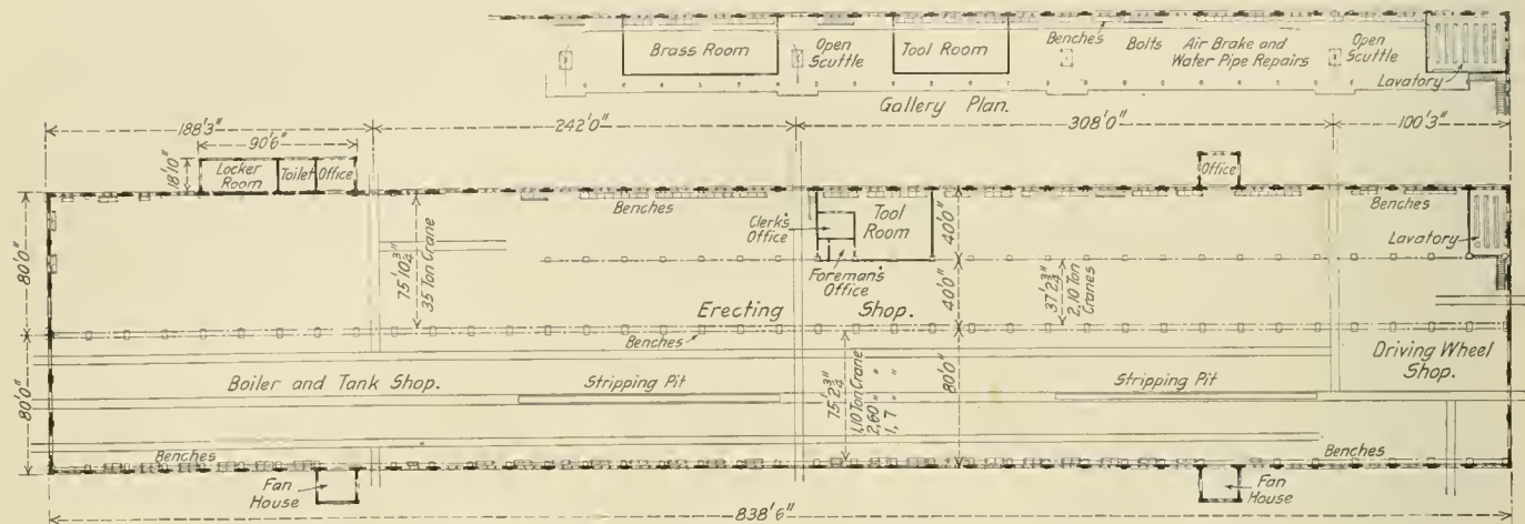
Plan Showing Arrangement of the Locomotive Shop
