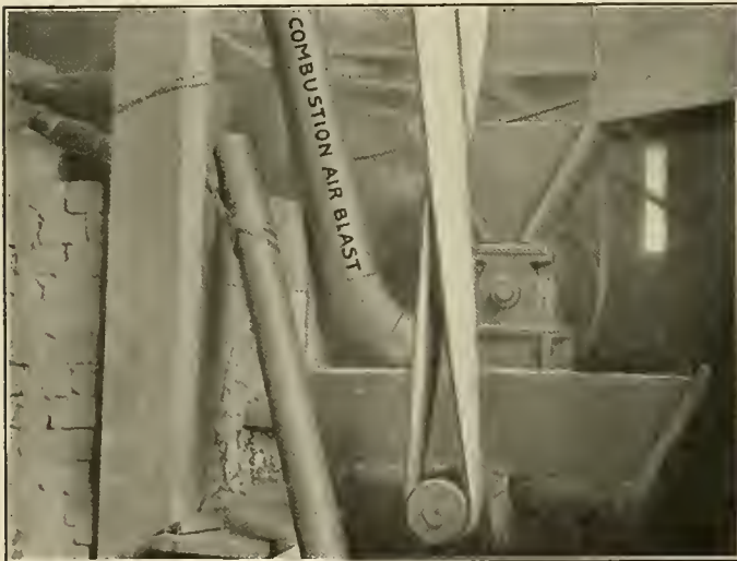
Fig. 1—Arrangement of Apparatus for Pulverizing Coal
