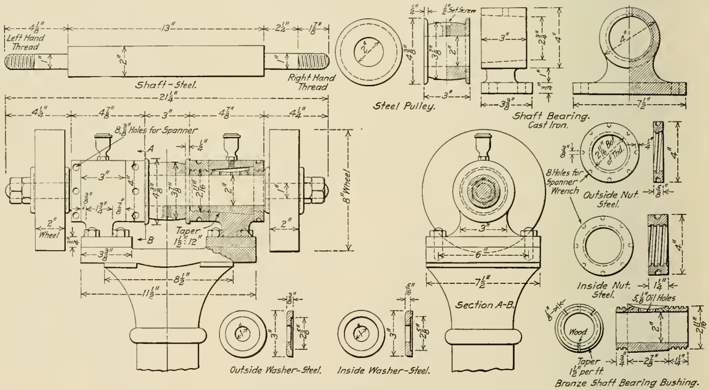
Arrangement and Details of Shop Emery Wheel Stand
