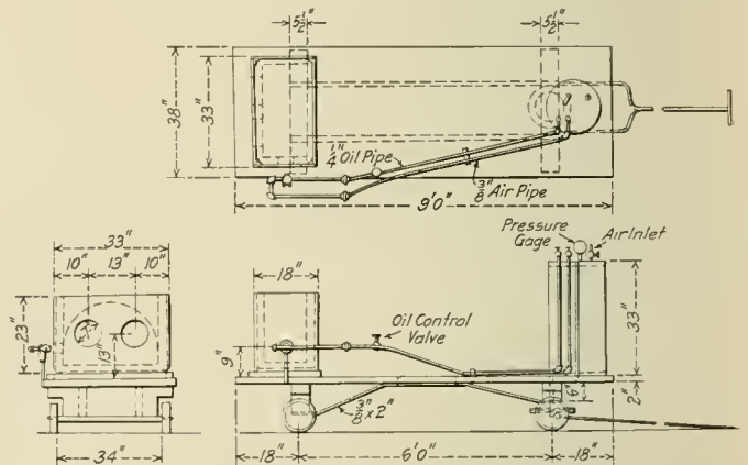
Furnace Used in Reclaiming Car Axles
