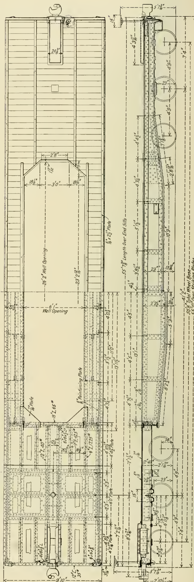
Plan and Sections of a Well Car with a Capacity of 220,000 lb.; Lehigh Valley
