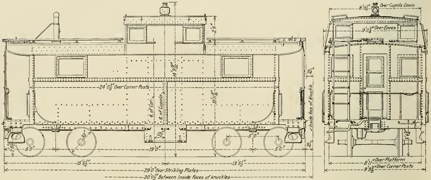
Elevations of the Pennsylvania Steel Caboose
