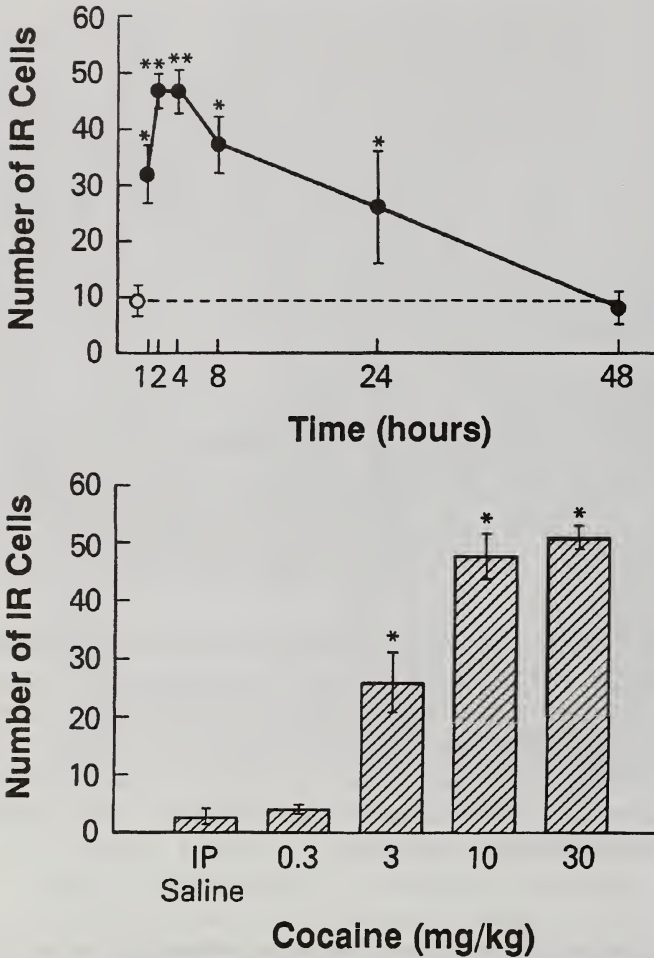
FIGURE 7. Time course and dose response of the increase in Fos-immunoreactive (IR) cell nuclei following cocaine 30 mg/kg IP. Upper panel: The peak elevation of Fos-immunoreactive proteins is seen between 2 and 4 hours and returns to control over approximately the next 24 hours. This contrasts with the increase in c-fos mRNA, which peaked sharply at 30 minutes. Lower panel: The increase in Fos-immunoreactive protein staining occurred over the same dose increase in mRNA. Data were collected 2 hours after injection. Stained nuclei were counted regardless of intensity. However, the intensity increased progressively, especially between 10 and 30 mg/kg. At the latter dose many neurons were very dark brown, almost black, in color. * p < 0.05 , ** p < 0.01 .
