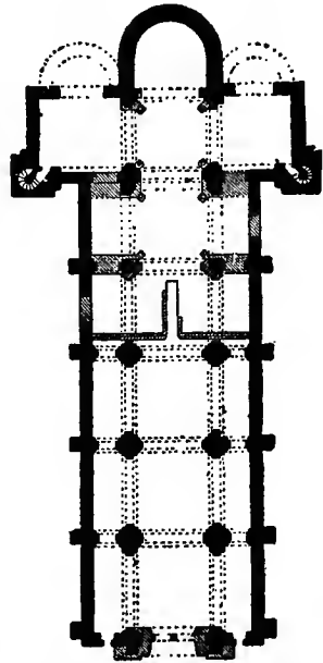
PLAN OF THE CHURCH OF ST. TROPHIME, ARLES FROM CORROYER'S "ARCHITECTURE ROMANE"
