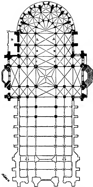
PLAN OF CATHEDRAL OF BEAUVAIS
