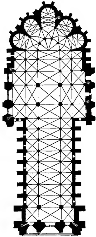
PLAN OF THE CATHEDRAL OF RHEIMS FROM VIOLETT-LE-DUC'S "DICTIONNAIRE DE L'ARCHITECTURE"
