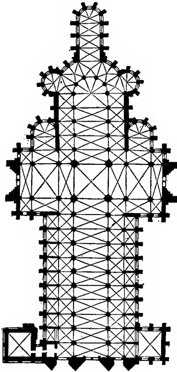
PLAN OF THE CATHEDRAL OF ROUEN
