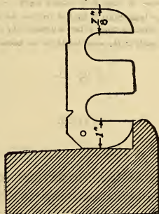
Method of Gauging Worn Flanges. See Rule 10.
