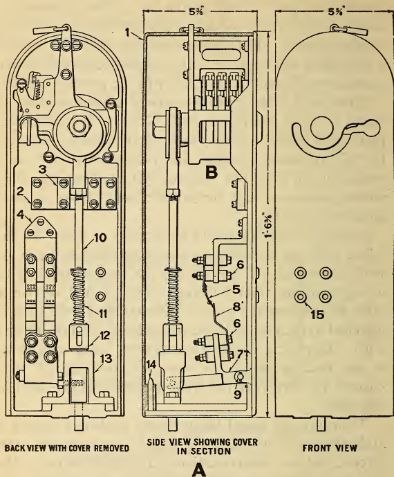
FIG. 129. STAFF LEVER LOCK.
