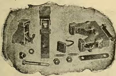
FIG. 90. BUCKER BRUSH HOLDERS AND DETAILS.
