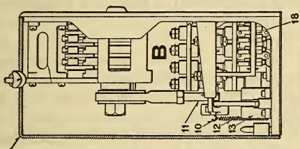
SIDE VIEW SHOWING COVER IN SECTION
