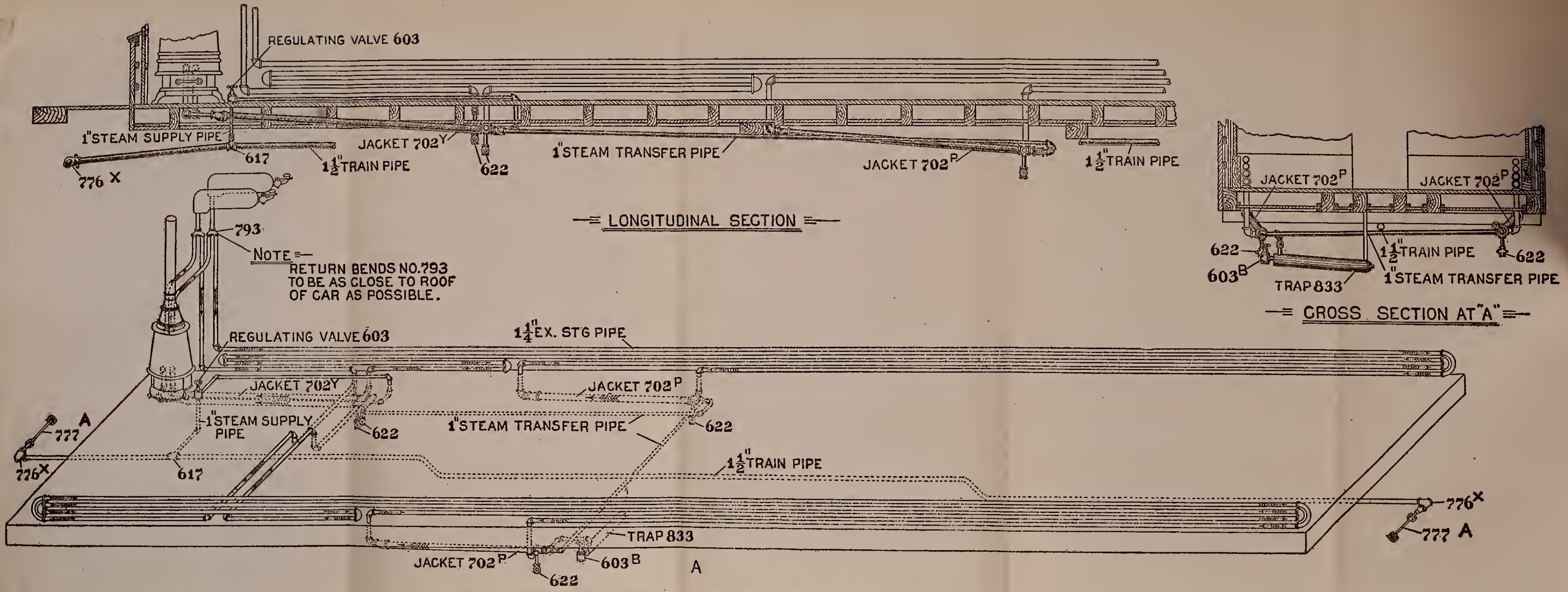
PLATE 2. Design showing Standard Heating System as used with Double Circulation Baker Heaters.
