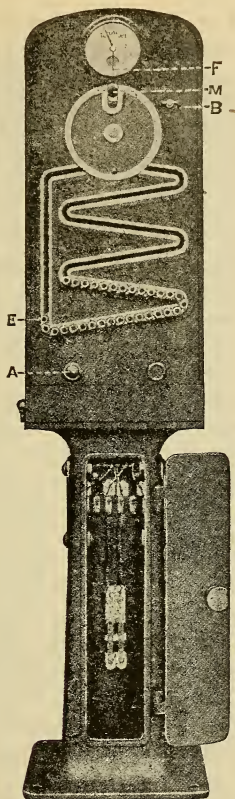
FIG. 120. ABSOLUTE STAFF INSTRUMENT WITH PEDESTAL. Front View Showing Door of Pedestal Open.
