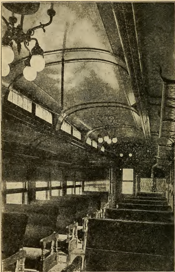
FIG. 57. INVERTED BURNER LAMPS IN PASSENGER COACH.
