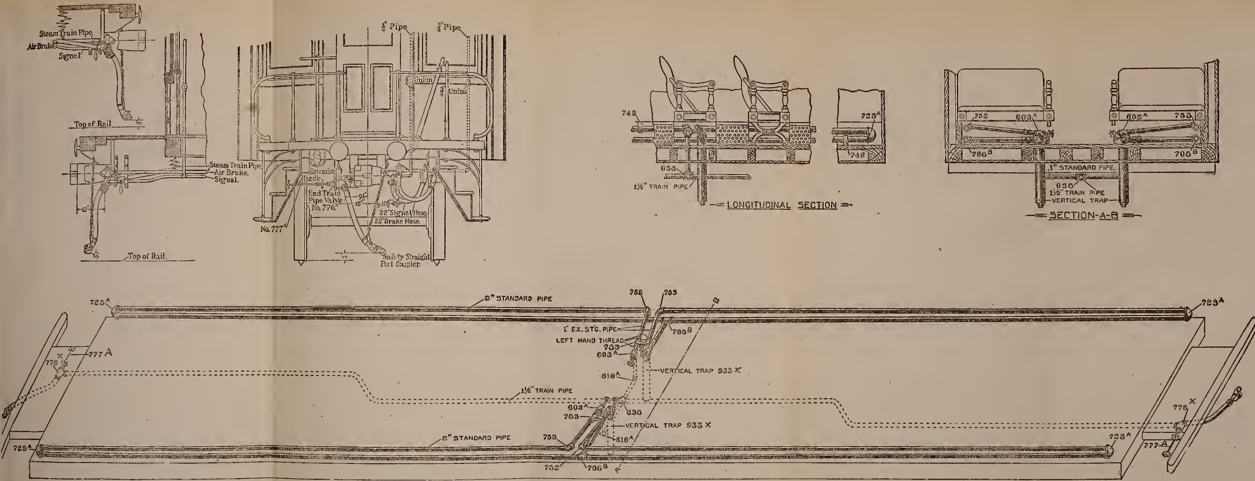
PLATE 3. Diagram illustrating design for Direct Steam Heating System.
