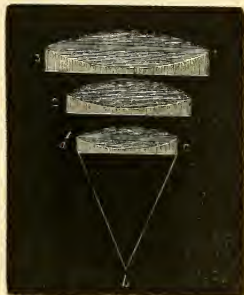
Section of an Achromatic Object-glass.
