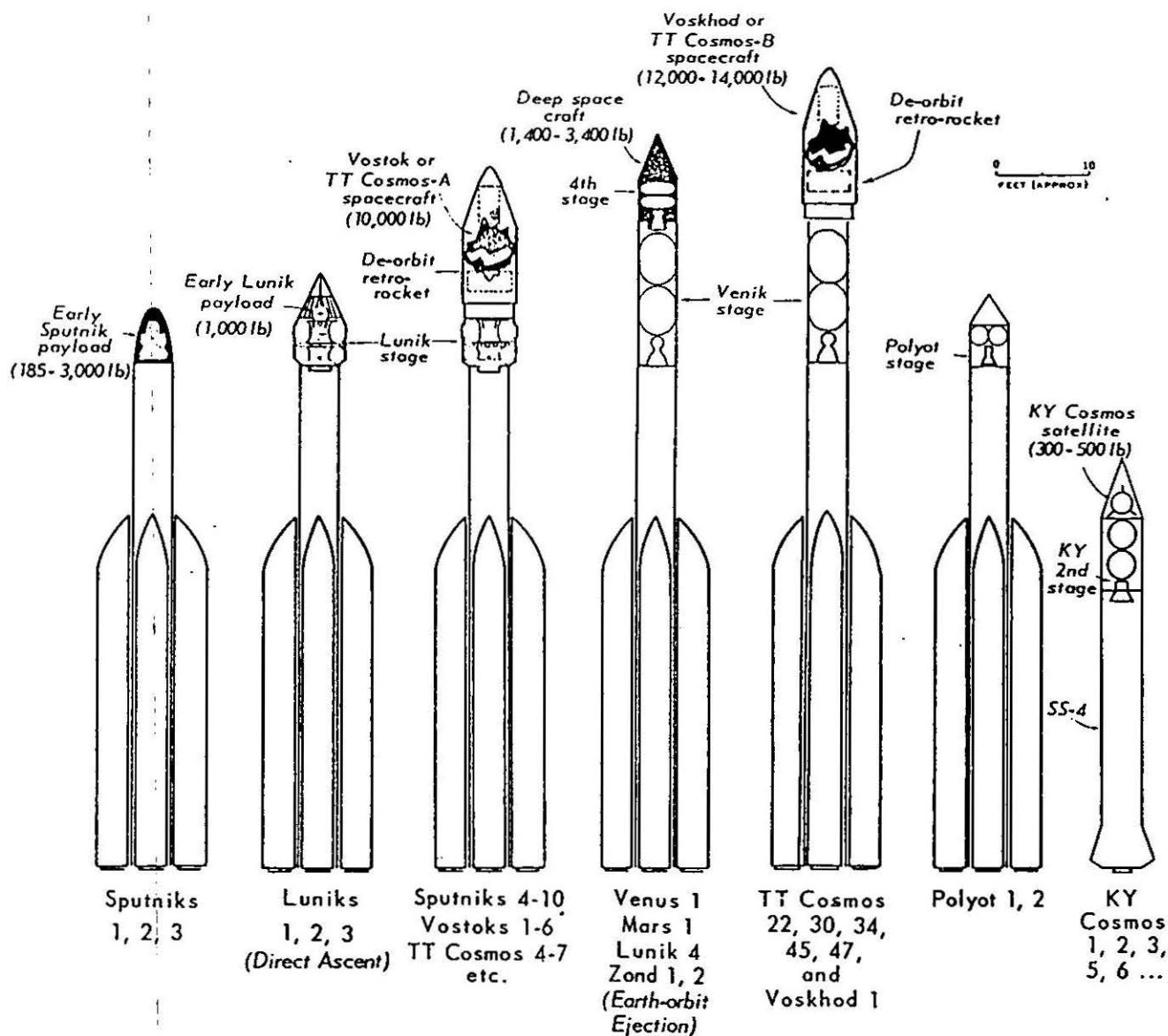
FAMILY OF SOVIET SPACE VEHICLES USED, 1957 - 1964
