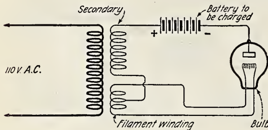
FIG. 14 A schematic diagram of a gas-filled charger
