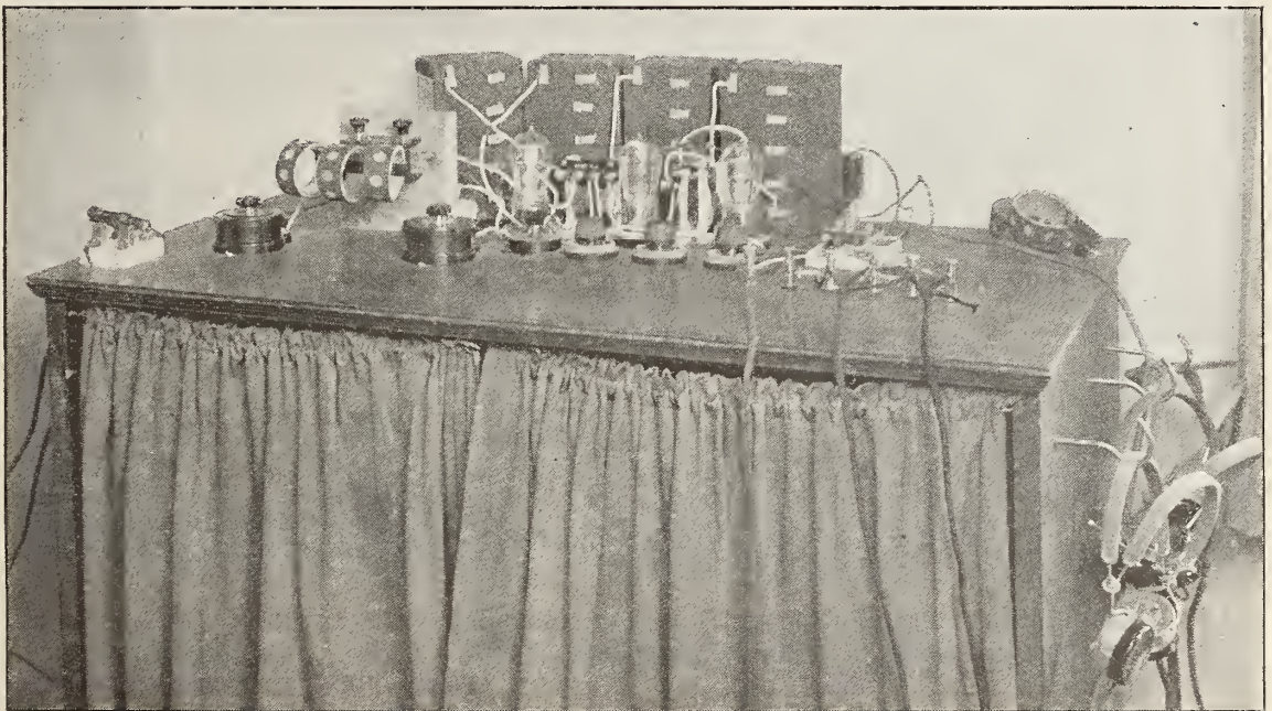
A receiving outfit of which the parts are screwed to a table top, and reduced to simple form. At the extreme left is the battery switch; then come the duo-lateral coils, the primary and secondary condensers, and the detector and amplifier bulbs with their accessories. The six binding posts on the right are so arranged that three head sets may be connected at one time. Behind them is a double-throw switch for cutting in the loud speaker
