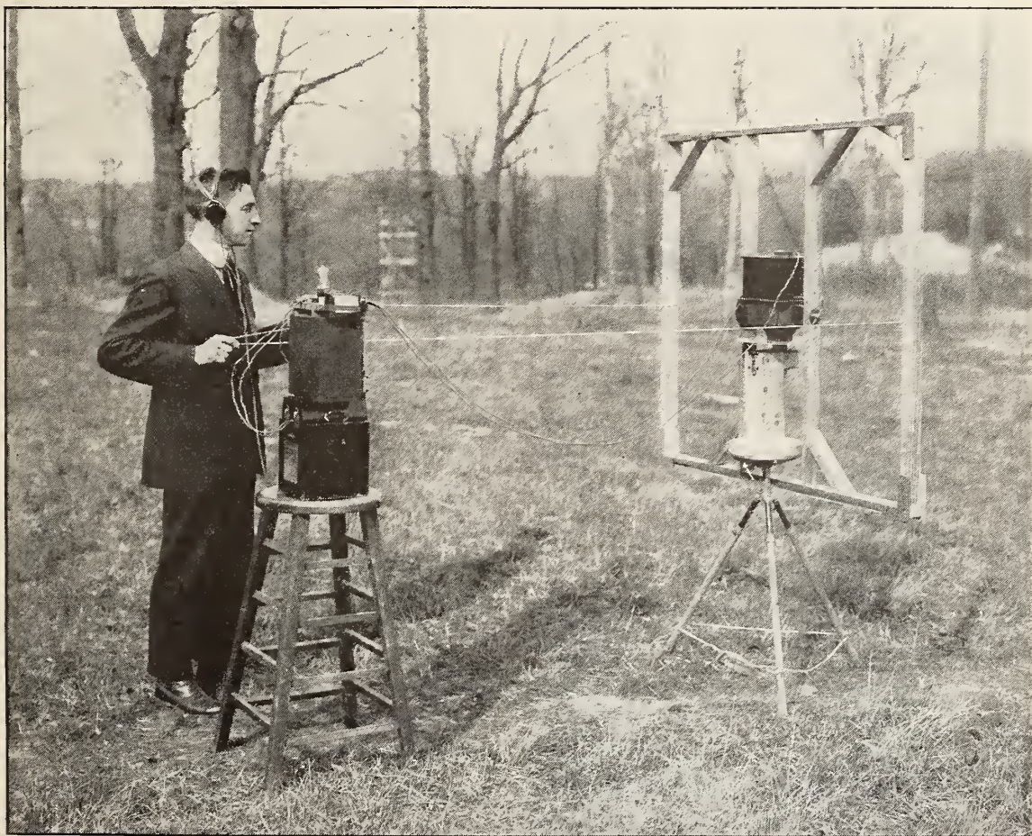
Radio direction finder in use in obtaining exact position of passing radio waves. The observer turns the frame by means of cords in order to be sure that his body has no effect on the direction of the waves. The detector and batteries are seen on the stool near the operator
