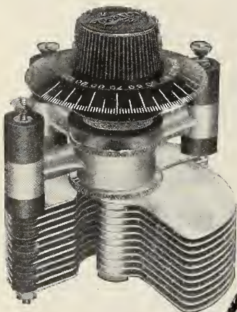
COTOCO VARIABLE AIR CONDENSER
