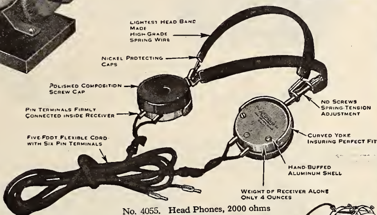
No. 4055. Head Phones, 2000 ohms
