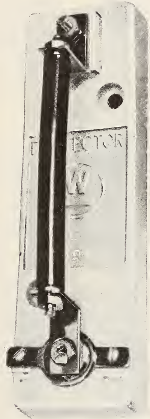
Fig. 6. A popular type of lightning arrester fitted with a fuse to protect the antenna in the event of its coming in contact with high voltage power lines
