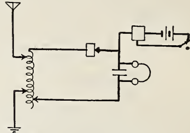
Fig. 4. Crystal receiver circuit showing test buzzer connections
