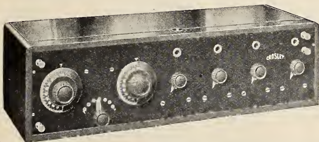
CROSLEY RECEIVER MODEL X. Is the same as MODEL VI with two stages of Audio Frequency Amplification added. In placing this receiver on the market we are offering you a unit whose range, volume and selectivity is remarkable. Nothing can compare with it at twice the price. Developed in the CROSLEY laboratories, this unit is absolutely the last word in long range Radio Receiving Apparatus. Used with head phones and loud speaker it will bring in distant stations all over the house. Price without phones, batteries or tubes, $55.00
