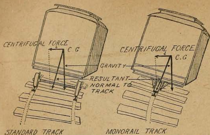
Courtesy of the "Scientific American." OLD AND NEW METHOD OF ROUNDING CURVES.
