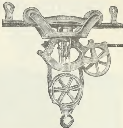
NO. 1—LOUDEN SENIOR HAY CARRIER
