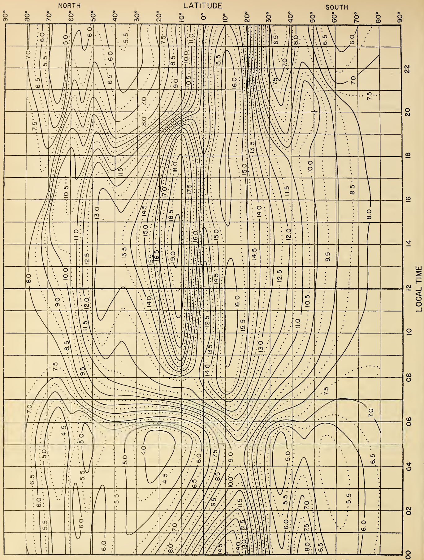
Fig. 7. F_2 ZERO-MUF, IN Mc, I ZONE, PREDICTED FOR OCTOBER 1947
