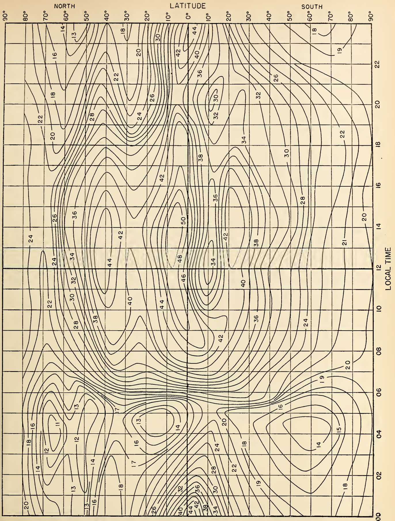
Fig. 6. F 2 4000-MUF, IN Mc, W ZONE, PREDICTED FOR OCTOBER 1947
