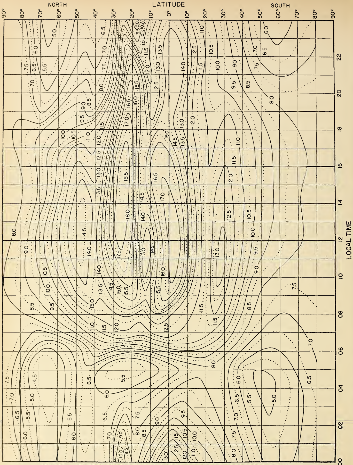
Fig. 9. F_2 ZERO-MUF, IN Mc, E ZONE, PREDICTED FOR OCTOBER 1947
