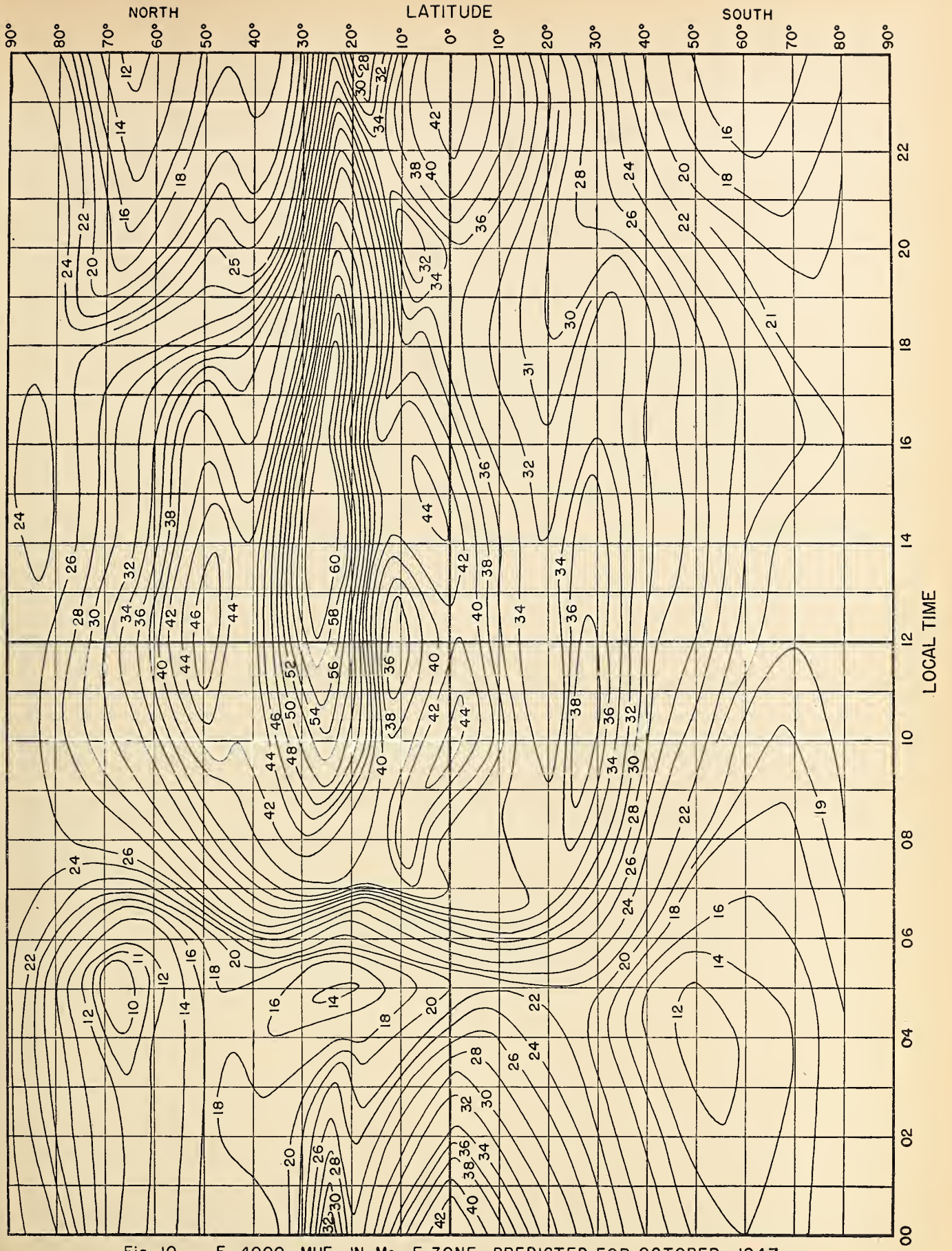
Fig. 10. F 2 4000-MUF, IN Mc, E ZONE, PREDICTED FOR OCTOBER 1947
