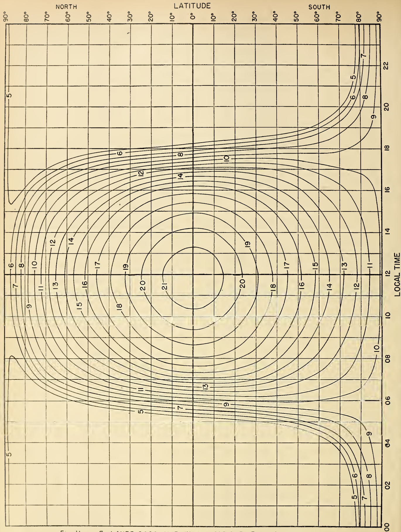
Fig. II E-LAYER 2000-MUF, IN Mc, PREDICTED FOR OCTOBER 1947
