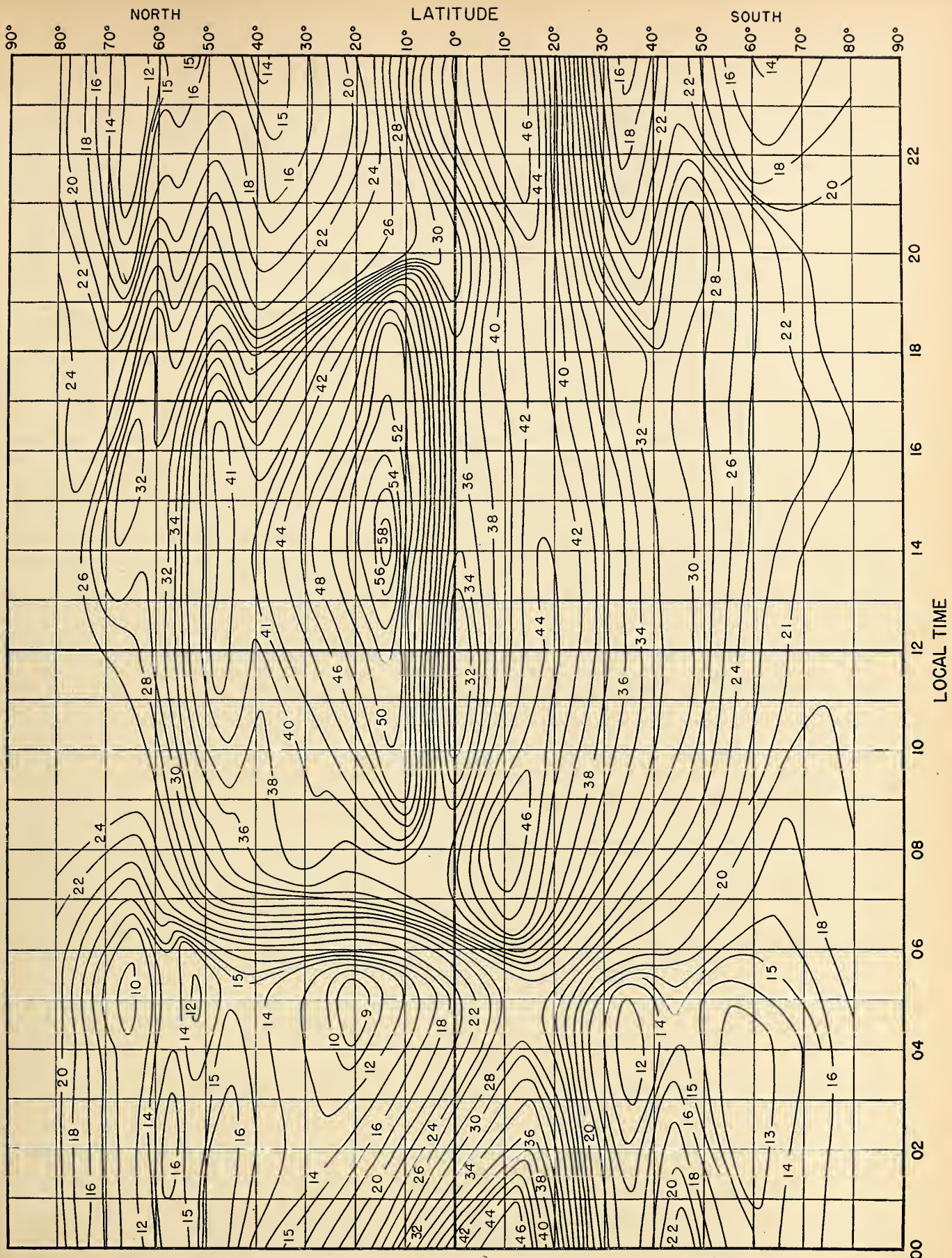
Fig. 8. F 2 4000-MUF, IN Mc, I ZONE, PREDICTED FOR OCTOBER 1947
