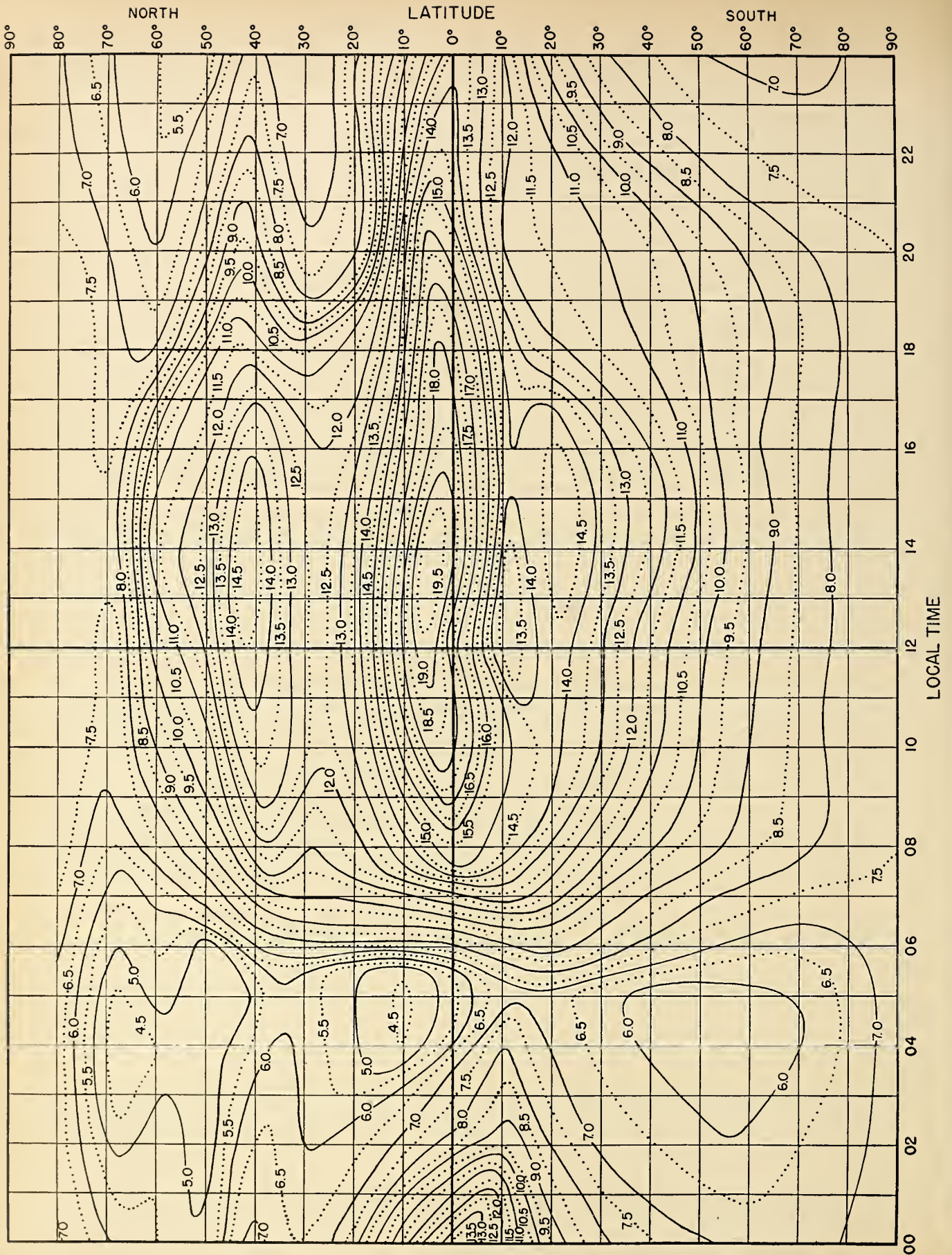
Fig. 5. F_2 ZERO-MUF, IN Mc, W ZONE, PREDICTED FOR OCTOBER 1947
