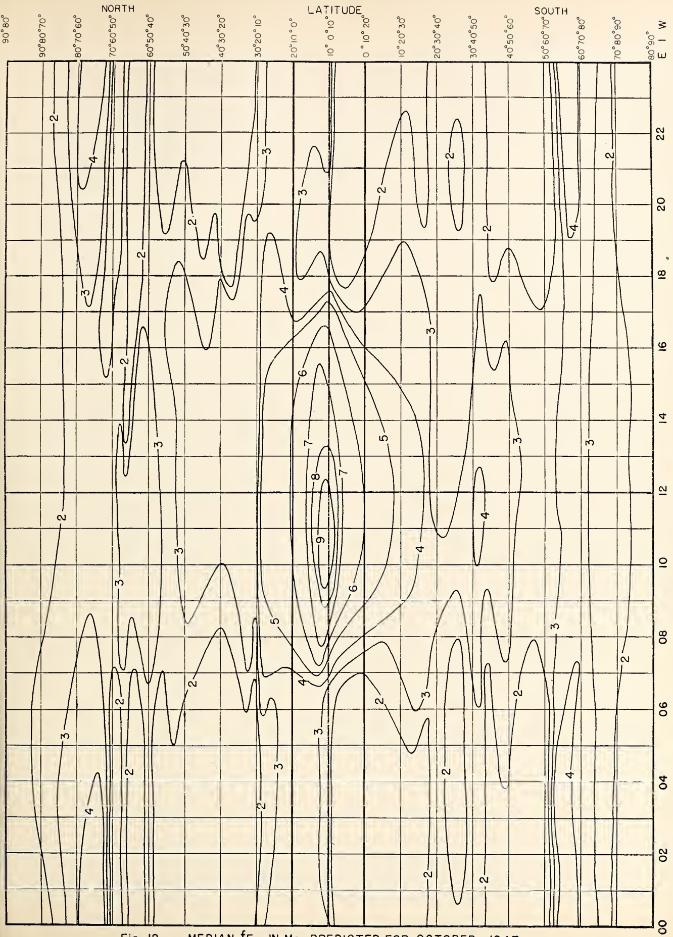
Fig. 12. MEDIAN fE_s , IN Mc, PREDICTED FOR OCTOBER 1947
