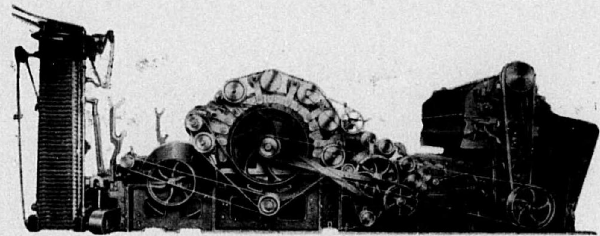
Three Card Set (Woollen)
