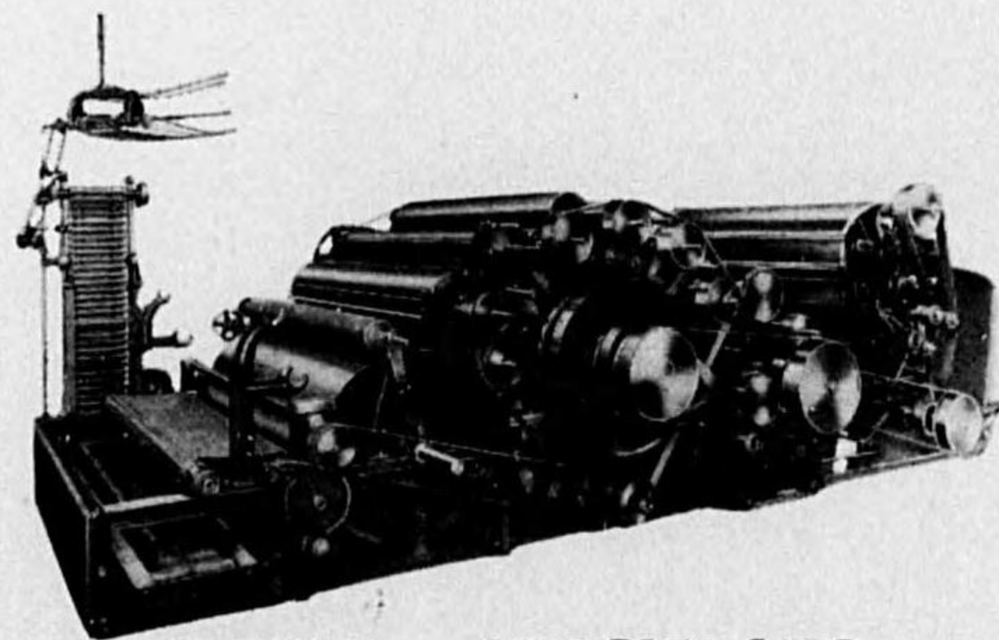
BREAKER or SCRIBBLER-CARD
