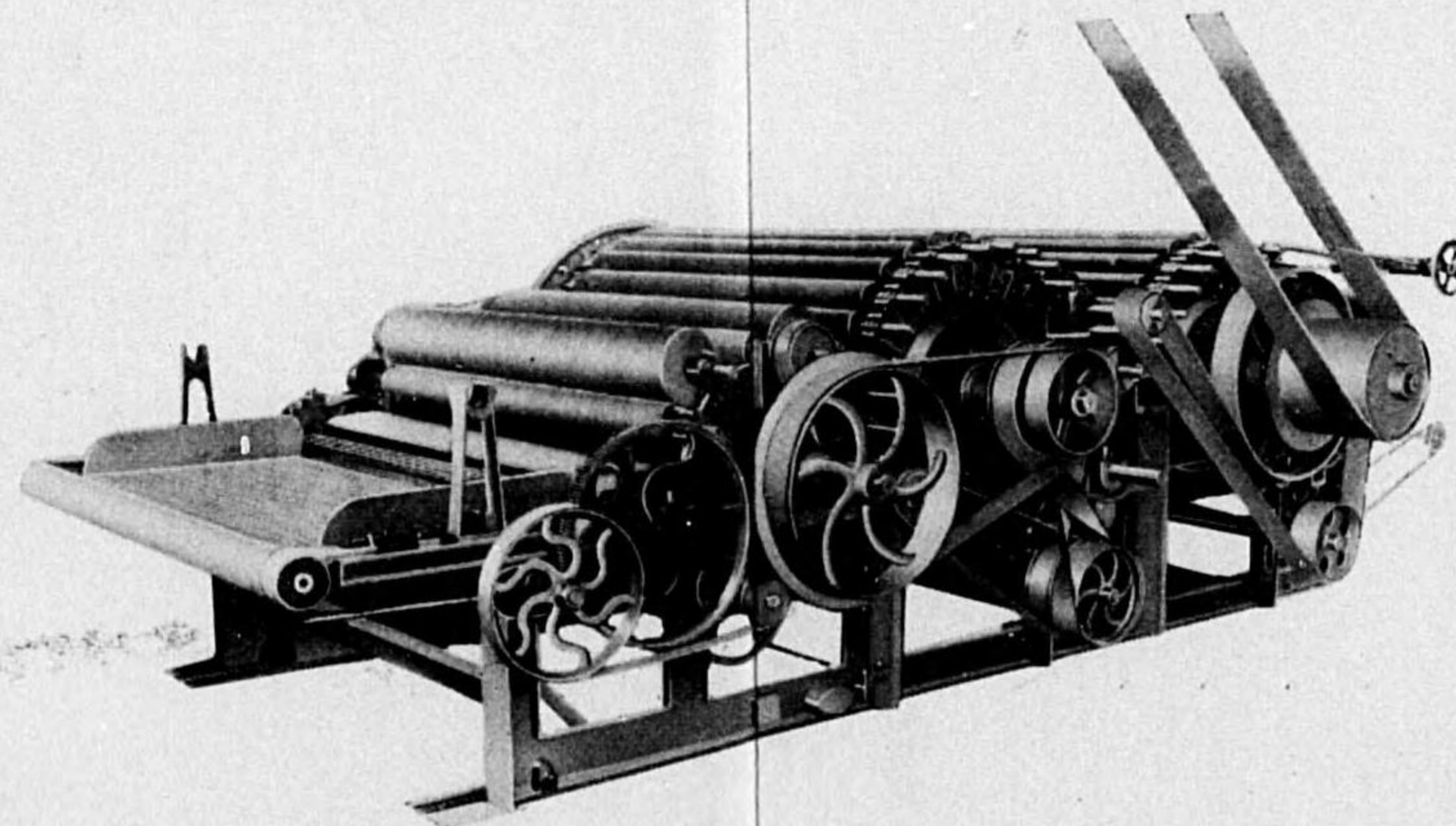
GARNETT MACHINE (With Breast Equipment)
