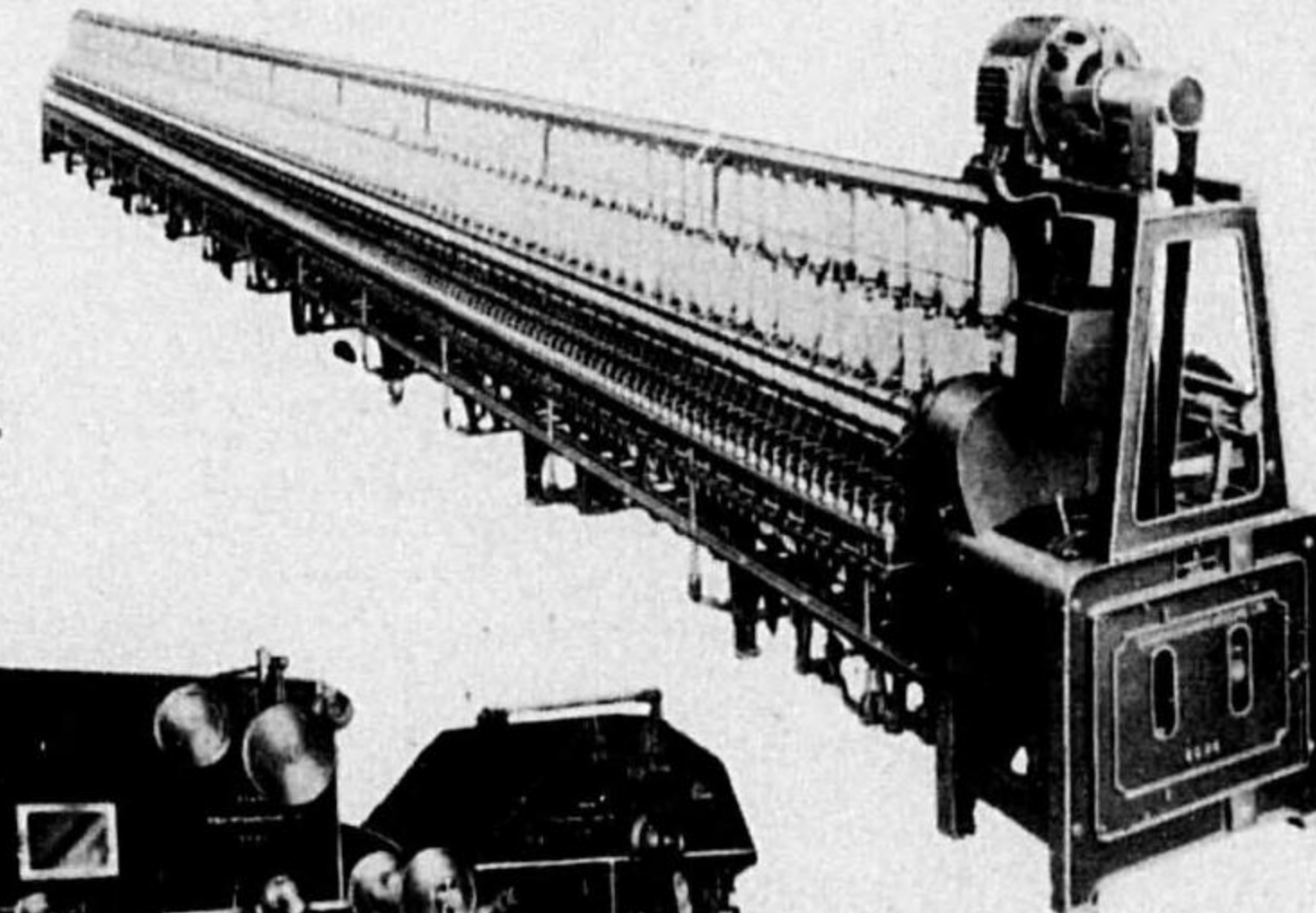
Ring Frame (Cotton) High drafting System
