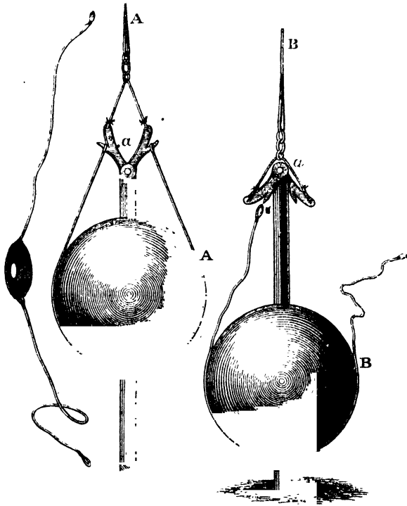
Fig. 1. Brooke's Sounding Apparatus
