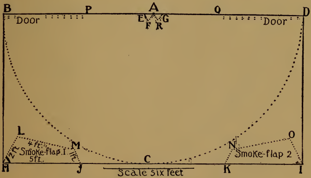
Cut VI—Pattern of 10-Foot Tepee.
