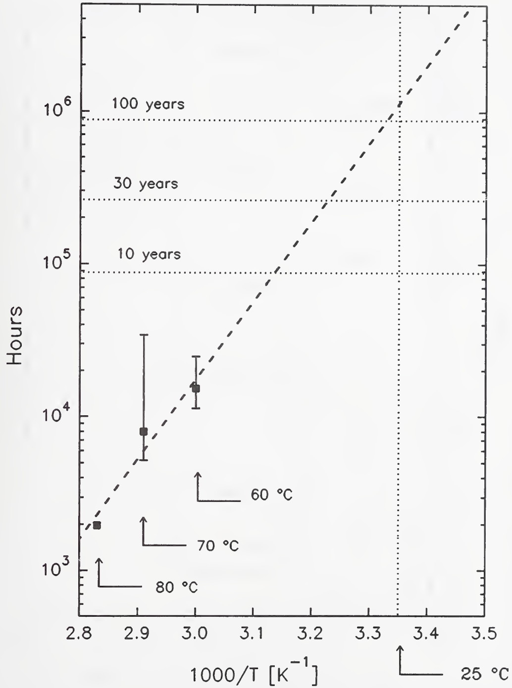
Figure 3.36. Arrhenius plot for the BER (middle area/high frequency pattern).
