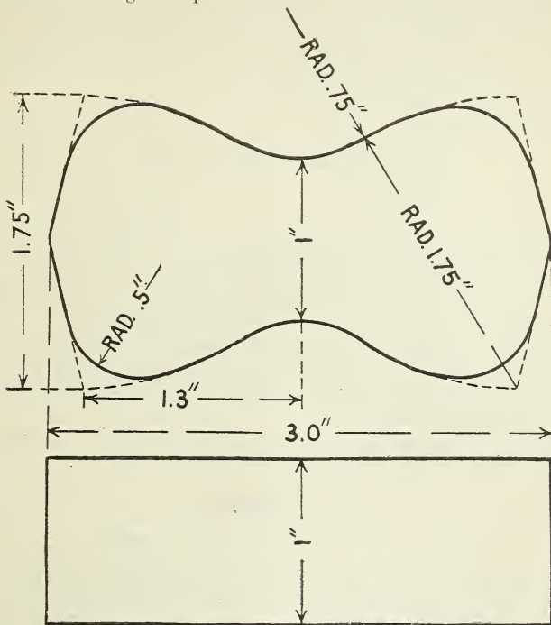
FIG. 13.—Form of briquette as recommended by the committee on uniform tests of cement of the American Society of Civil Engineers.
