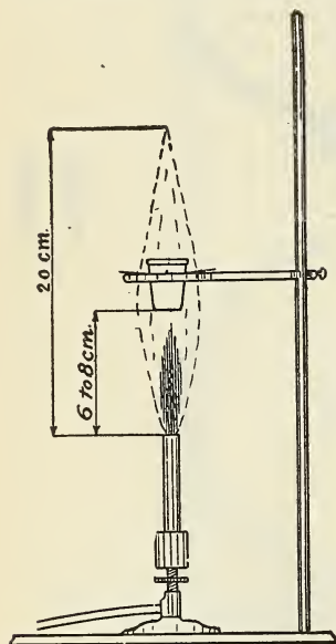
FIG. 22.—Apparatus for determining fixed carbon.
