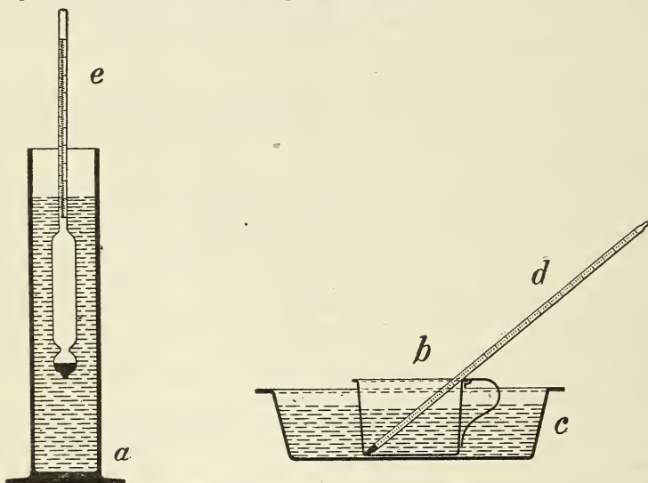
FIG. 15.—Hydrometer method of determining specific gravity.
