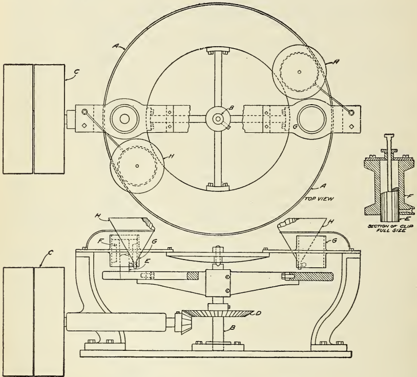
FIG. 2.—Details of Dorry hardness machine.
