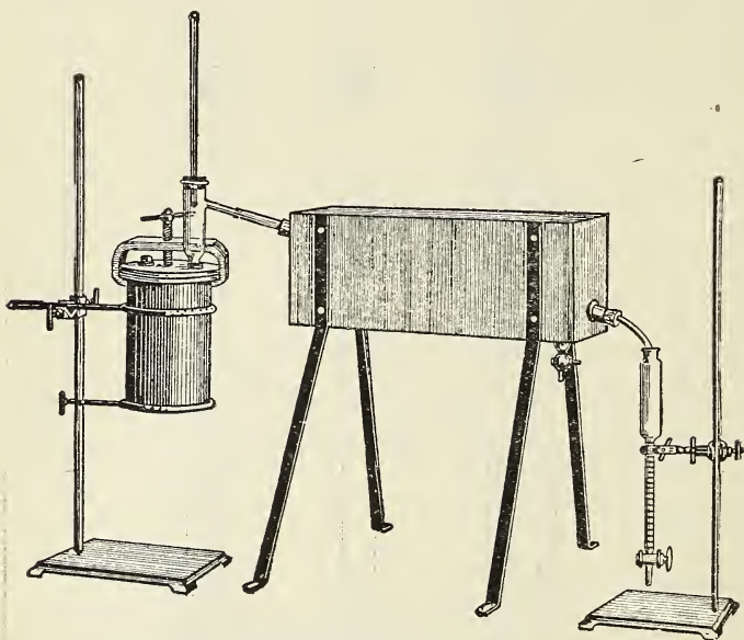
FIG. 27.—Dehydrating apparatus.
