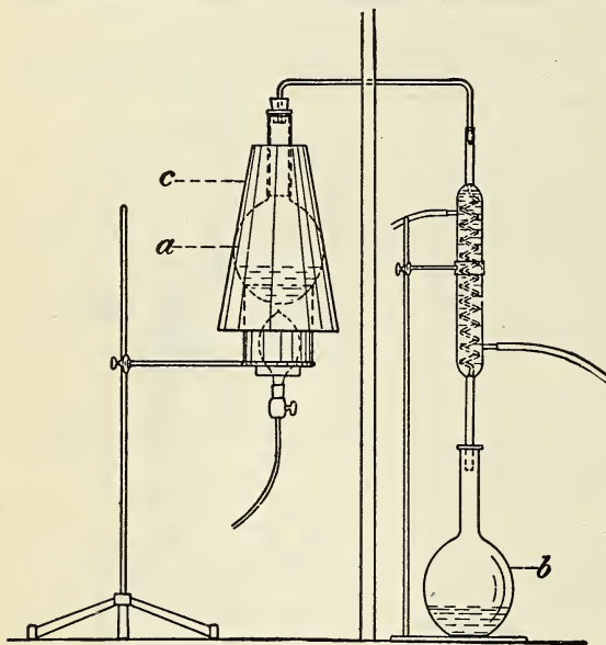
FIG. 31.—Recovery apparatus.
