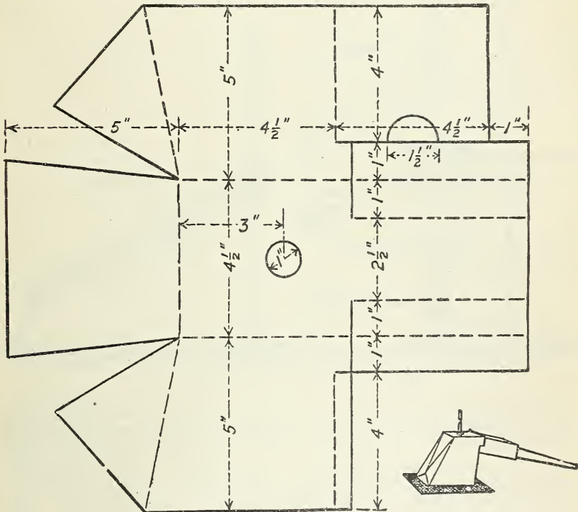
FIG. 33.—Asbestos shield.
