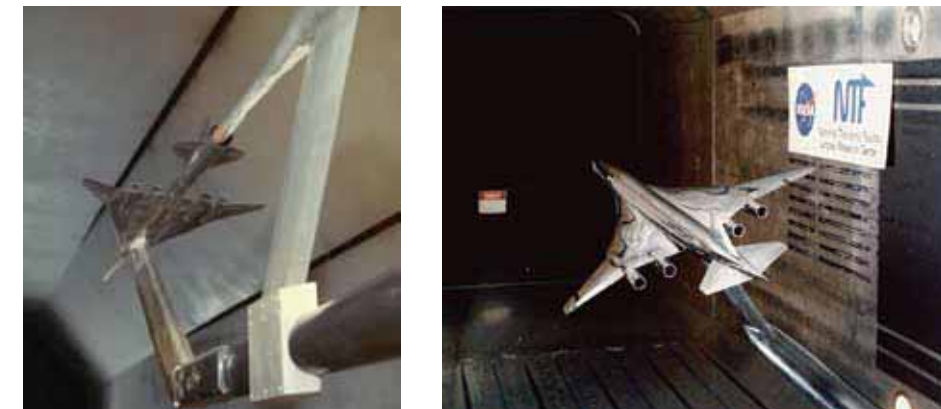
Extensive testing of the High Speed Research Reference H configuration was conducted in many Langley tunnels, including the 16-Foot Transonic Tunnel (left) and the National Transonic Facility (right).
