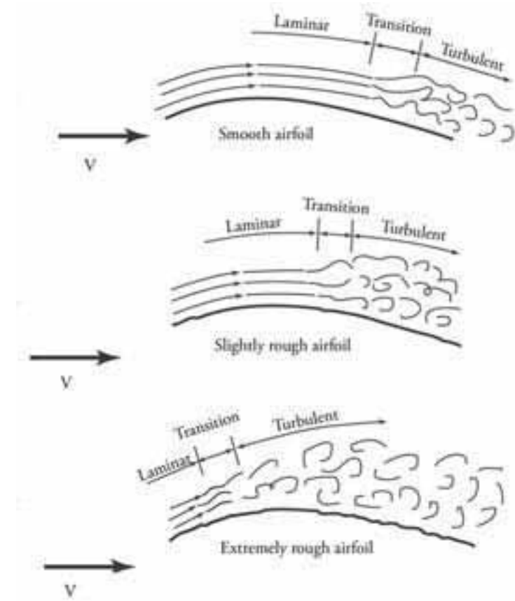
Effect of airfoil surface condition on boundary-layer flow.
