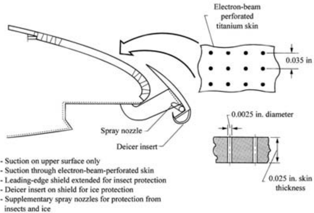
The perforated Douglas Leading Edge Flight Experiment panel.
