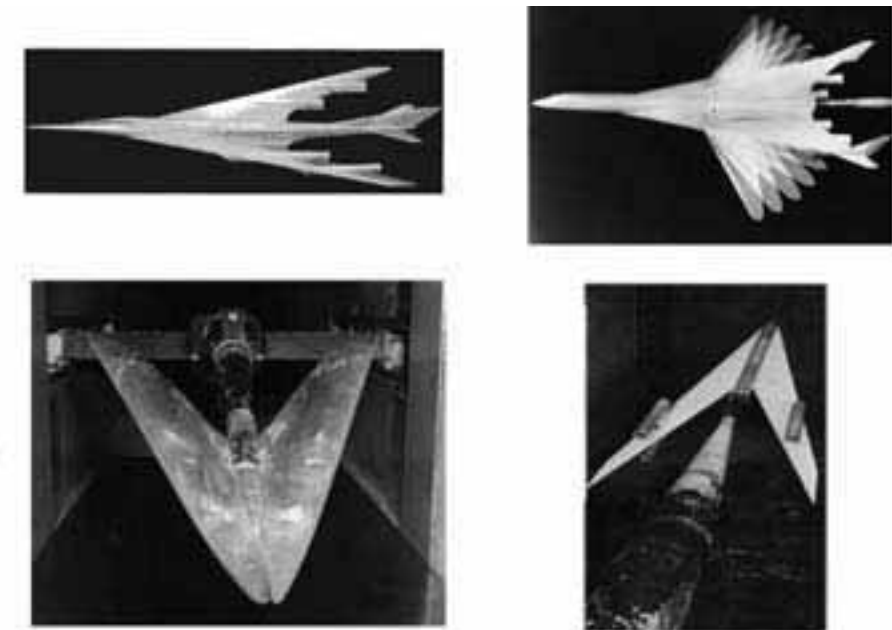
Highly swept arrow wings are nearly optimum shapes for supersonic flight.
