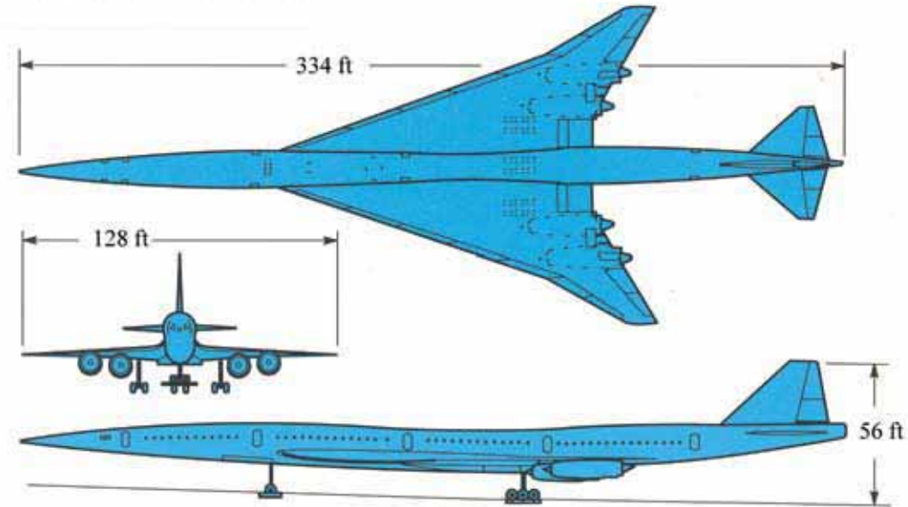
A McDonnell Douglas High-Speed Civil Transport concept during the early High Speed Research Program
