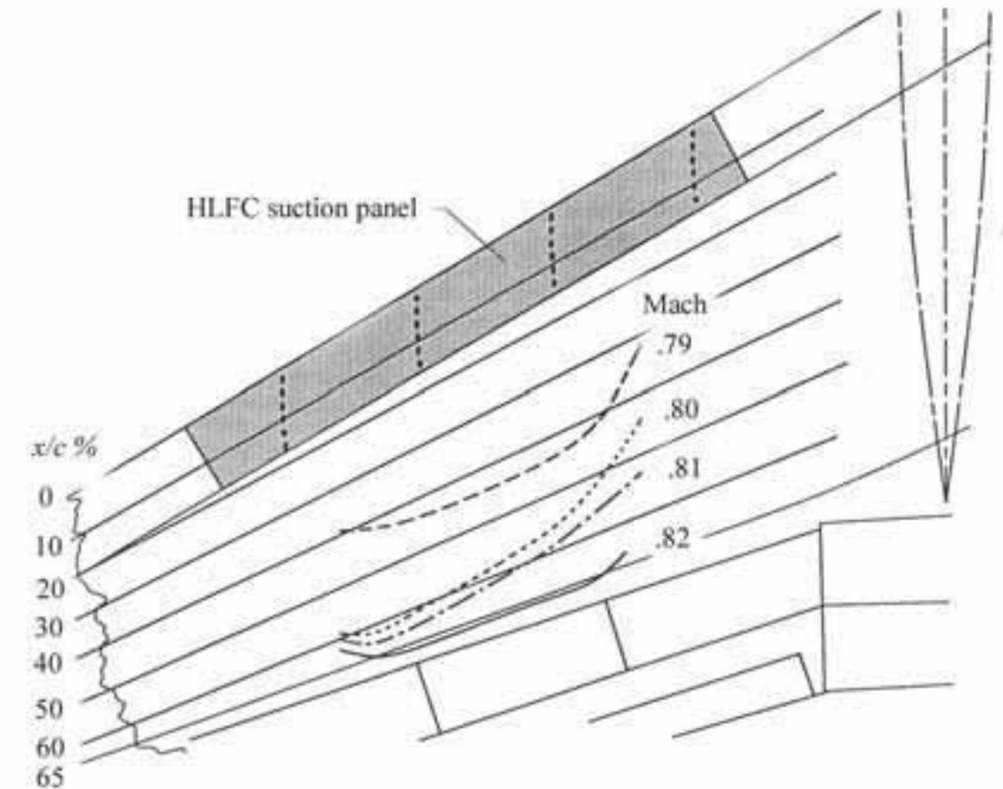
Transition contours showing the extent of laminar flow obtained on the wing upper surface of the 757 with hybrid laminar flow control.
