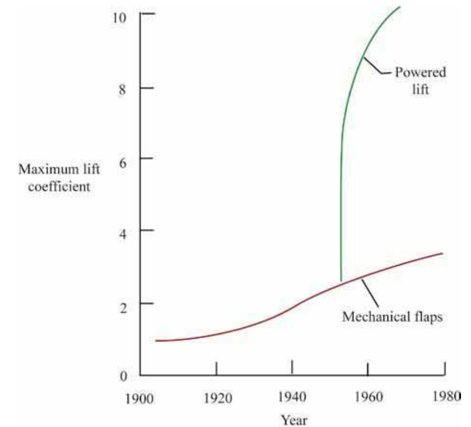
Historical development of maximum lift coefficient for aircraft.
