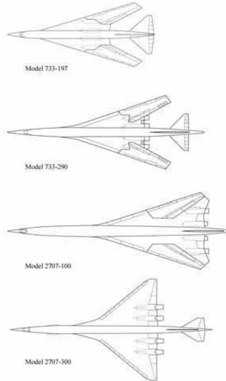
Evolution of the final Boeing Supersonic Transport configuration.
