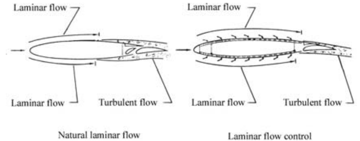
Laminar flow obtained by airfoil shaping in the natural laminar flow concept (left) and active suction flow control in the laminar flow control concept (right).
