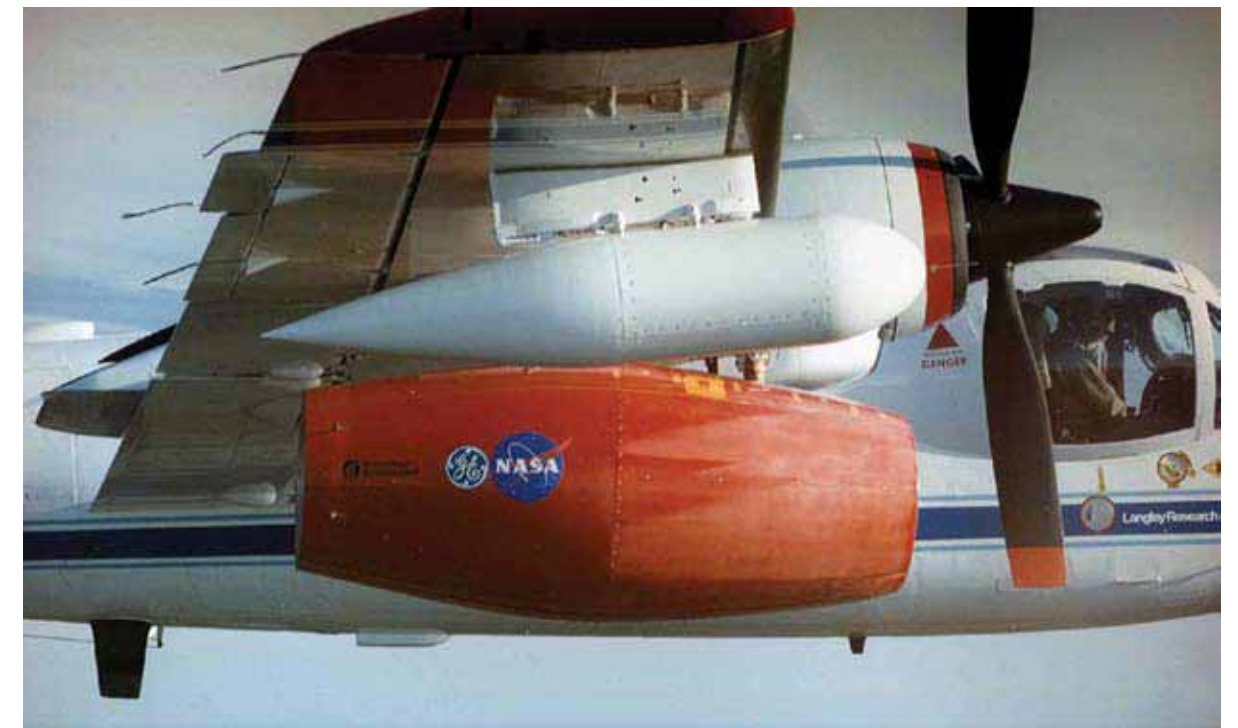
Sublimating chemicals indicate laminar flow (white area) on forward region of NLF nacelle during research flight.
