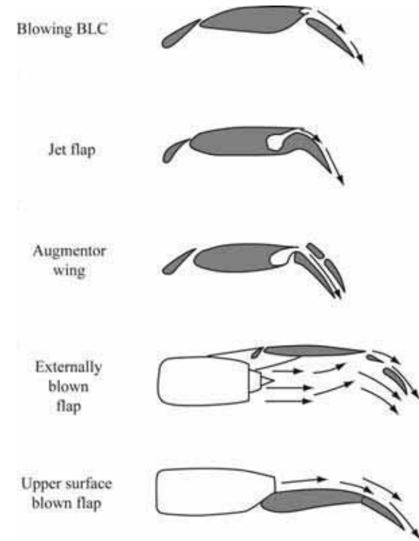
Powered-lift concepts for lift augmentation.
