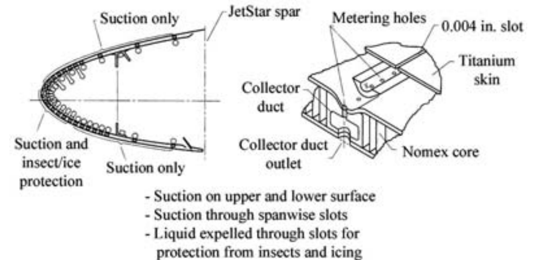
The slotted Lockheed Leading Edge Flight Experiment panel.
