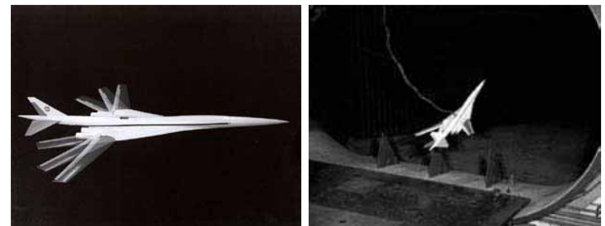
Time-lapse photography shows the variable sweep wing of early Boeing Model 733-290 Supersonic Transport design. Free-flight testing was conducted in the Langley Full-Scale Tunnel.
