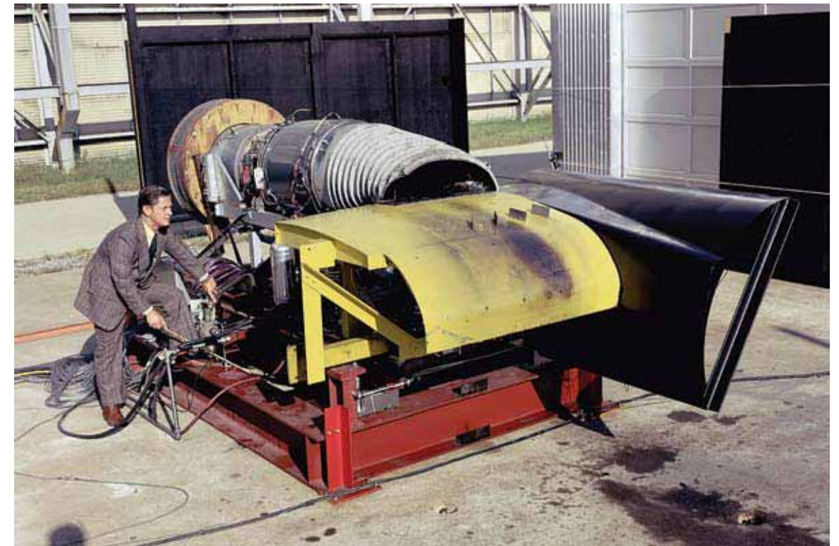
James L. Hassell inspects the 0.25-scale model of the YC-14 USB arrangement. Note vortex generators deployed on USB flap.
