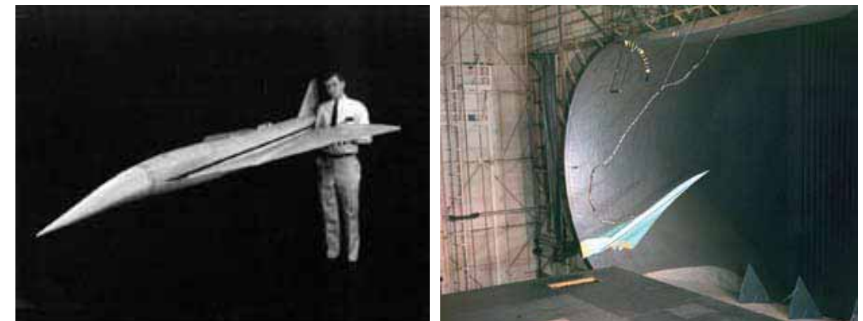
Researcher Delma C. Freeman, Jr., inspects a free-flight model of the Lockheed L-2000 Supersonic Transport design (left) used in tests in the Langley 30- by 60-Foot Full-Scale Tunnel.
