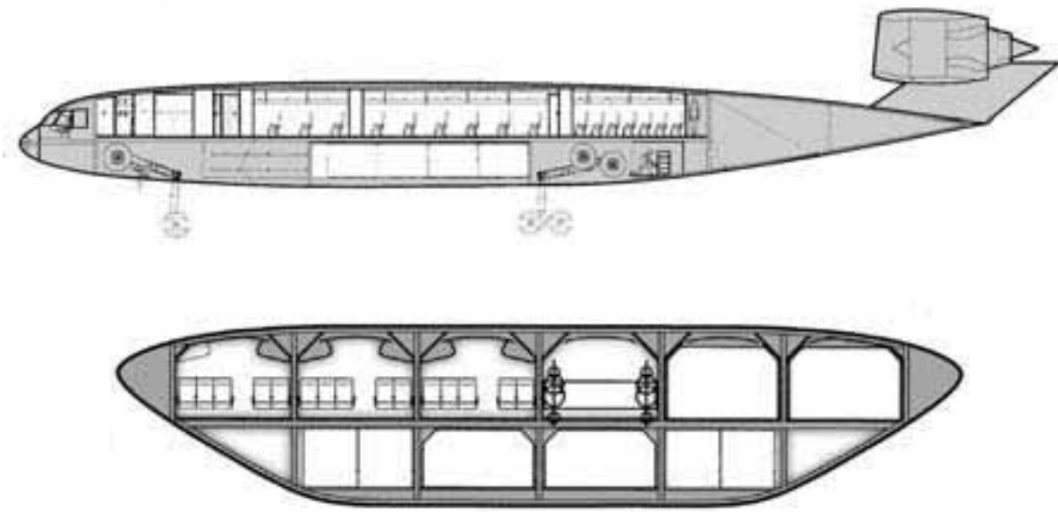
Schematic of Blended Wing Body passenger cabin showing side view (upper sketch) and front view (lower sketch) of layout.
