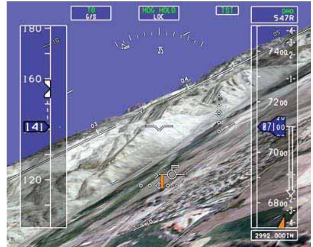
Details of the synthetic vision system display used in the demonstration flights.
