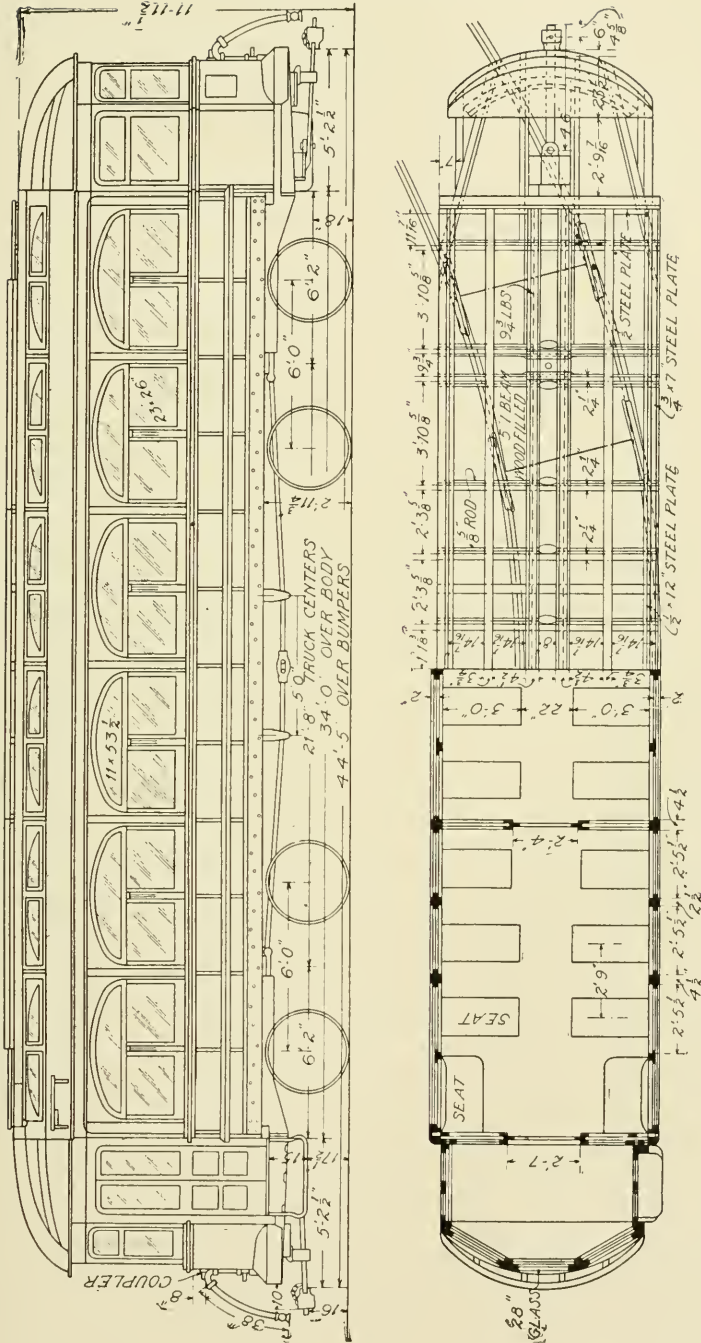
Fig. 2. Plan and Elevation of Interurban Car
