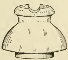
HEIGHT 3\frac{1}{2} " TESTED AT 40,000V.
