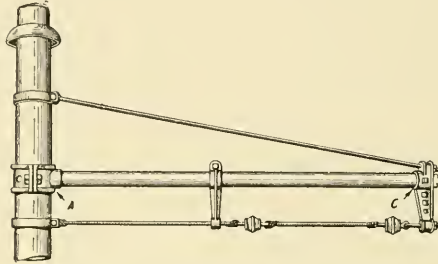
Fig. 196. Bracket Used on Metal Poles
