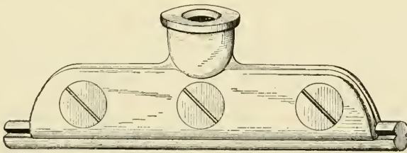
Fig. 186. Clamp Used with Groove Trolley Wire
