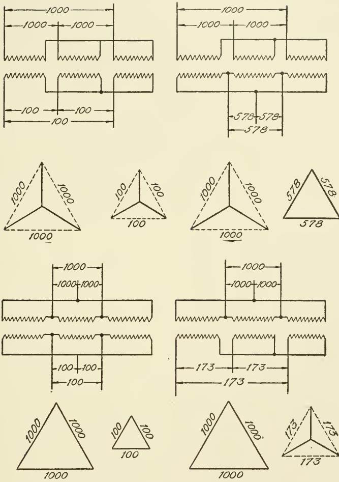
Fig. 31. Vector Diagrams of Step-down Transformers by \Upsilon and \Delta Systems—Primary Voltage 1,000
