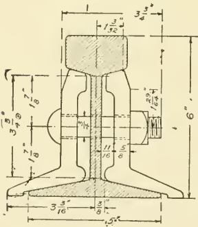
Fig. 223. Shanghai T Rail
