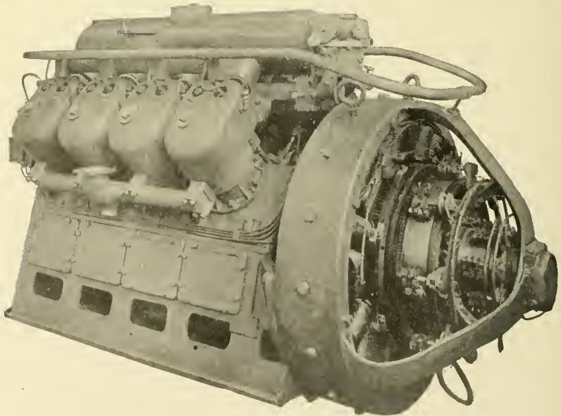
Fig. 14. Gas Engine and Generator of Gas-Electric Car.
