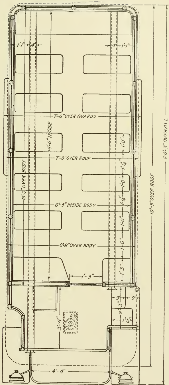
Fig. 18. Diagram Showing Interior Arrangement of Leeds Trackless Trolley Cars
