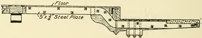
Fig. 7. Platform Knee
