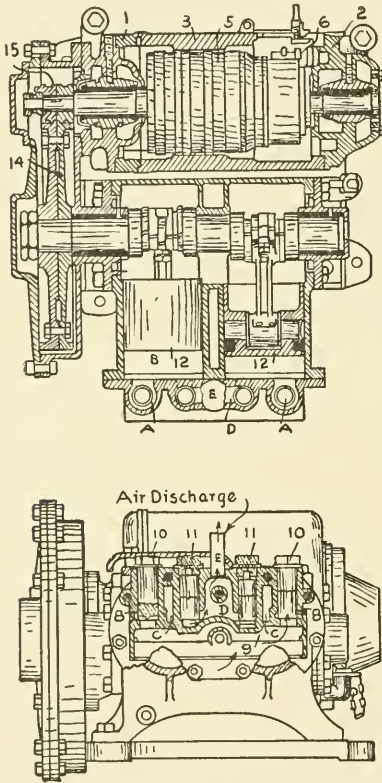
Fig. S7. Section of Motor and Pump in Motor Driven from Pressure
