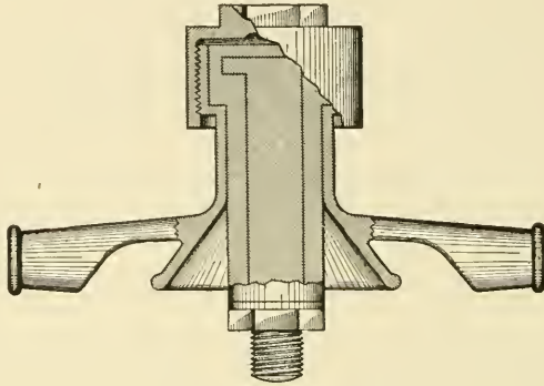
Fig. 183. Section of a Hanger
