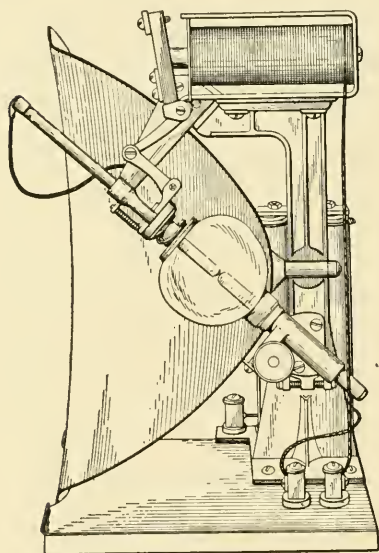
Fig. 116. Section of Arc Headlight
