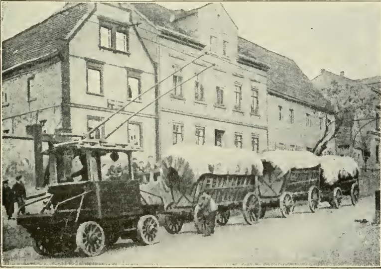
Fig. 4. Industrial Trackless Trolley Line at Wurzen, Germany Courtesy of Horseless Age
