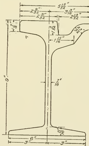
Fig. 225. "Trilby" or Grooved Rail
