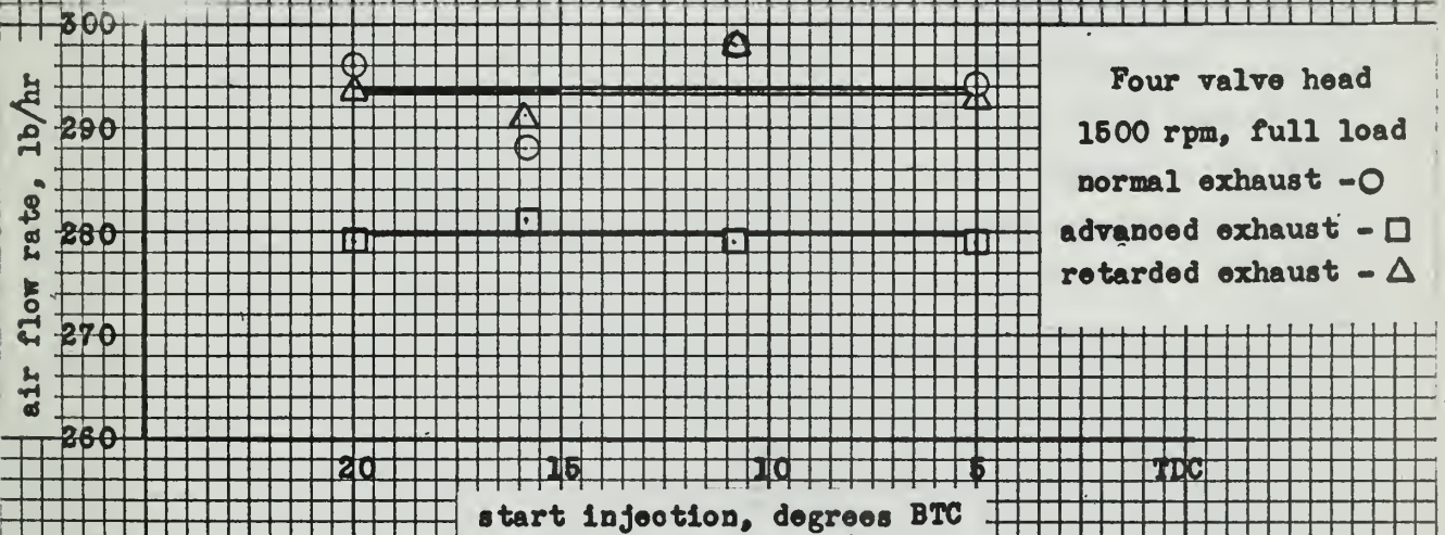
Fig. 34. Air flow rate versus injection point for various exhaust timings.
