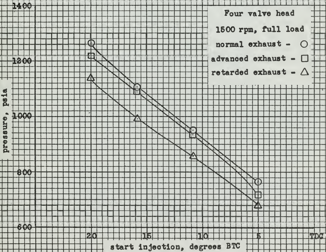
Fig. 35. Peak firing pressures versus injection point for various exhaust timings.
