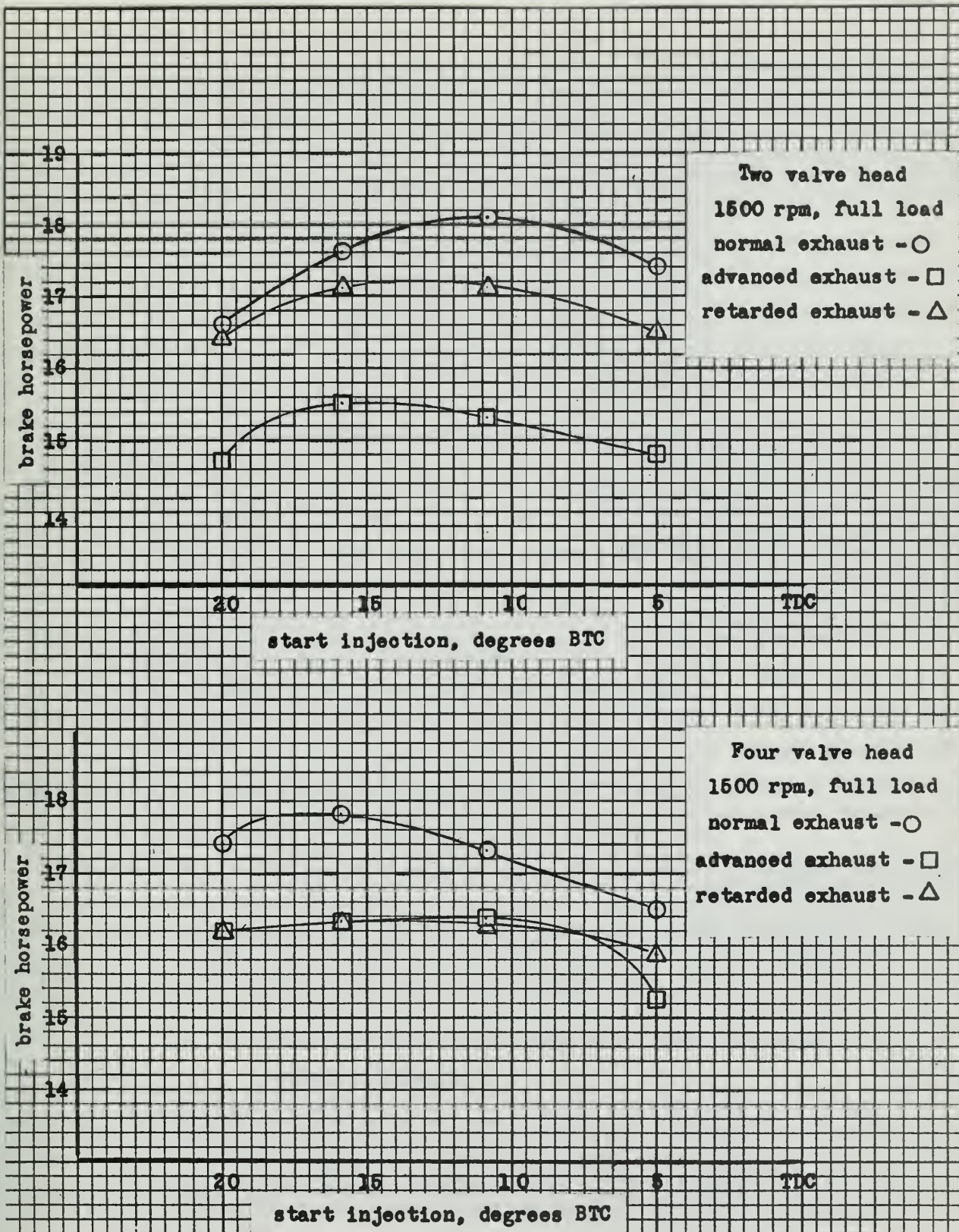
Fig. 33. Brake horsepower versus injection point for various exhaust timings.
