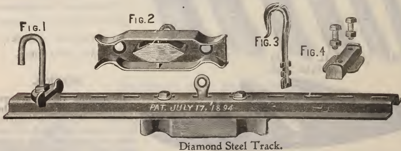
Diamond Steel Track.
