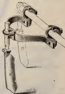
Double Row Extension. Fig. 147
