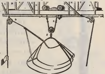
GRAPPLING HAY FORK & RAILWAY HAY CONVEYOR
