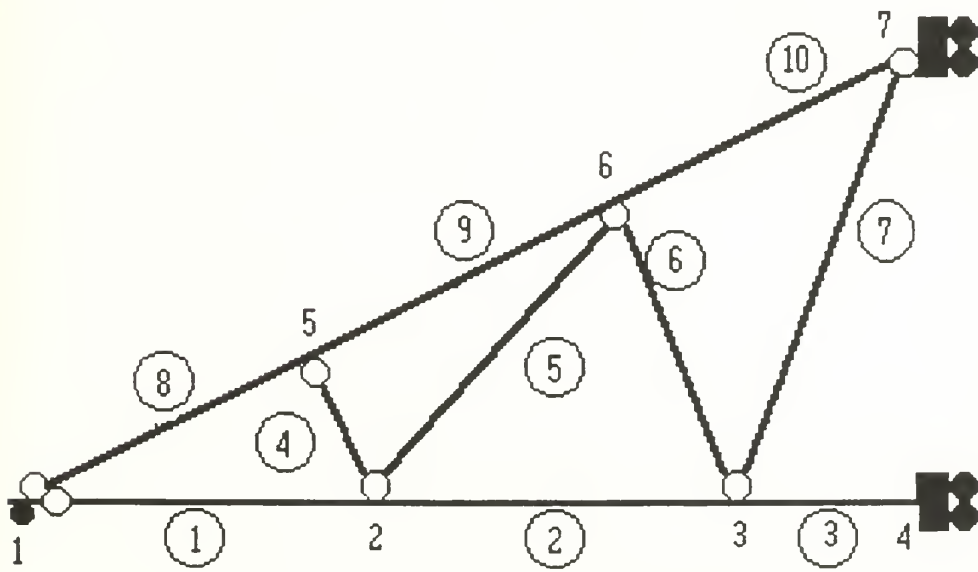
Fig. 3.5 TRUSS 5
