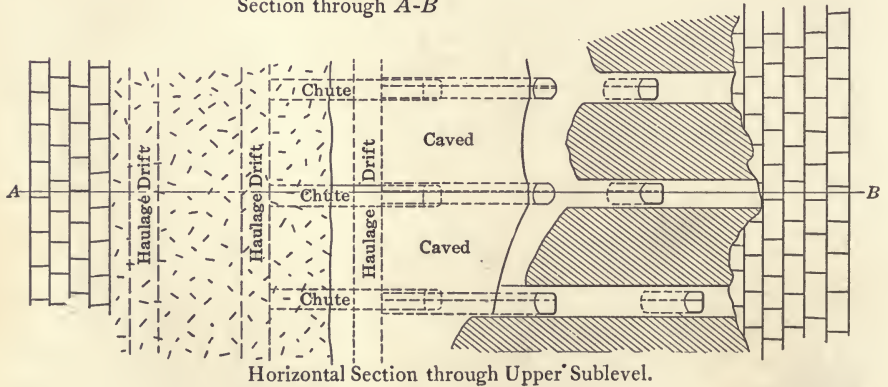
FIG. 106.—Stoping at Mercur mine.
