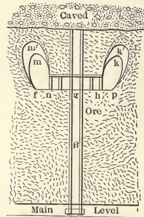
Fig. 92.—Enlarging stope at Pioneer mine.
