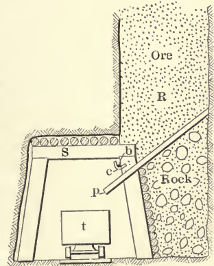
FIG. 37.—Chute for milling system.
