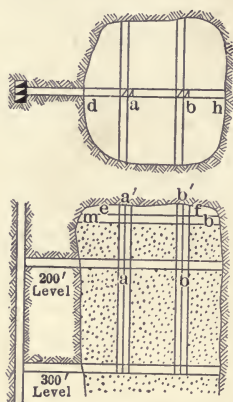
FIG. 101.—Stoping at Old Jordan mine.
