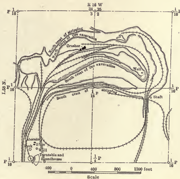
FIG. 28.—Biwabik open pit.
