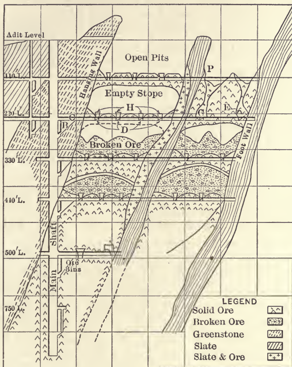
FIG. 38.—Alaska Treadwell mine, cross section.
