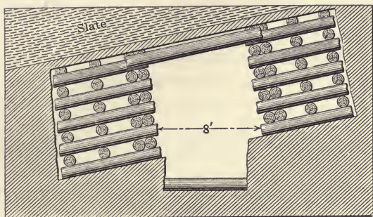
FIG. 126.—Cross section of road, Drummond colliery.
