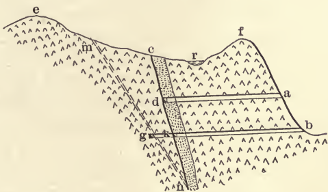
FIG. 21.—Drainage in massive rock.
