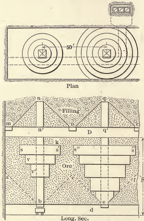
FIG. 47.—Stoping at Section—21 mine.
