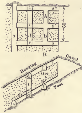
FIG. 98.—Stopping at Commercial mine.
