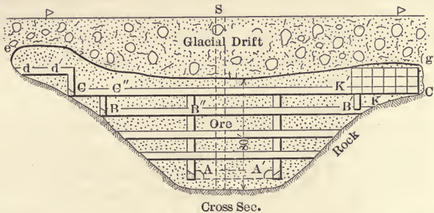
FIG. 105.—Cross-section of stope, Glenn mine.
