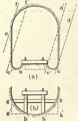
FIG. 24.—Adit sections.
