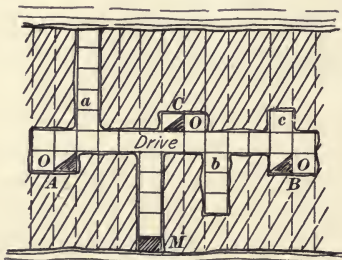
FIG. 73.—Plan of Gross-cut slope, Proprietary mine.
