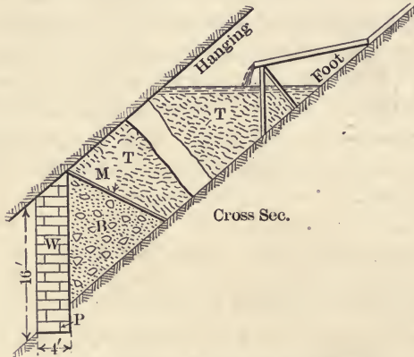
FIG. 145.—Dam for holding slush, Transvaal.
