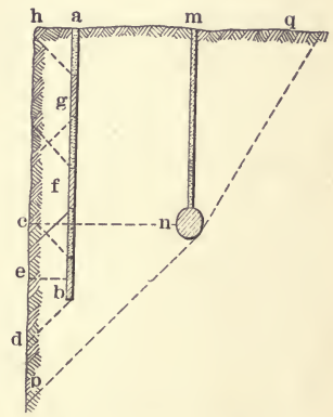
FIG. 9.—Holes for high bench.
