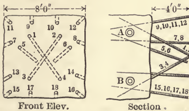
FIG. 6.—Holes for Leyner tunnel cut.
