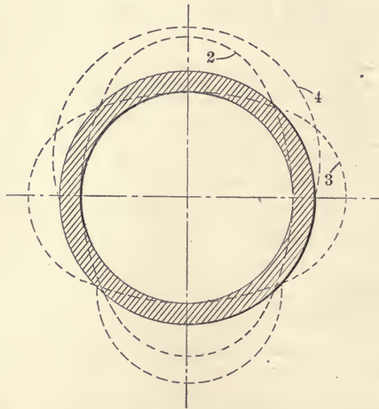
FIG. 17.—Tunnel sections.
