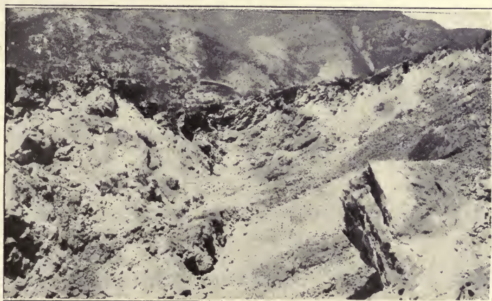
FIG. 93.—Caved surface, Utah Copper mine.
