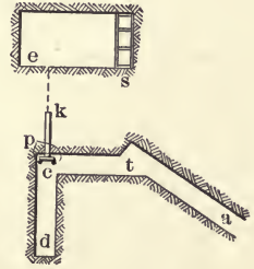
FIG. 22.—Tapping sump at Iron Mt. Mine, Montana.
