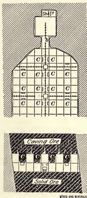
FIG. 95.—Stoping at Mowry mine.
