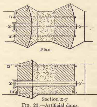
FIG. 23.—Artificial dams.
