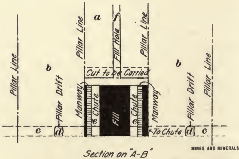
FIG. 64.—Stoping by submethod "A", Los Pilares mine.
