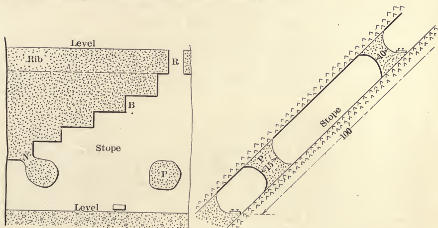
FIG. 49.—Stoping at Wolverine mine.
