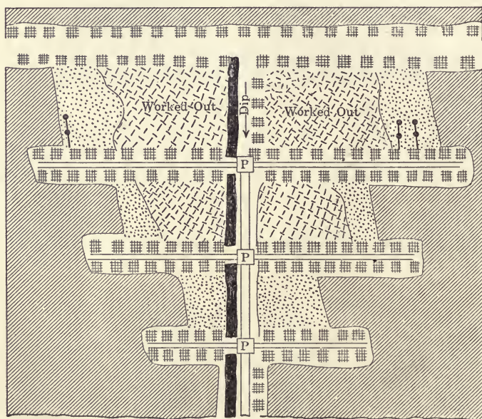
FIG. 128.—Plan of jig road, Drummond colliery.
