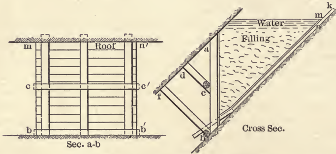
FIG. 144.—Dam for holding slush, Eastern Pa.
