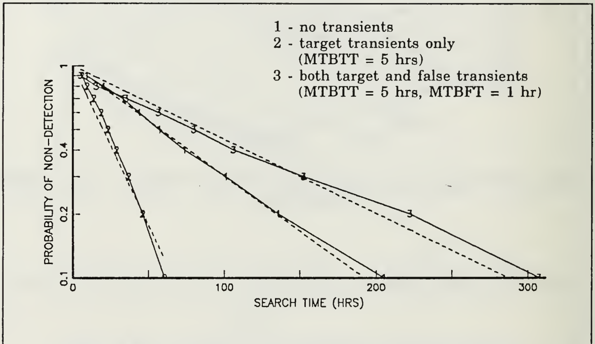
Figure 5.17. Excursion 2 - Probability of Non-Detection.
