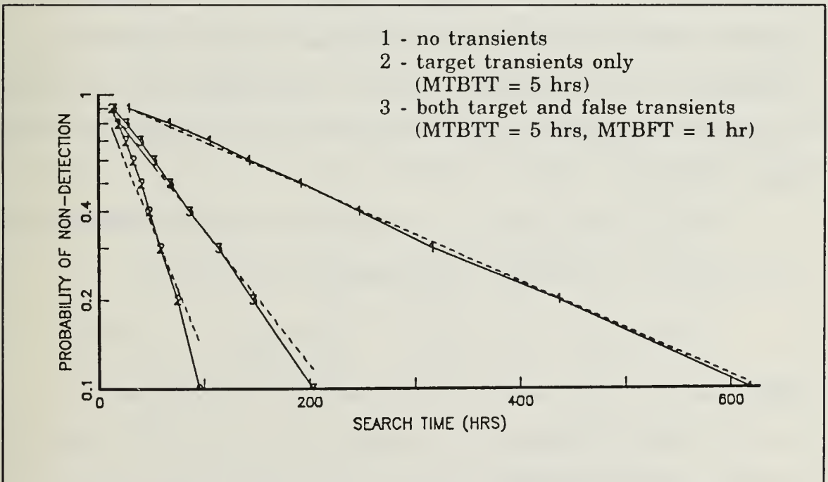
Figure 5.12. Test Case 4 - Probability of Non-Detection.
