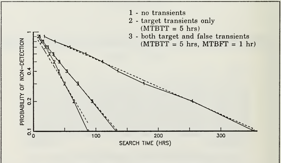
Figure 5.10. Test Case 2 - Probability of Non-Detection.
