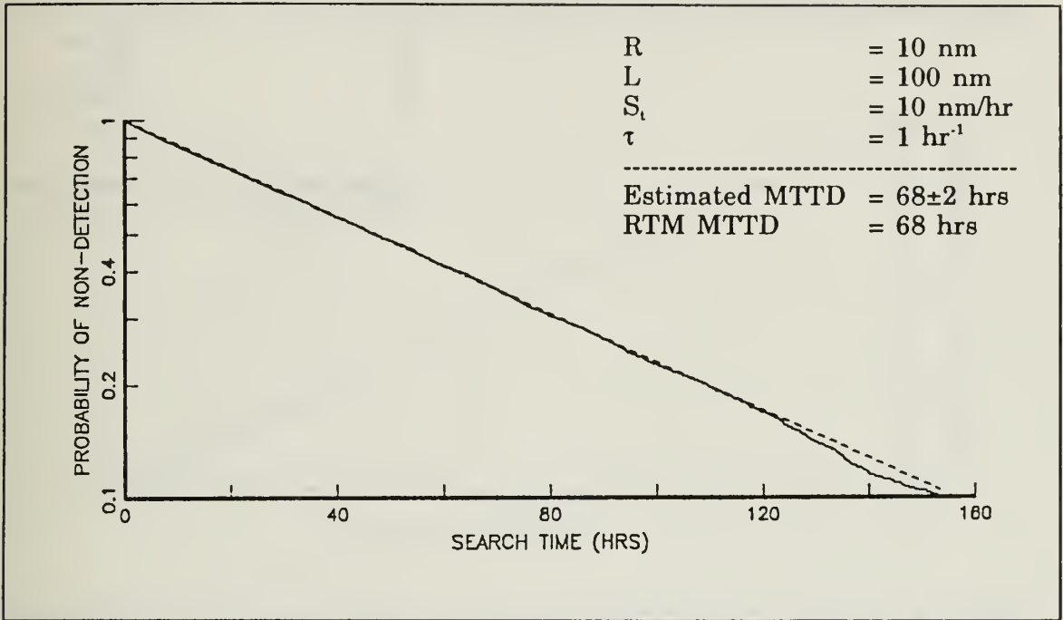
Figure 4.5. Random Tour Model Approximation Case 1 - Probability of Non-Detection.
