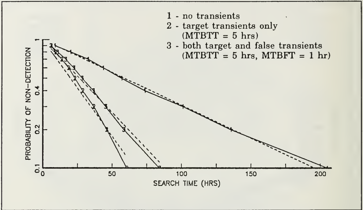
Figure 5.9. Test Case 1 - Probability of Non-Detection.
