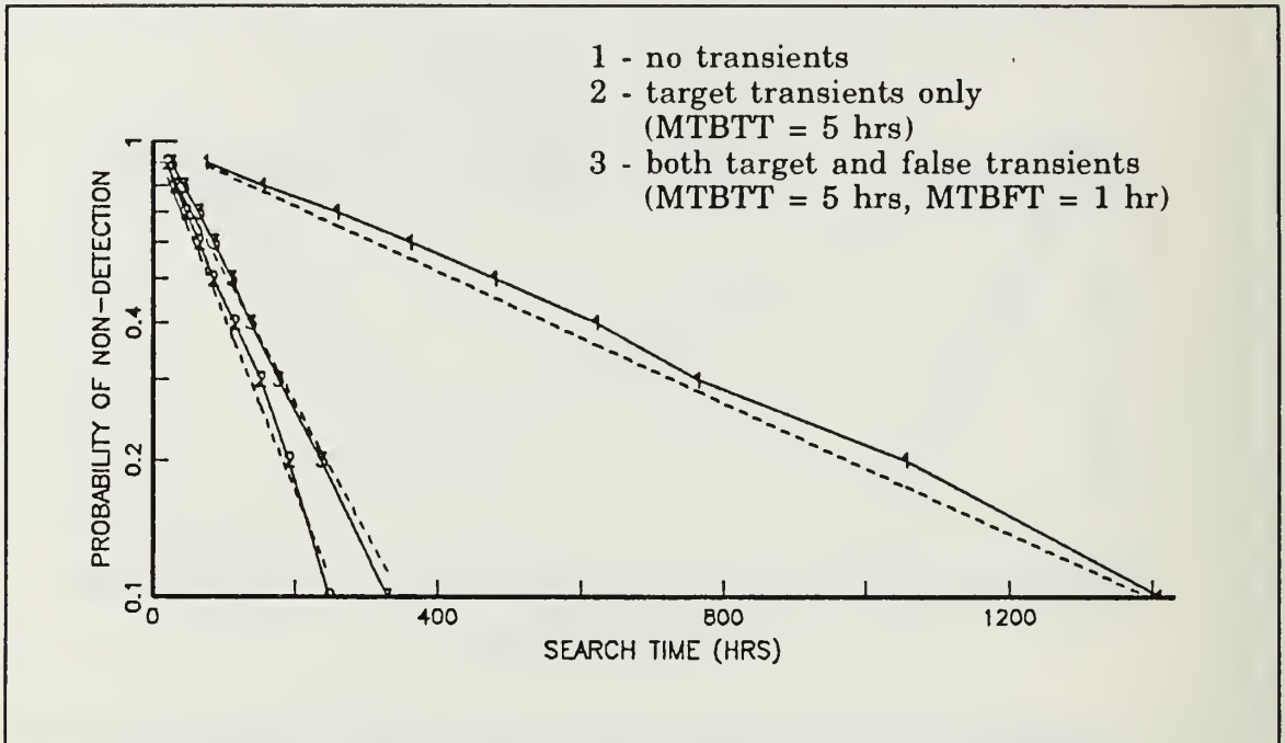
Figure 5.13. Test Case 5 - Probability of Non-Detection.
