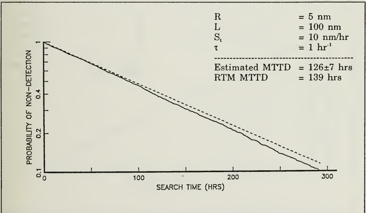
Figure 4.6. Random Tour Model Approximation Case 2 - Probability of Non-Detection.
