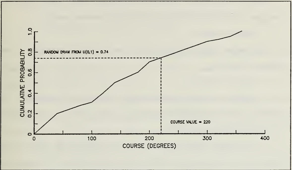
Figure 2.2 Inverse Probability Integral Transformation Method.
