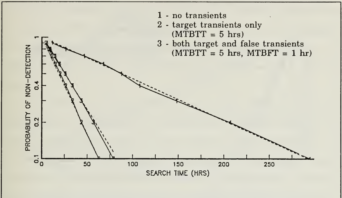
Figure 5.11. Test Case 3 - Probability of Non-Detection.
