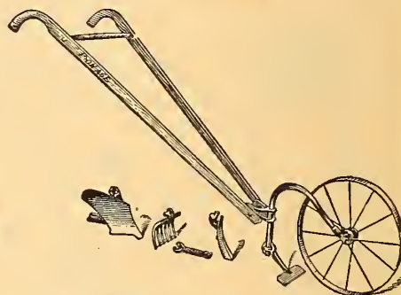
"Iron Age" No. 12 Wheel Plow and Cultivator
