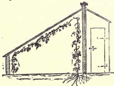
Fig. 301.— Lean-to Grapery.
