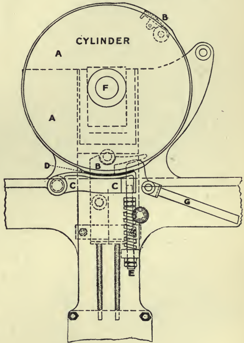
Fig. 17. FURNIVAL BRAKE.
