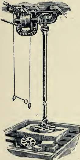
Fig. 2. OVER-HEAD STONE GRINDING MACHINE.
