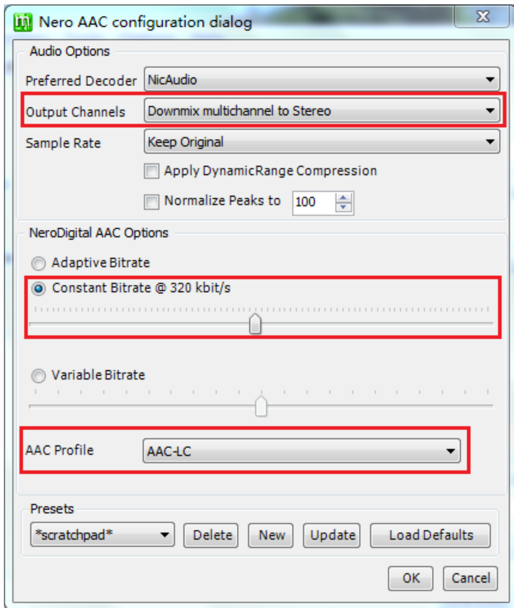
Figure 1 The items needed attention are in red boxes.
