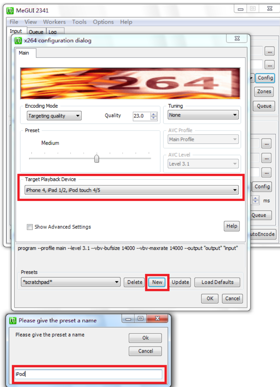
Figure 2 Setting up presets.
