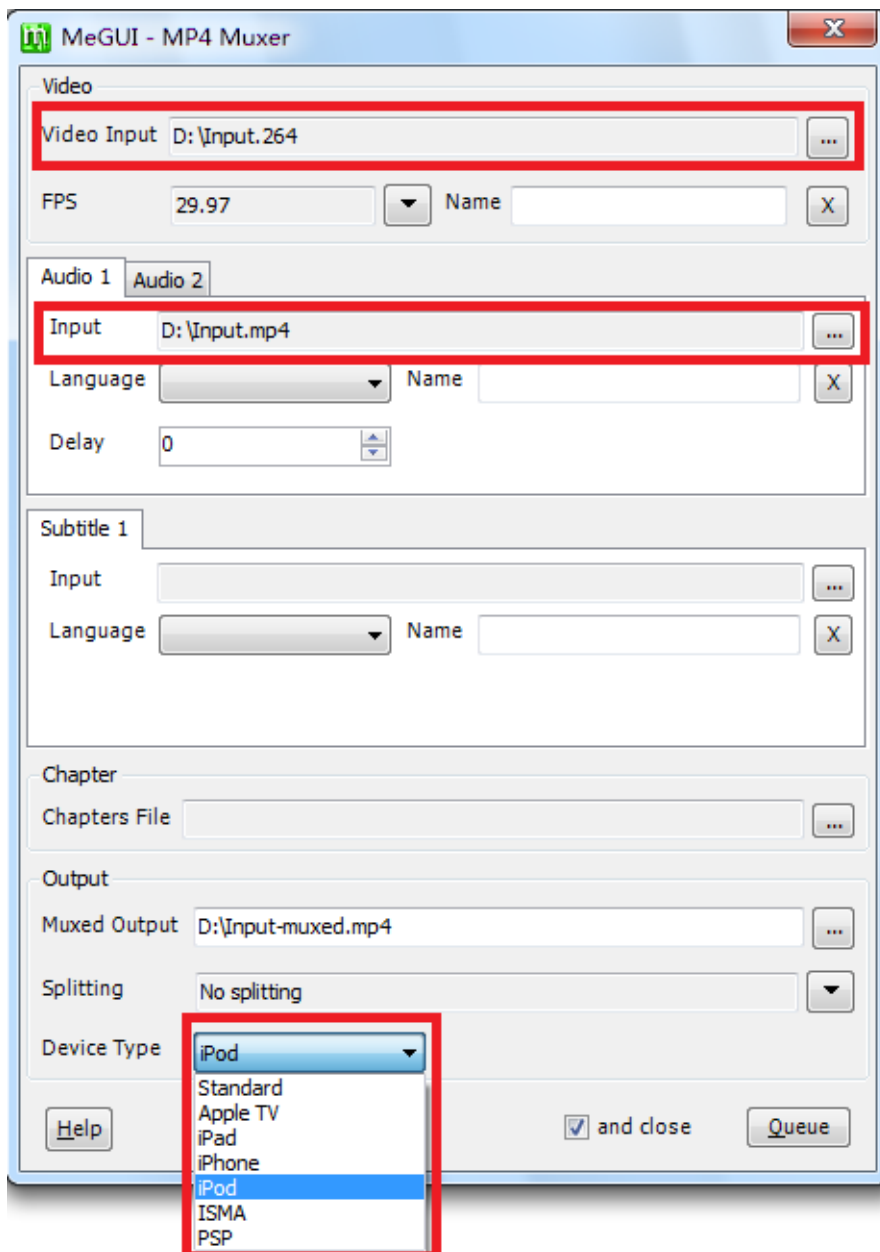
Figure 4 The options that should be changed are in red boxes.
