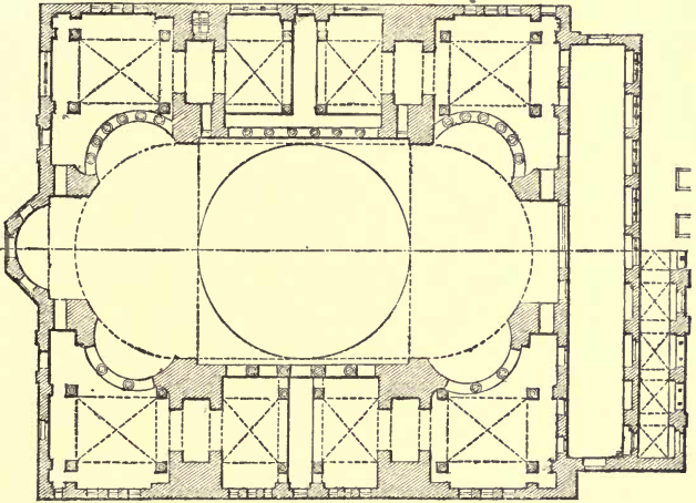
GROUND-PLAN OF THE CHURCH OF ST. SOPHIA
