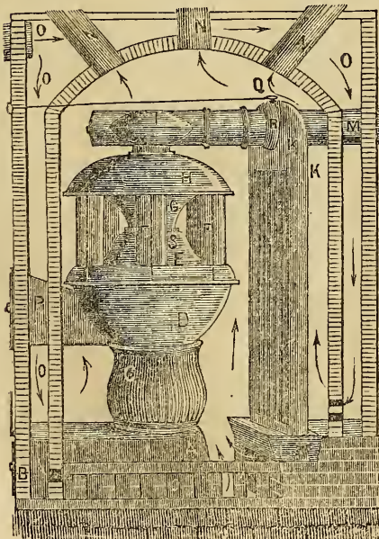
Fig. 3.—CULVER'S FURNACE.
