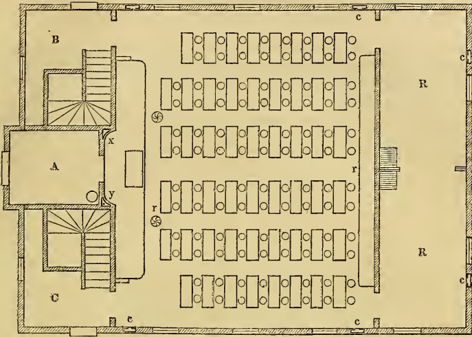
Fig. 3—FIRST FLOOR.
