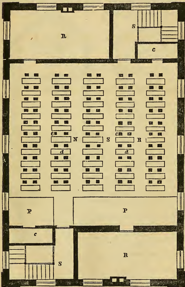
Fig. 6.—UPPER STORY.
