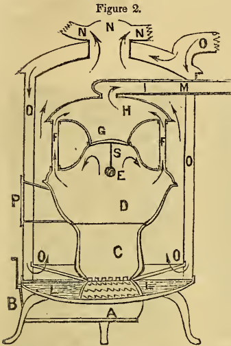
Figure 2 represents a section of large size Portable Furnace or double casings of sheet iron or zinc. The same letters for reference are used as in Fig. 1.
