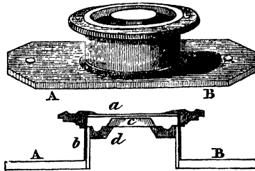
Fig. 57.—Varley's Animalcule-cage.
