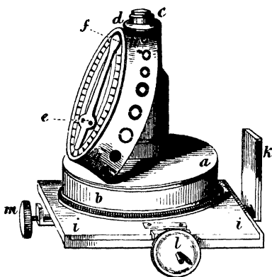
Fig. 42.—Gillett's Condenser.
