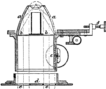
Fig. 44.—Wenham's Parabolic Reflector.
