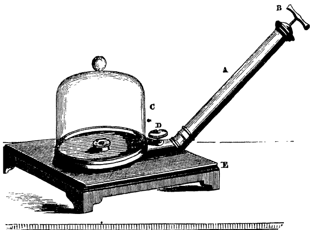
Fig. 74.—Air-Pump.
