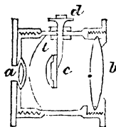
Fig. 2. Lieberkuhn's Microscope.
