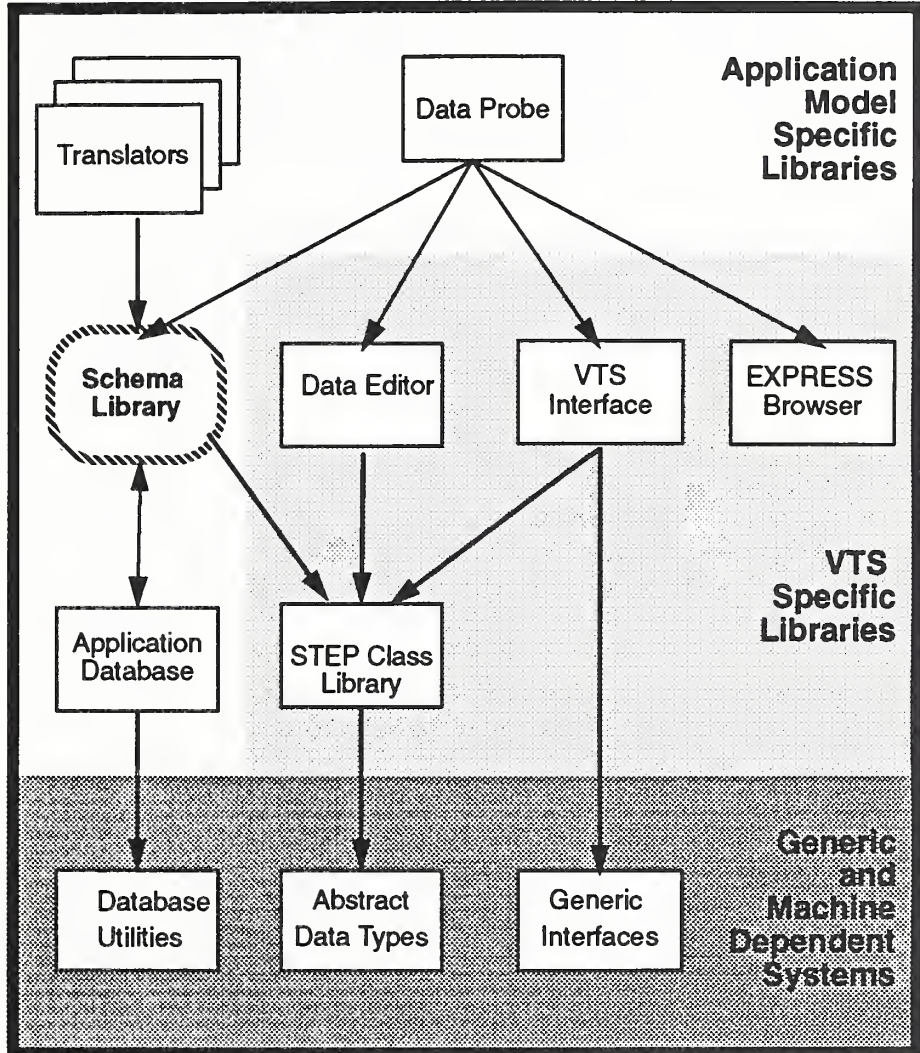
VTS Software Component Relationships
