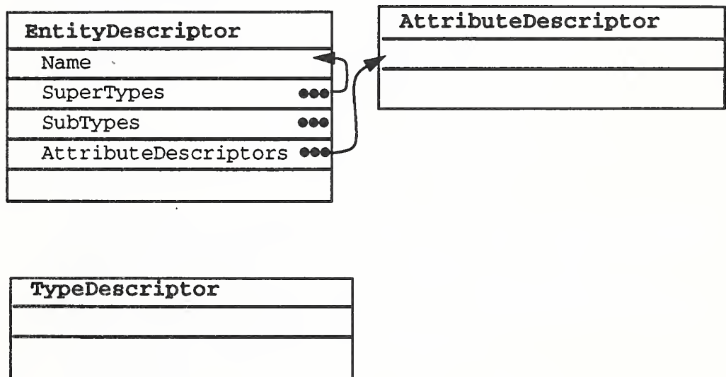
Registry classes
