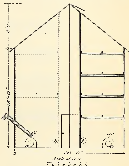
FIG. 9.—End view of a paprika curing house, showing furnaces, smoke pipes, and the arrangement of the interior framework to support the crates.
