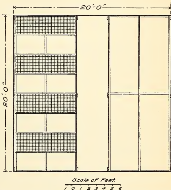
FIG. 11.—Plan of floor of a paprika curing barn, showing on the right side the arrangement of the timber supports and on the left the crates in position.
