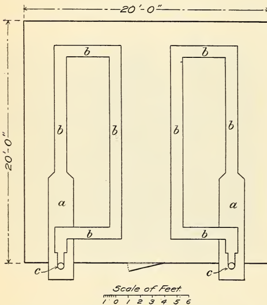
FIG. 10.—Ground-floor plan of a paprika curing barn.
