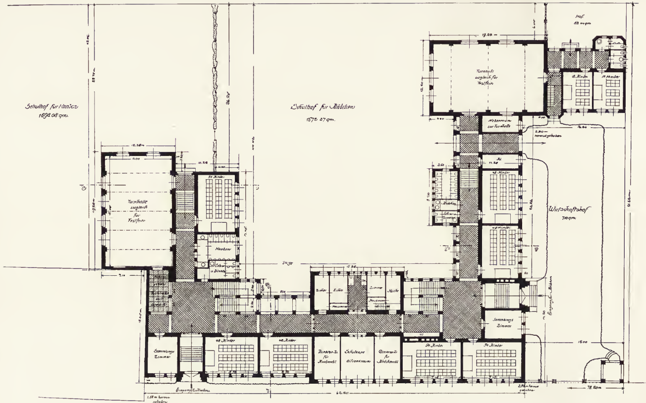
Erdgeschoss.
