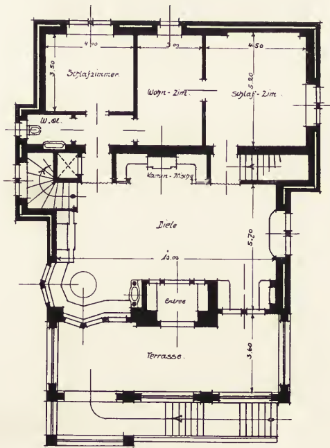
o GRUNDRISS = ERDGESCHOSS o
