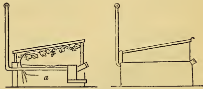
Fig. 8. Section and End Elevation of Mr. White's Vine Pit.
