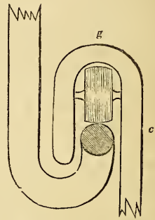
Fig. 29. Section of the horizontal Rod of the Sliding Ladder.
