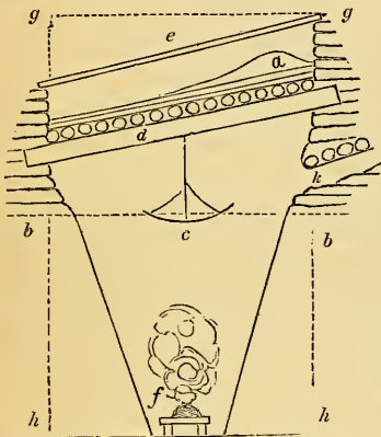
Fig. 52. Section of Hotbed on Forsyth's System.
