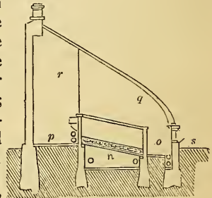
Fig. 14. Cross Section of the House.
