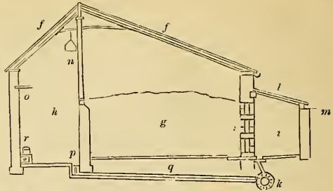
Fig. 19. Cross Section of a Pit to be heated according to Mr. Corbett's System.
