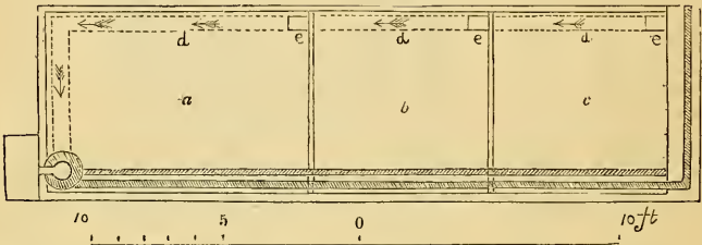
Fig. 10. Ground Plan of Mr. Cunningham's Pits for Grapes, Melons, and Peaches.
