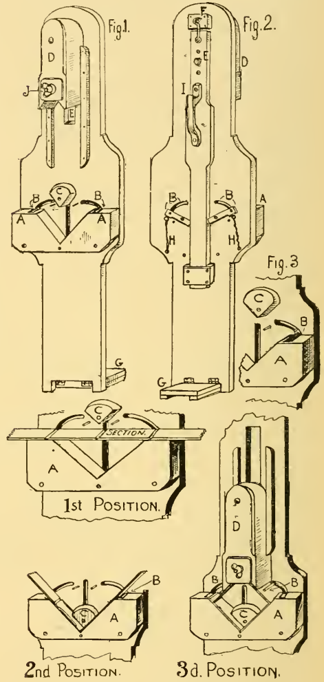
FIG. 1.—FRONT VIEW.
