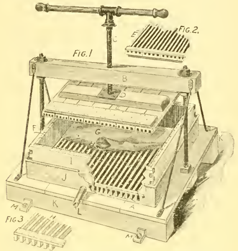
FIG. 1.—HATCH-GEMMILL WAX-PRESS.
