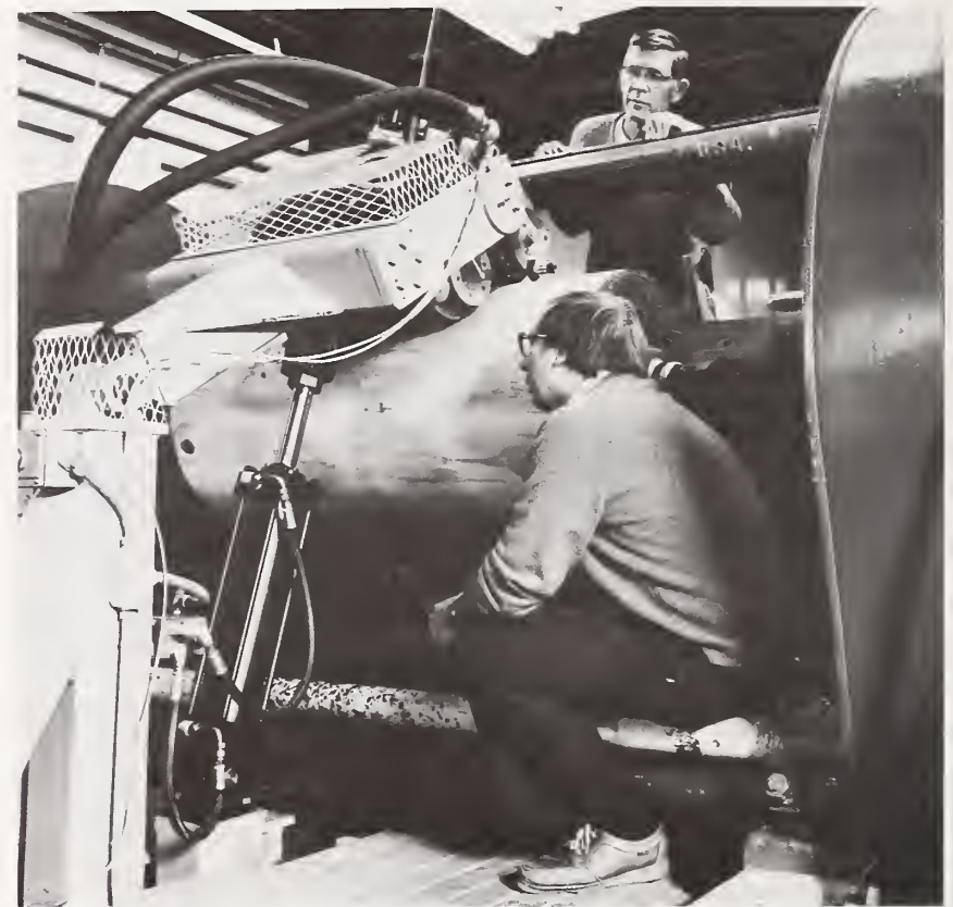
Researchers check alignment of powered backup roll equipment before making a trial veneer peeling.
