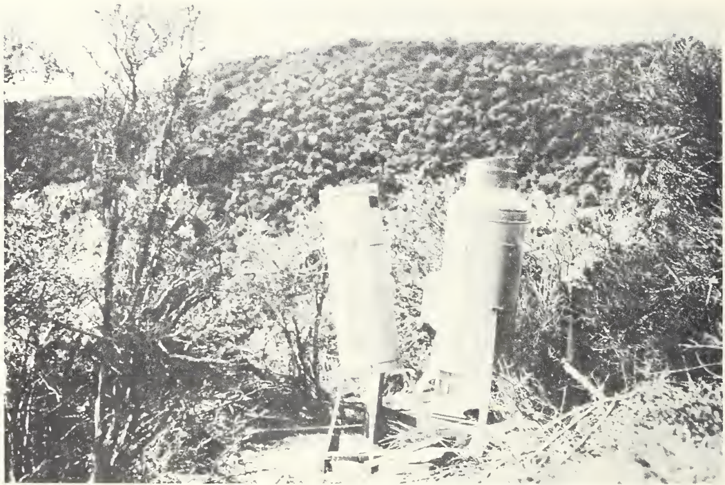
Figure 2.--More accurate measurements of rainfall result when storage gages are tilted (left) and recording gages are fitted with "stereo" funnels (right).
