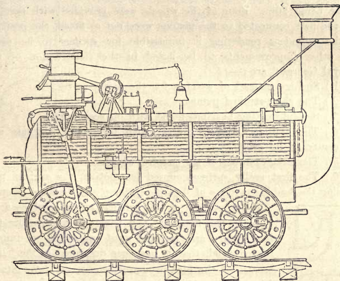
FIG. 12.—THE FIRST SUCCESSFUL LOCOMOTIVE, HACKWORTH'S "ROYAL GEORGE," STOCKTON AND DARLINGTON RAILWAY, 1827
