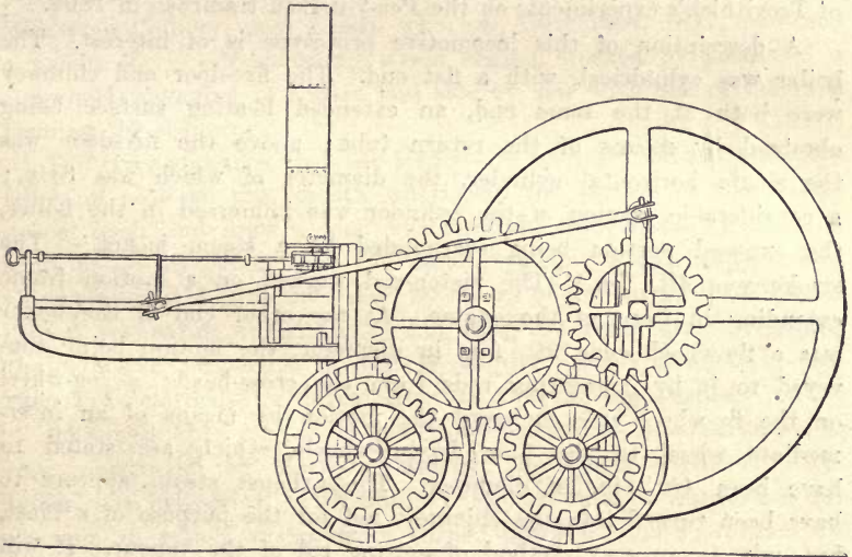
FIG. 1.—THE FIRST RAILWAY LOCOMOTIVE OF WHICH AUTHENTIC PARTICULARS ARE KNOWN
