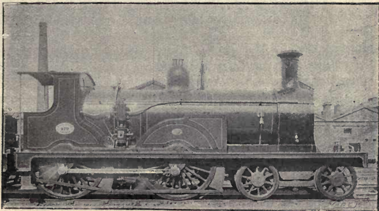
FIG. 116.—FOUR-COUPLED PASSENGER ENGINE WITH LEADING BOGIE, N.B.R.
