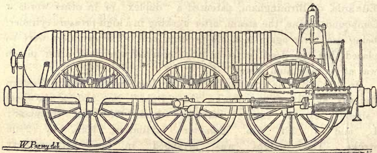
FIG. 65.—PÁSEY'S COMPRESSED AIR LOCOMOTIVE, TRIED ON THE EASTERN COUNTIES RAILWAY IN 1852
