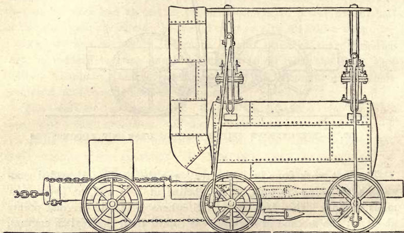
FIG. 7.—STEPHENSON AND DODD'S PATENT ENGINE, BUILT IN 1815
