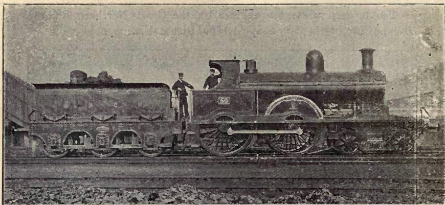
FIG. 143.—“JUBILEE,” 4-WHEELS COUPLED COMPOUND LOCOMOTIVE, BELFAST AND NORTHERN COUNTIES RAILWAY
