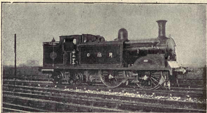
FIG 125.—MCINTOSH'S 5FT. 9IN. CONDENSING TANK ENGINE, CALEDONIAN RAILWAY
