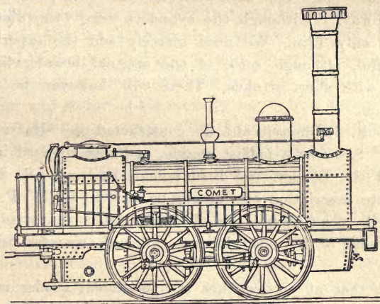
FIG. 25.—HAWTHORN'S "COMET," THE FIRST ENGINE OF THE NEWCASTLE AND CARLISLE RAILWAY, 1835
