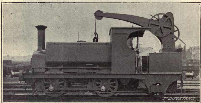
FIG. 89.—LOCOMOTIVE AND TRAVELLING CRANE, N.L.R.
