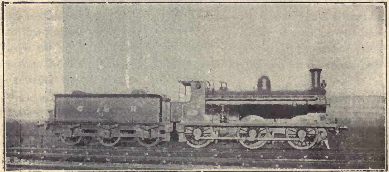
FIG. 123.—SIX-WHEELS-COUPLED CONDENSING ENGINE, CALEDONIAN RAILWAY
