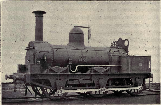
FIG. 81.—SIX-COUPLED MINERAL ENGINE, TAFF VALE RWY., BUILT 1860
