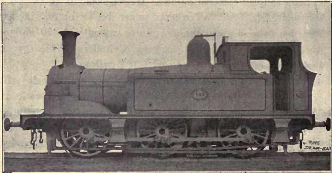
FIG. 126.--"No. 143," TAFF VALE RAILWAY INCLINE TANK LOCOMOTIVE
