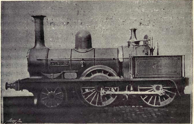
FIG. 84.—“ALBION,” CAMBRIAN RAILWAYS, 1863
