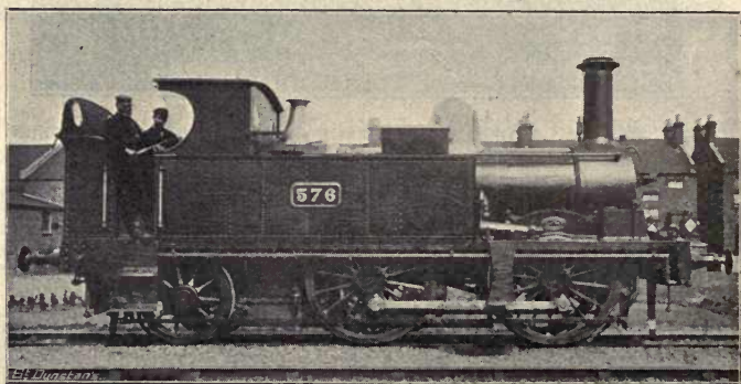
FIG. 135.—4-COUPLED-IN-FRONT PASSENGER TANK ENGINE, G.W.R.
