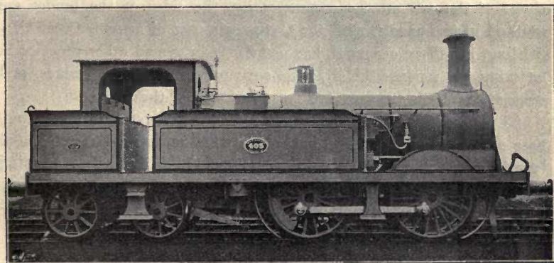
FIG. 111.—STANDARD PASSENGER TANK LOCOMOTIVE, S.E. R.WY.
