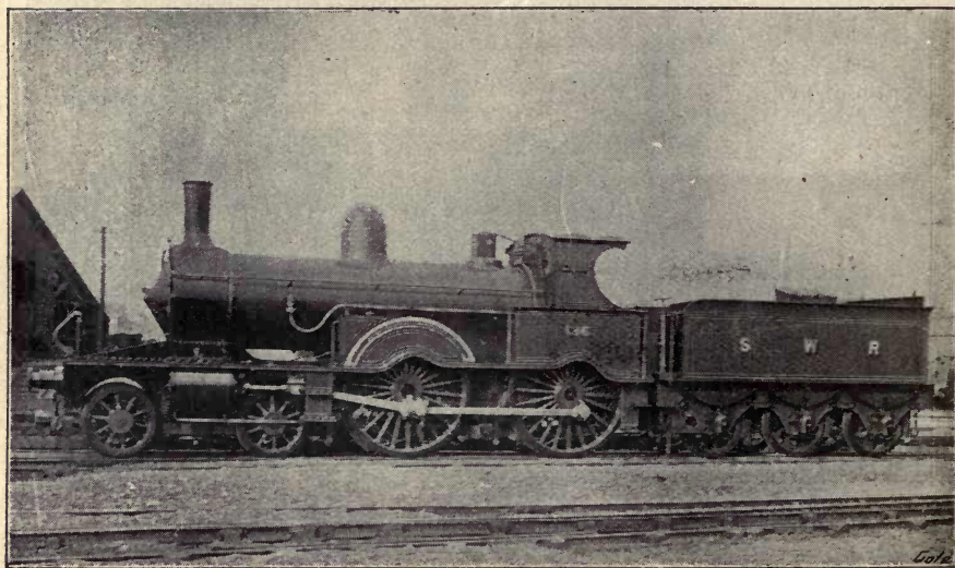
FIG. 114.—A "WINDCUTTER" LOCOMOTIVE ENGINE, "No. 136," L. & S.W.R., FITTED WITH A CONVEX SMOKE-BOX DOOR
