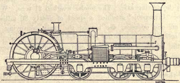
FIG. 55.—CRAMPTON'S "LIVERPOOL," L. AND N.W.R.
