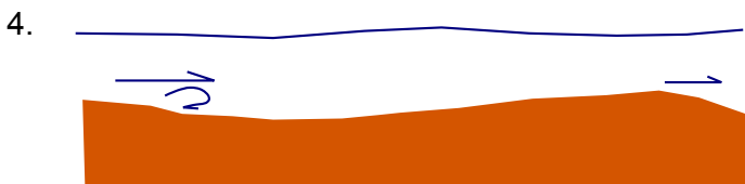
Washed out dunes
