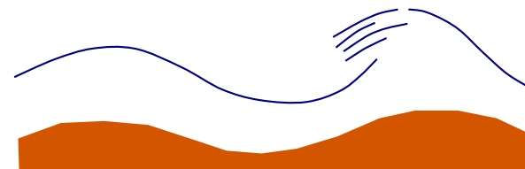
Antidune breaking wave
