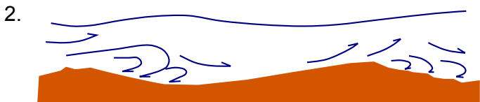
Dunes with ripples superposed
