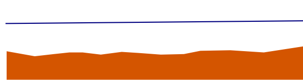
Plane bed
