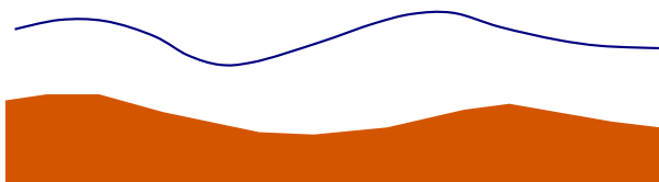
Antidune standing wave
