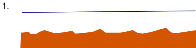
Typical ripple pattern
