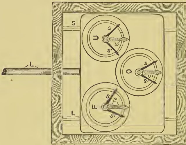
FIG. 17.—Plan. U, upwards; F, forwards; O, outwards.
