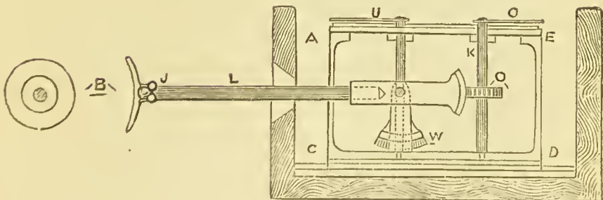
FIG. 16.—Sectional side elevation.
