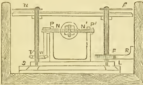
FIG. 14.—Sectional end elevation.
